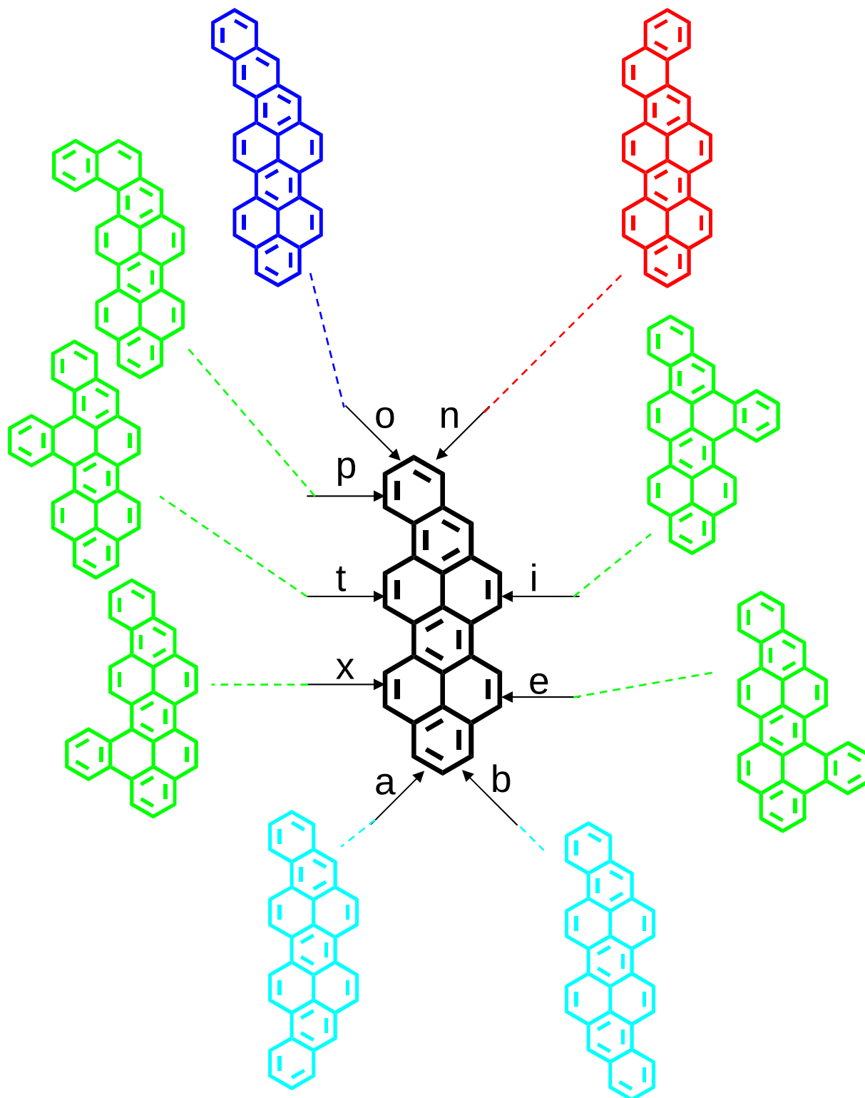
Figure 10. Benzo[cd]naphtho[1,2,3- lm ]perylene and the 9 possible benzenoid C_{34}H_{18} that can result from ring fusion to benzo[cd]naphtho[1,2,3- lm ]perylene. Benzo[cd]phenanthro[1,2,3- lm ]perylene, shown in red, is deduced to be the 1-methylnaphthalene product component eluting at 174 min in Figure 7.
