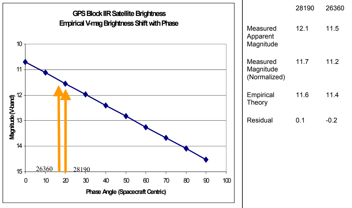
Figure 16. GPS IIR empirical satellite brightness versus phase angle. Both measurements from MOST are consistent with the plot.
