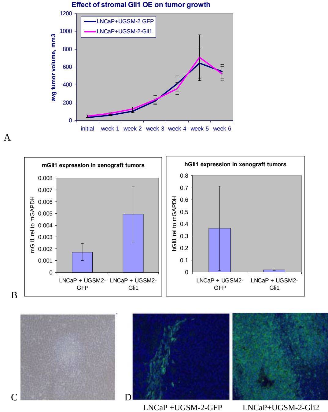
Figure 4. Effect of stromal Gli over-expressing on tumor growth. The growth of LNCaP + UGSM-2-Gli1 tumor didn't show any difference compared to control (Figure3A), P > 0.05 . Neither hGli1 or mGli1 was over-expressed in the xenograft tumors (Figure 3B), P > 0.05 . For each group, data were analyzed from the real time PCR results from three different tumors. (C) Over-expression of Gli2 caused cell transformation. (D) Immunohistochemical staining for GFP positive UGSM-2 cells in the xenograft tumor. Left is control tumor (LNCaP+UGSM-2 GFP), Right is UGSM-2 over-expressing Gli2 cells co-injected with LNCaP. Compared to control, LNCaP+ UGSM-2-Gli2 tumors are mainly composed of UGSM-2 cells (green cells), indicating the tumors are sarcomas. Blue is for DAPI, Green is for GFP.
