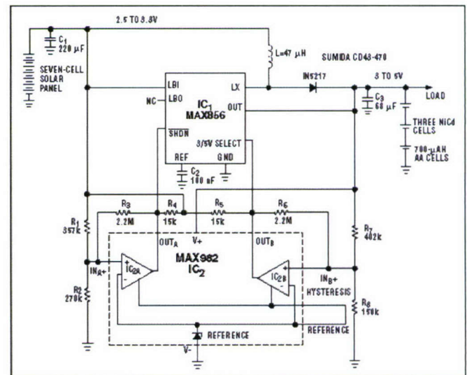
Figure 6. Maxim PPT and BCR Circuit
