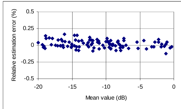
Figure 2: The relative error of 100 mean estimates.
