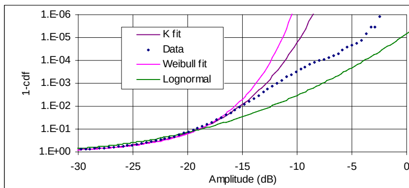
(c) 1-cdf abscissa on log scale to view cdf convergence
