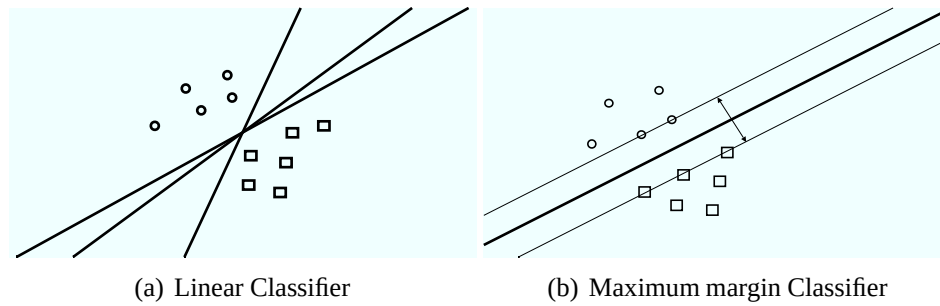
Figure 4.1. Linear classifiers.
