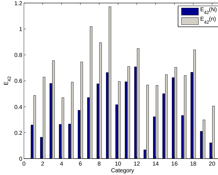
(b) 20 Newsgroups
