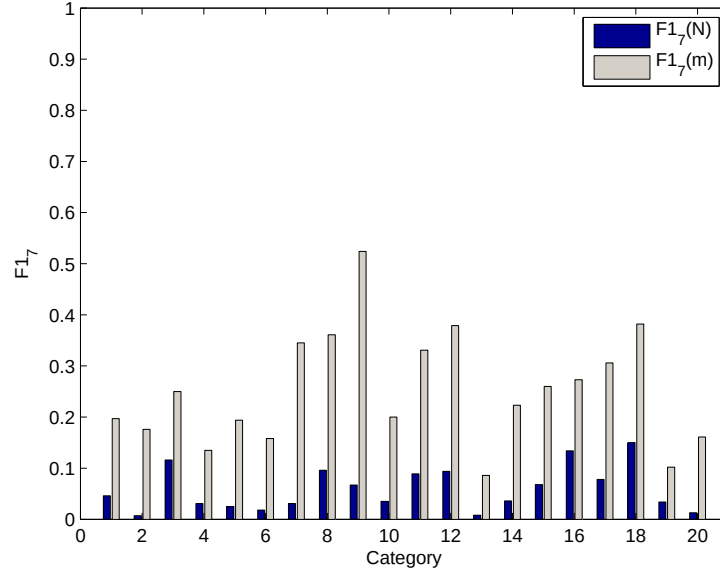
(b) 20 Newsgroups
