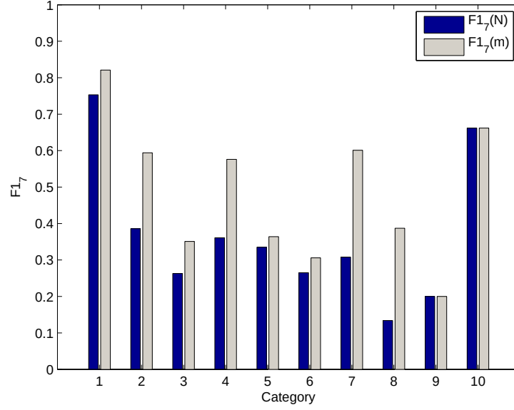
(a) Reuters
