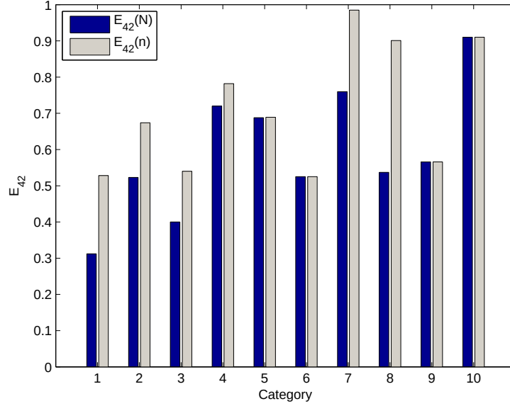
(a) Reuters
