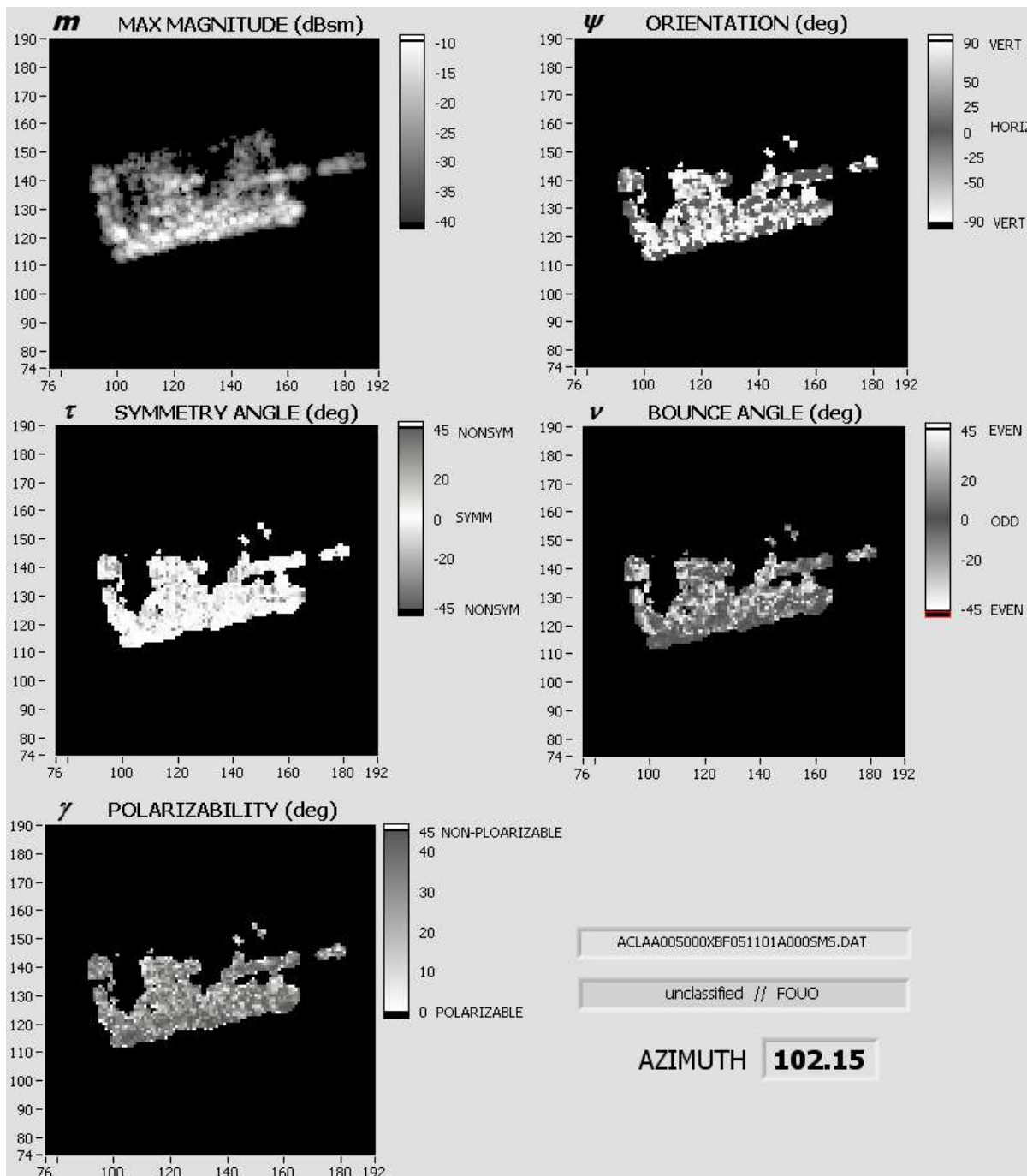
Figure 1. ISAR Images in Optimized Euler Parameter Space of the T-72BK Tank Fingerprint
