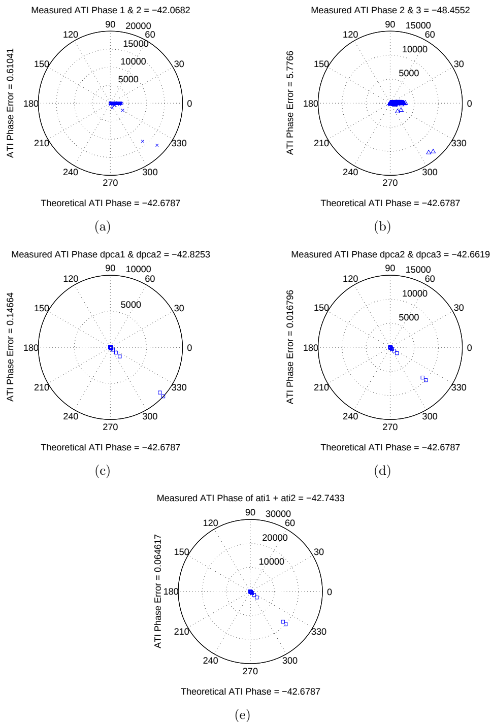
Figure 15: The same mode as Fig. 15. Polar plots of the phase and amplitude of the interferogram between (a) channels 1 and 2, (b) channels 2 and 3, (c) DPCA of channels 1 and 2 and DPCA of channels 2 and 3, (d) DPCA of channels 2 and 3 and DPCA of channels 3 and 4, and (e) by adding (c) and (d).
