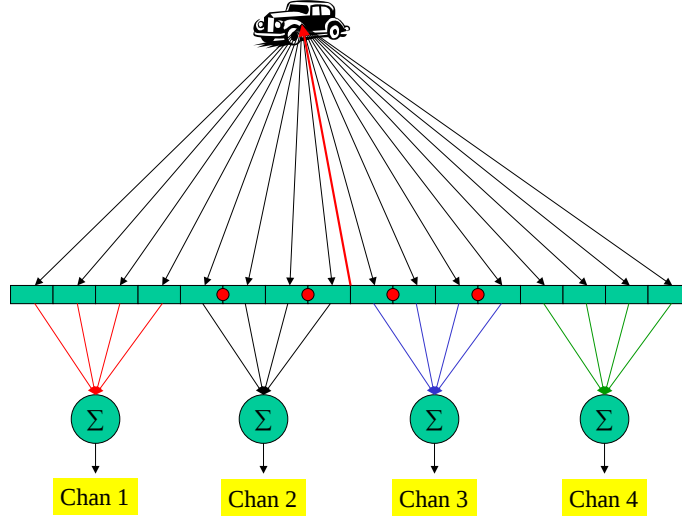
Figure 6: Schematic showing the simulation of a multi-aperture antenna: the radar signal is transmitted using the full aperture and returns are received using 16 sub-panels. The return signals received at the 16 sub-panels are added in such a way as to form four phase centres.
