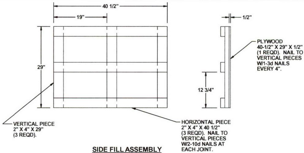
SIDE FILL ASSEMBLY (2 REQD)
