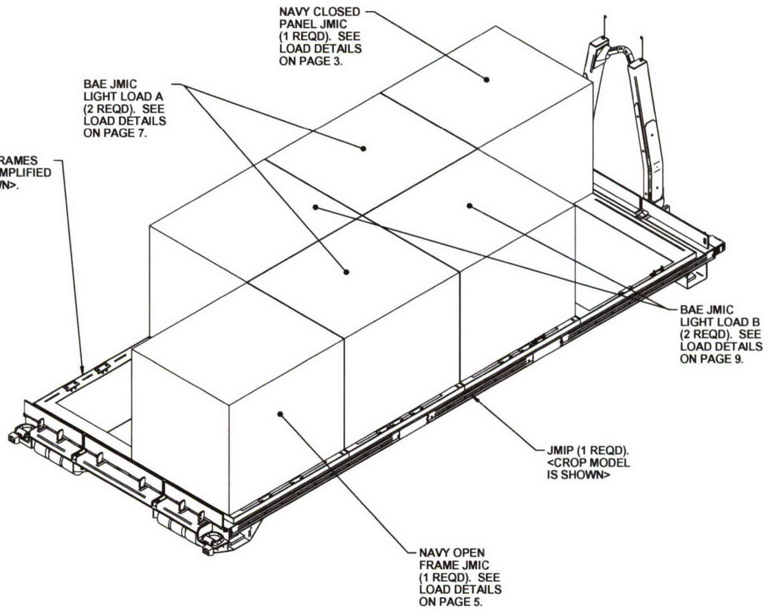
ISOMETRIC VIEW
