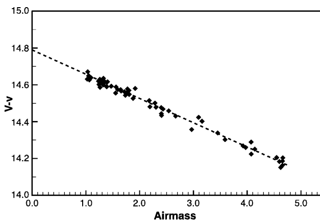
FIG. 13.—Example “extinction plot” showing offset of measured magnitudes from standard system as a function of air mass after the color transformation term is applied.
