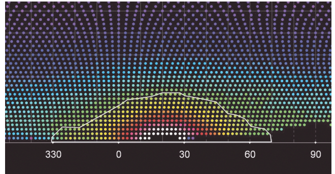
FIG. 5.—Light dome of Las Vegas, Nevada, as seen from Mojave National Preserve, and its boundary (white outline) defined as described in the text. The numbers shown at the bottom represent the azimuth in degrees. The color of each sample point represents sky brightness, following the legend in Figs. 7–9.
