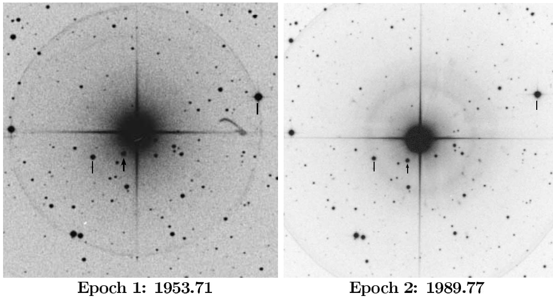
FIG. 2.—DSS images from two epochs for HD 9826. The 10' square images have north up and east to the left. WDS lists components B and C (marked by lines), which are background stars. WDS component D (marked by an arrow), however, is a CPM companion. The primary's \mu = 0''.42 \text{ yr}^{-1} at 204^\circ .
