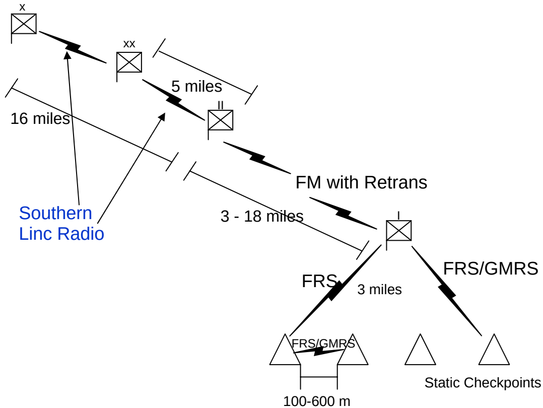
Figure 3. Voice Network from Checkpoint to Division Headquarters
