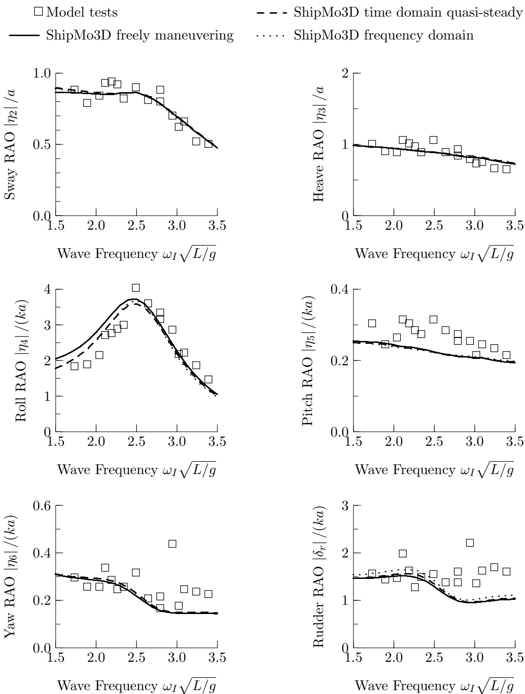
Figure 24: RAOs for Steered Warship, Stern Quartering Seas at 75 degrees, Froude Number 0.18
