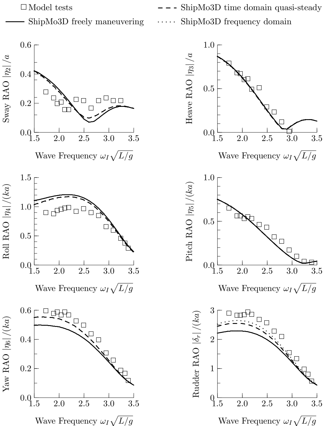
Figure 18: RAOs for Steered Warship, Stern Quartering Seas at 30 degrees, Froude Number 0.18
