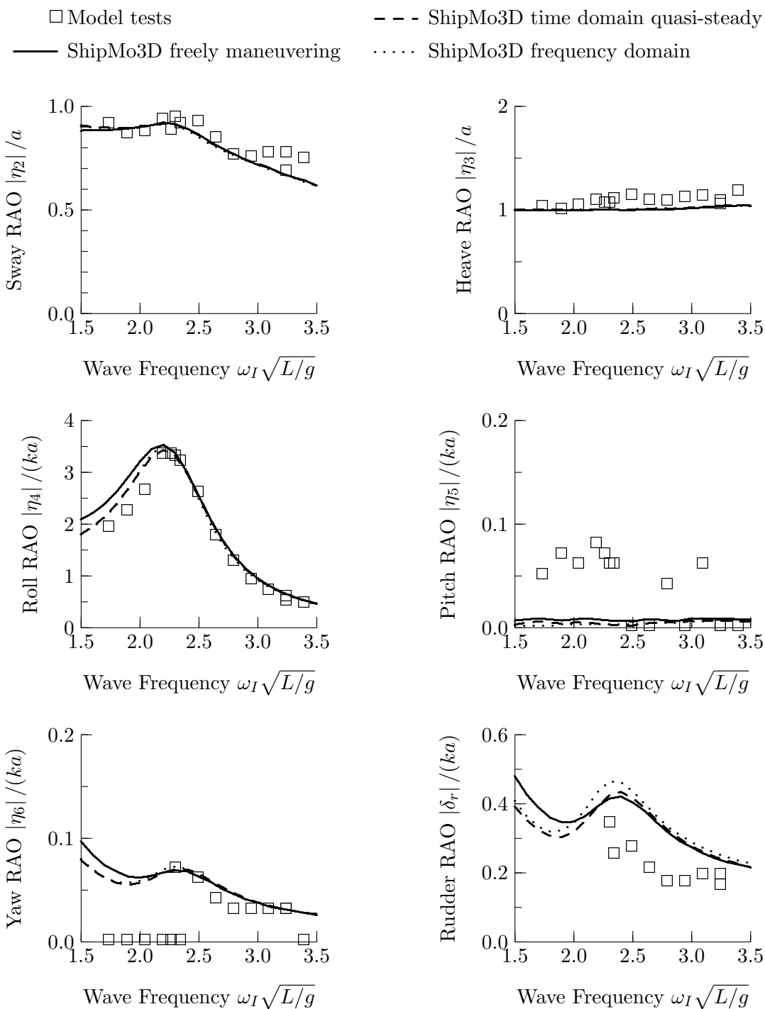
Figure 27: RAOs for Steered Warship, Stern Quartering Seas at 90 degrees, Froude Number 0.18
