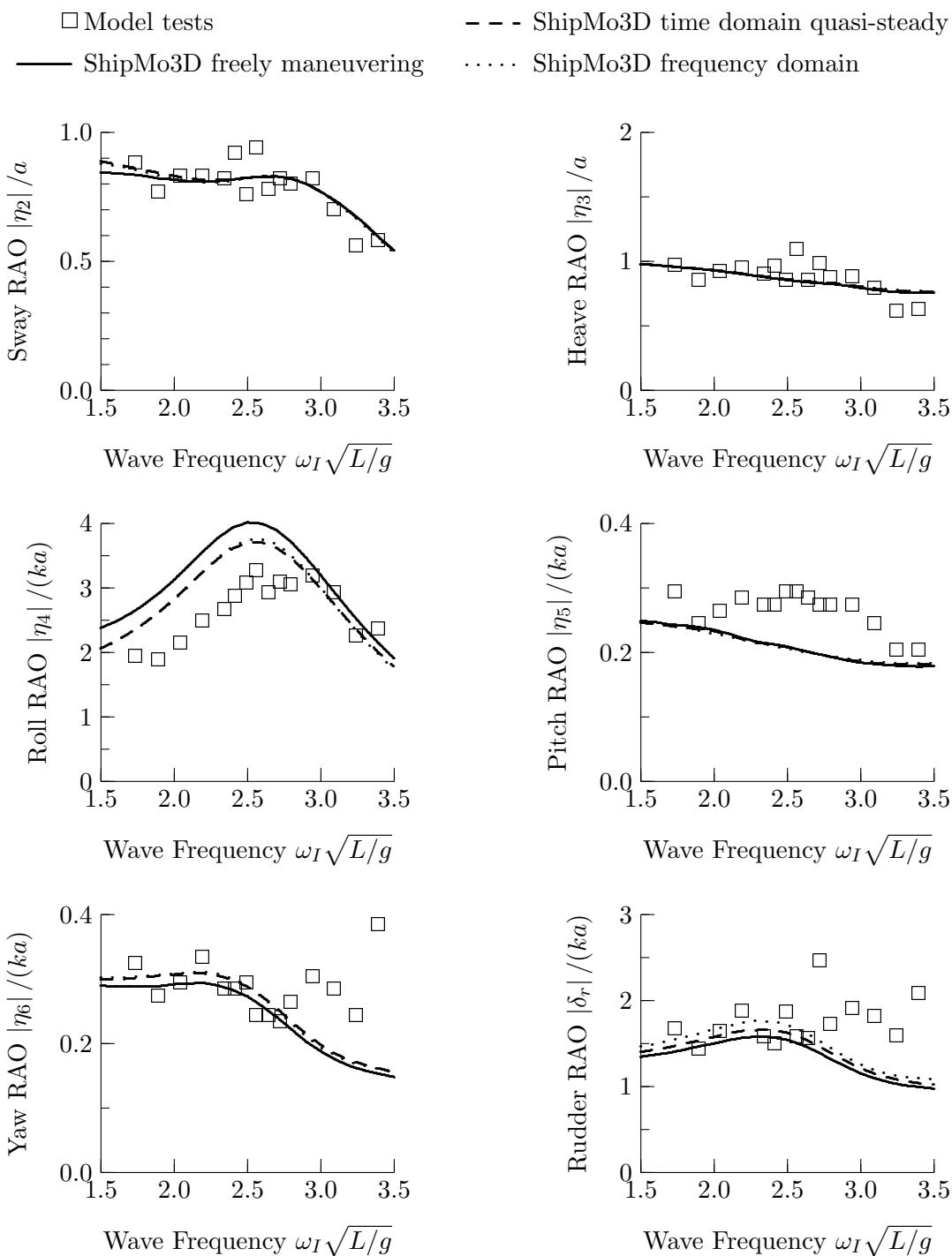
Figure 25: RAOs for Steered Warship, Stern Quartering Seas at 75 degrees, Froude Number 0.28
