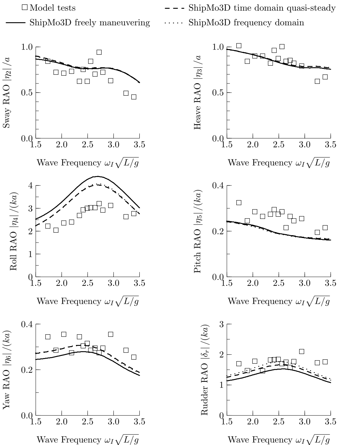
Figure 26: RAOs for Steered Warship, Stern Quartering Seas at 75 degrees, Froude Number 0.36
