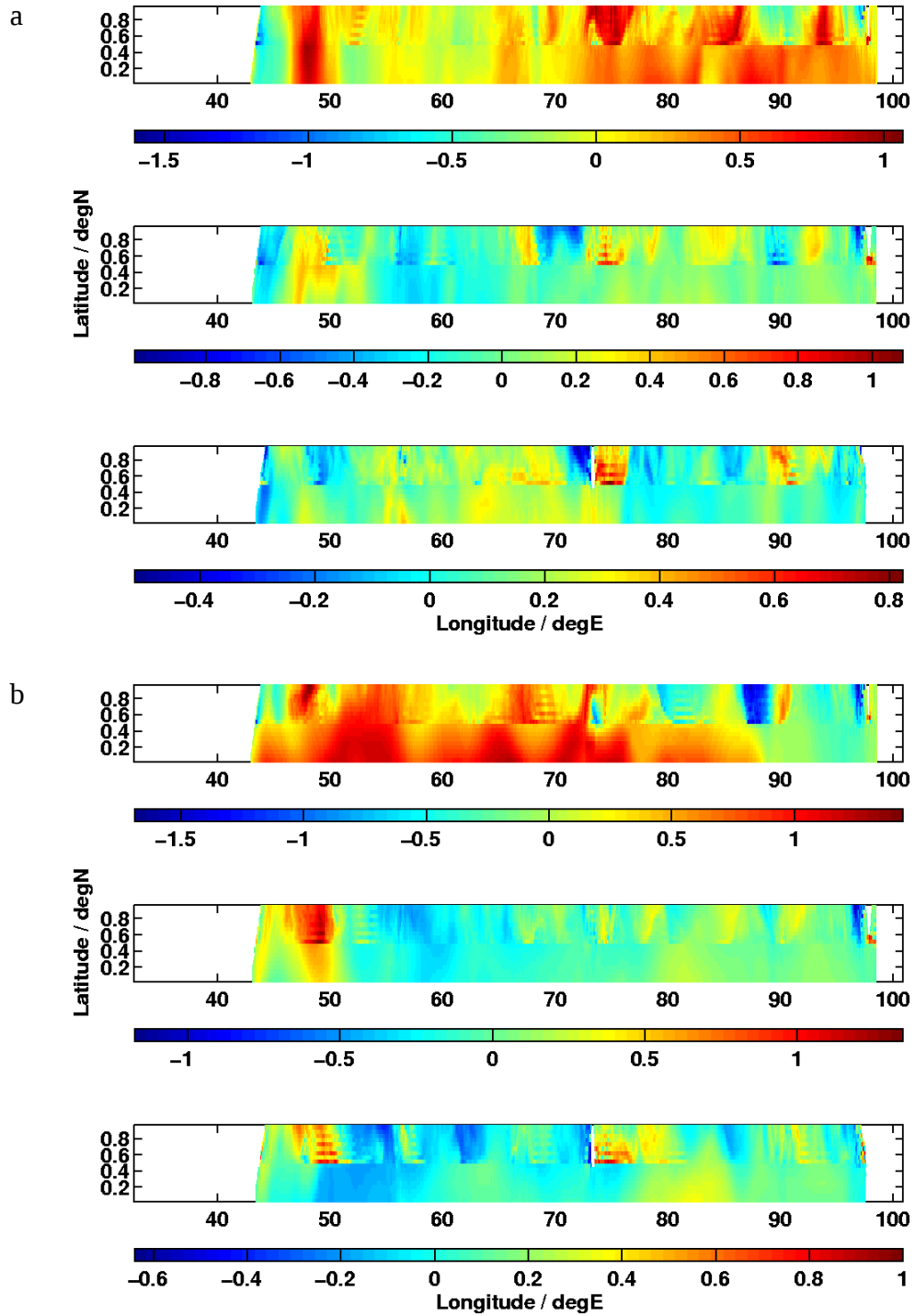
Fig. 119 – Zonal velocity (m/s) along the southern boundary of the SWAFS ionest domain restart files valid 07 Dec 2003 using the northworld (a) and NCOM/OSU (b) boundary conditions, each at 0 (top), 200 (middle), 1000 (bottom) m.
