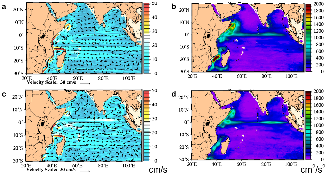
Fig. 34 – Indian Ocean zoom of mean 1998-2000 100m speed with superimposed currents (left; a, c) and 100m EKE (right; b, d) for free-running (top; a, b) and assimilative (bottom; c, d) 1/8° global NCOM.
