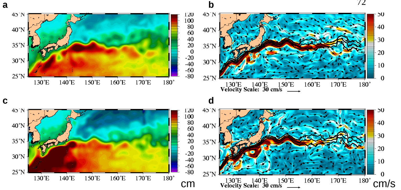
Fig. 31 – Kuroshio zoom of mean SSH (left;a,c) and surface speed with superimposed currents (right;b,d) for assimilative 1/8° global NCOM (top;a,b) and assimilative 1/4° SWAFS Northworld (bottom;c,d). Superimposed black curves are the mean and mean \pm 1 standard deviation fronts from the NAVOCEANO Kuroshio north wall bogues from archives over the same time period. Mean is over period of available SWAFS surface data, 9/1/2002 – 5/31/2003. To enable the same color bar and ranges to be used, the mean SWAFS SSH is offset to equal the mean NCOM SSH over this domain. NCOM has a more realistic eastward extension of the Kuroshio.
