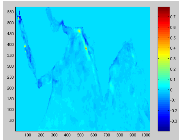
Fig. 113 – The heat flux adjustment parameter for the operational SWAFS ionest run 08 Dec 2003.
