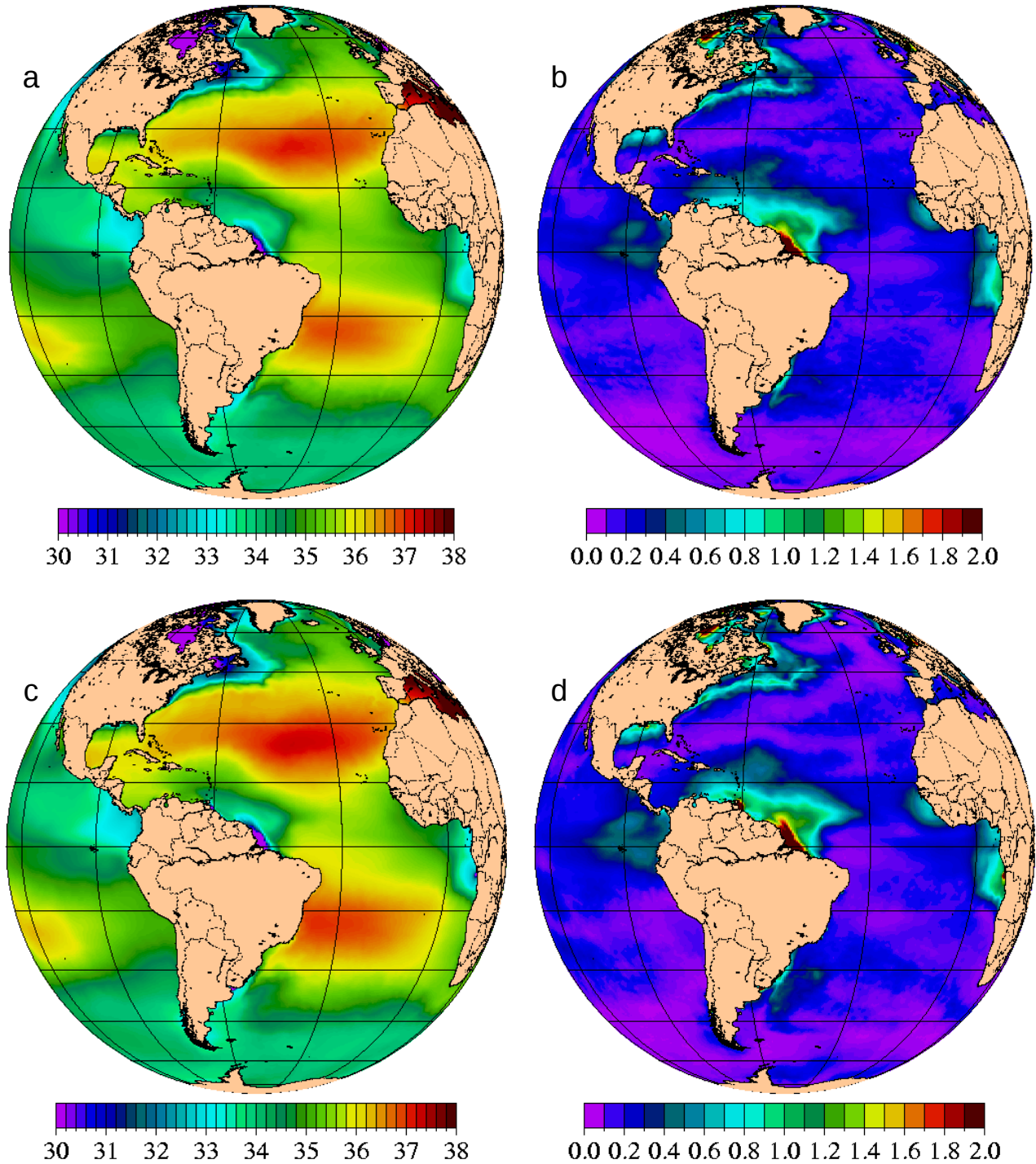
Fig. 7 – Atlantic hemispheric view of mean 1998-2000 SSS (left; a, c) and SSS standard deviation (right; b, d) for free-running (top; a, b) and assimilative (bottom; c, d) 1/8^\circ global NCOM. NCOM is forced with NOGAPS wind and thermal fluxes. The assimilative case relaxes to MODAS synthetic temperature and salinity derived from 1/8^\circ MODAS2D SST and 1/16^\circ NLOM SSH.
