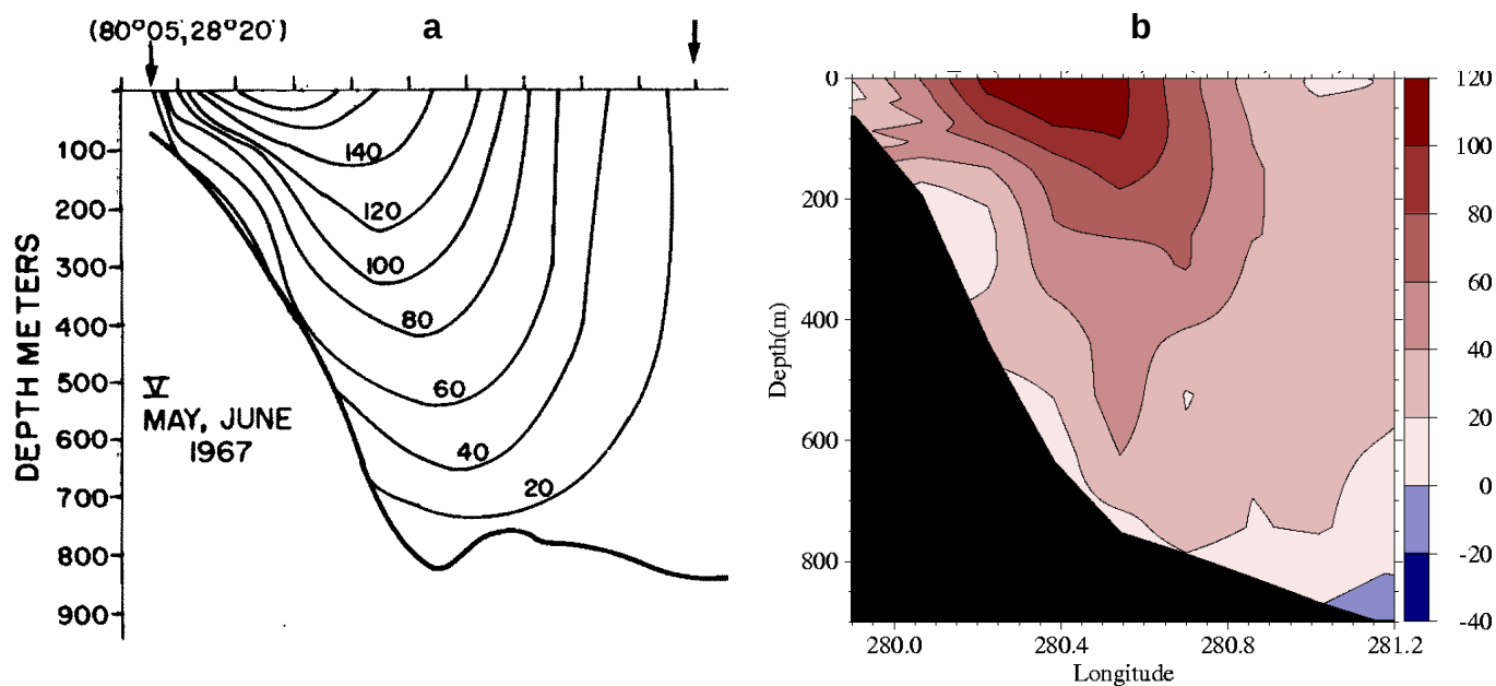
Fig. 68 – Comparison of mean currents through Florida Current section V. (a) downstream speed contours from Schmitz (1996) with observations from May-June 1967 and (b) northward speed contours from assimilative 1/8^{\circ} global NCOM 1998-2000 mean section at 28^{\circ}20'N , 80^{\circ}06'W - 78^{\circ}48'W .
