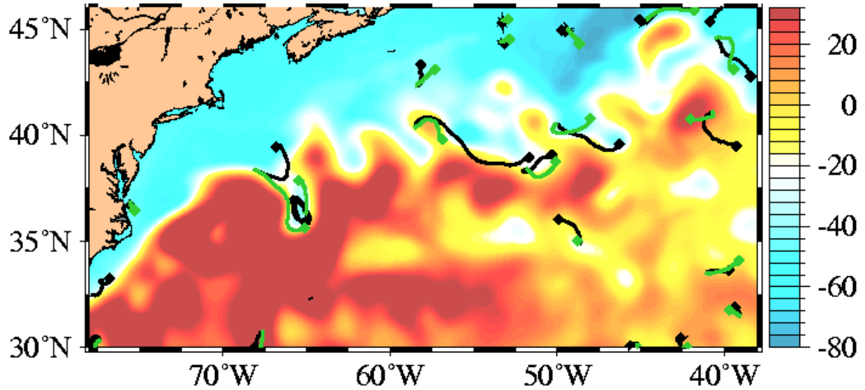
Fig. 59 – Comparison between observed WOCE drifter trajectories (black) and trajectories simulated using data-assimilative 1/8^\circ global NCOM (green). The trajectories start at the same location and time, 31 July 2002. All trajectories are seven days long. The trajectories are superimposed on NCOM SSH for the start date.
