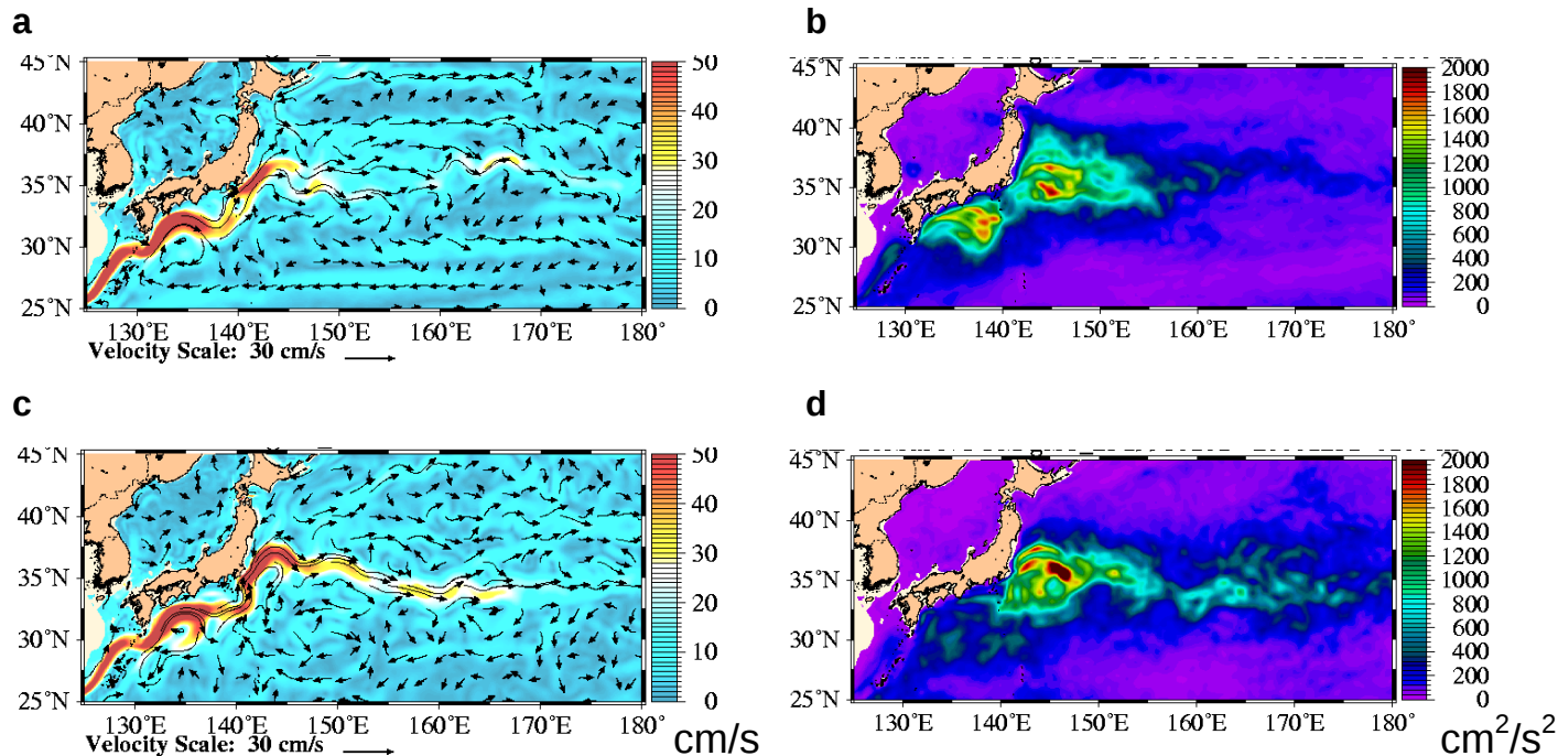
Fig. 28 – Kuroshio zoom of mean 1998-2000 surface speed with superimposed currents (left;a,c) and surface EKE (right;b,d) for free-running (top;a,b) and assimilative (bottom;c,d) 1/8^\circ global NCOM. Superimposed black curves are the mean and mean \pm 1 standard deviation fronts from the NAVOCEANO Kuroshio north wall bogues from archives over the same time period.
