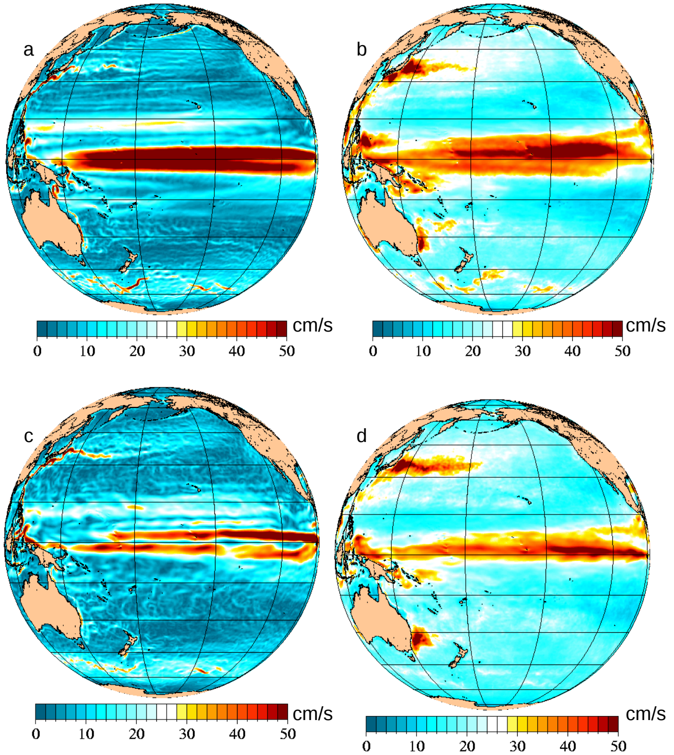
Fig. 18 – Pacific hemispheric view of mean 1998-2000 surface speed (left; a,c) and surface speed standard deviation (right; b,d) for free-running (top; a,b) and assimilative (bottom; c,d) 1/8^\circ global NCOM. NCOM is forced with NOGAPS wind and thermal forcing. The assimilative case relaxes to MODAS synthetic temperature and salinity derived from 1/8^\circ MODAS2D SST and 1/16^\circ NLOM SSH.
