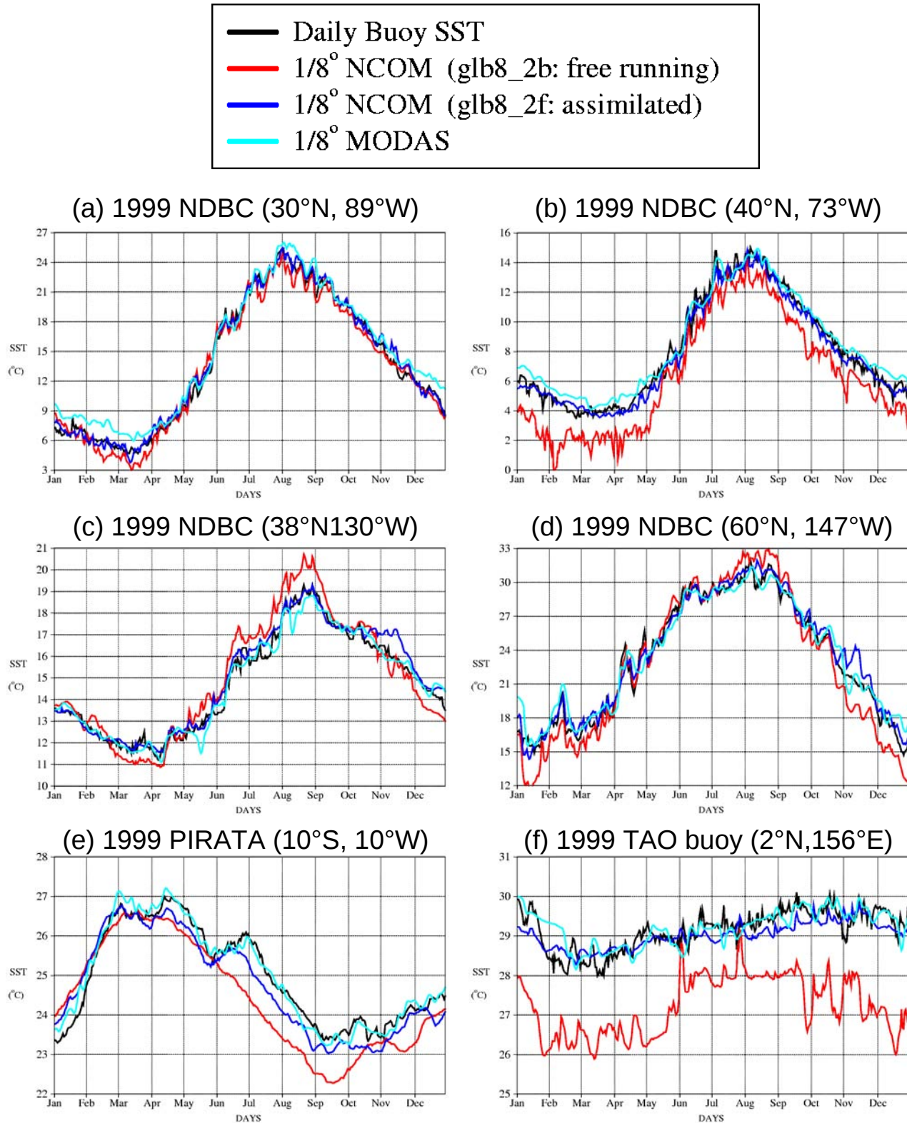
Fig. 49 – Comparison between observed (black), free-running NCOM (red), assimilative NCOM (blue) and MODAS analyses (SST) at a sample of observing buoy stations for 1999. (a) NDBC buoy along the U.S. Gulf coast (30°N, 89°W); (b) NDBC buoy along the U.S. east coast (40°N, 73°W); (c) NDBC buoy along the U.S. west Coast (38°N, 130°W); (d) NDBC off the coast of Alaska (60°N, 147°W); (e) PIRATA buoy in the equatorial Atlantic (10°S, 10°W); (f) TAO buoy in equatorial Pacific warm pool (2°N, 156°E)
