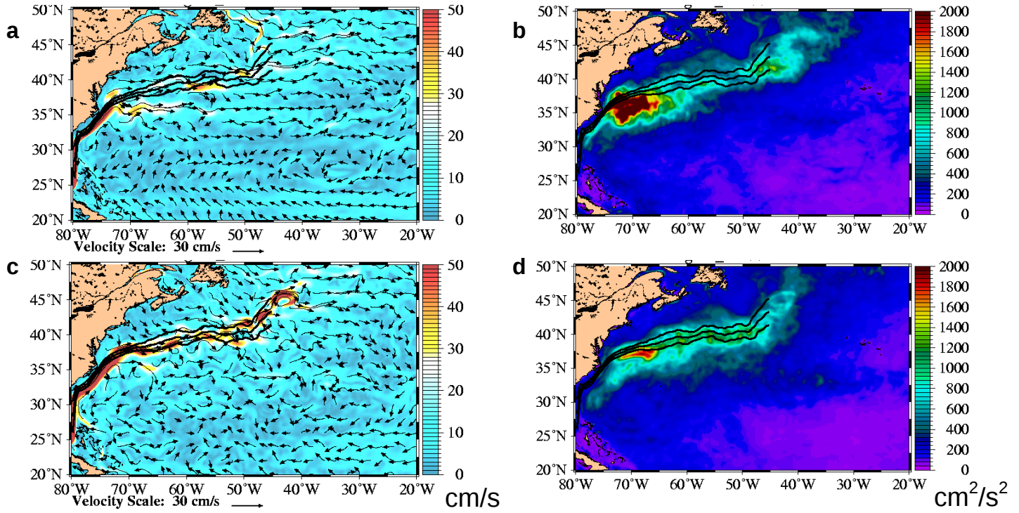
Fig. 20 – Gulf Stream zoom of mean 1998-2000 surface speed with superimposed currents (left;a,c) and surface EKE (right;b,d) for free-running (top;a,b) and assimilative (bottom;c,d) 1/8° global NCOM. Superimposed black curves are the mean and mean \pm 1 standard deviation fronts from the NAVOCEANO Gulf Stream north wall bogues from archives over the same time period.
