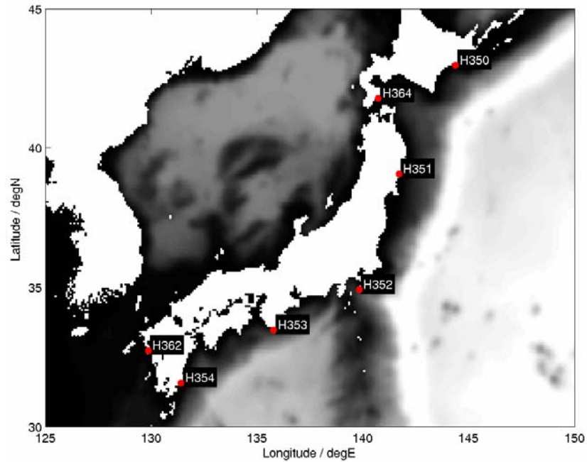
Fig. 110 Locations of the tide gauge stations used for NCOM/OSU validation. The ‘H’ in each id refers to the hourly data contained in the file, and the number is the GLOSS database station identifier.
