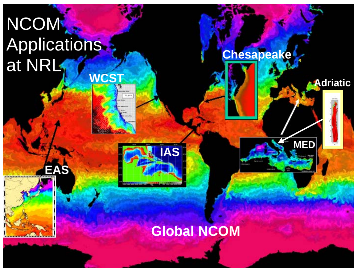
Fig. 122 – An example of some of the applications of NCOM at NRL. The EAS, IAS and WCST domains use boundary and/or initial condition information from global NCOM.
