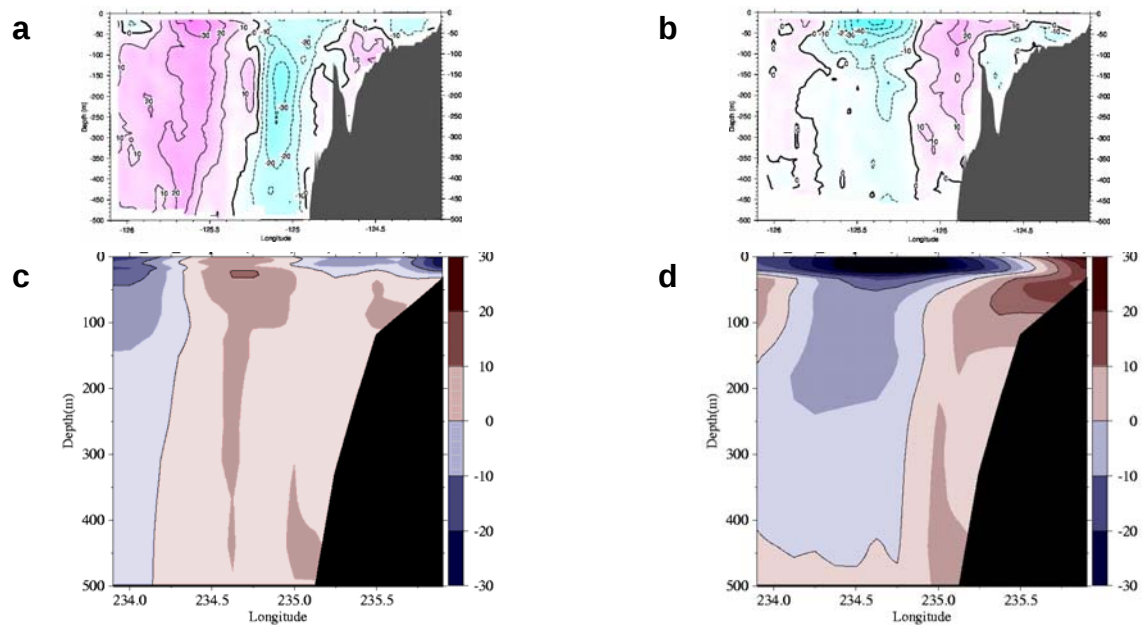
Fig. 90 – Comparison of northward velocity (cm/s) through a section at 44.6°N near Newport, Oregon. Sections from (a,b) ADCP surveys conducted as a part of the Northeast Pacific Long Term Observation Program at Oregon State University and (c,d) snapshots from the assimilative 1/8° global NCOM. The (a) Sep. 22-23 1999 survey and the (c) 22 Sep. 1999 snapshot present currents that are almost opposites. Better agreement is found between (b) the 4-5 Nov. 1999 survey and (d) 4 Nov. 1999 snapshot, although the model surface current is too broad.
