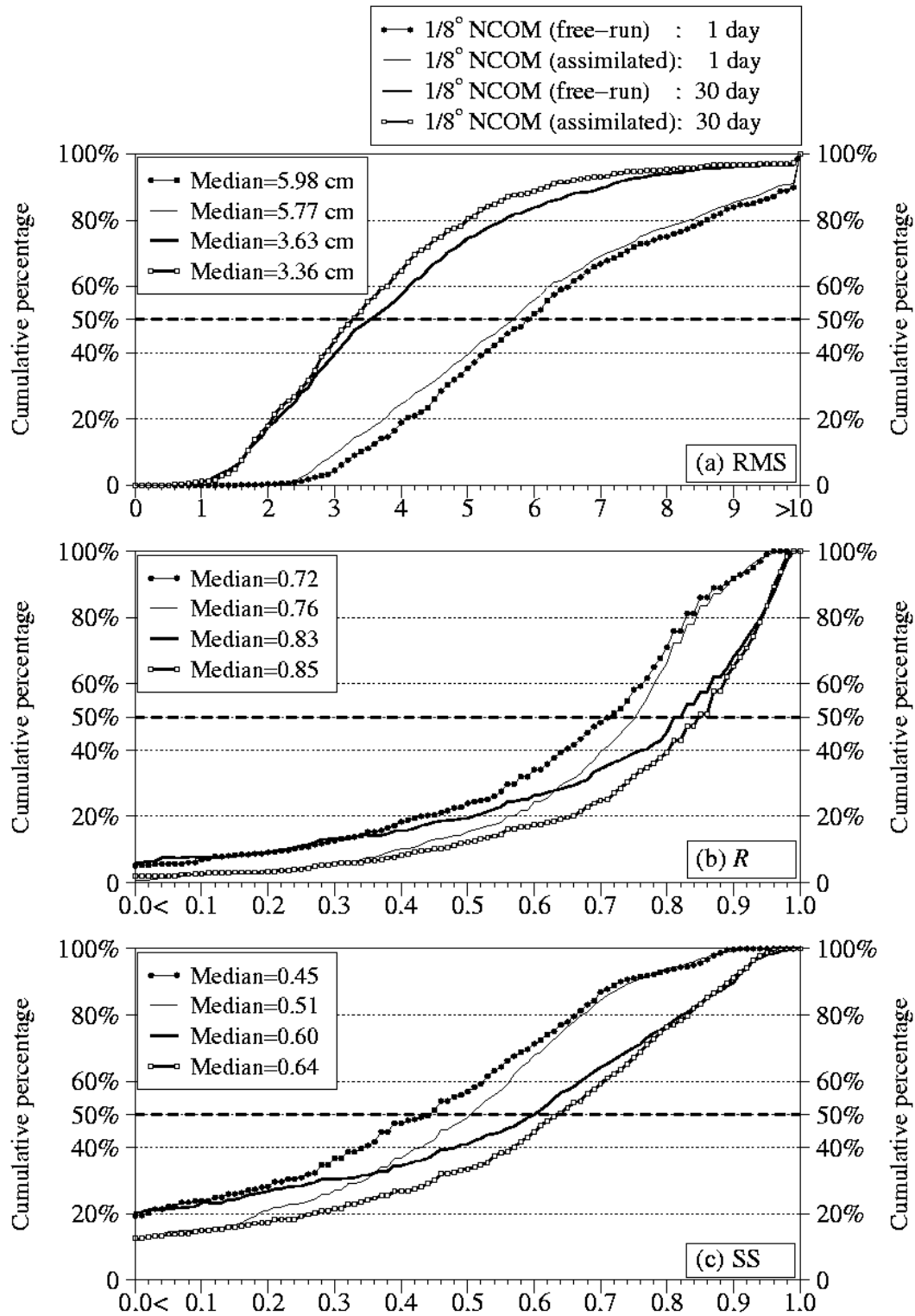
Fig. 46 – Cumulative percentage of RMS, R and SS values calculated using year-long SSH time series from all the tide gauges and 1/8° NCOM over the global ocean during 1998-2001. The results are shown for both free-running and data-assimilative 1/8° NCOM simulations when applying 1-day and 30-day running averages on the time series. Note that an inverse barometer correction has been applied to the tide gauge data before the statistical analysis.
