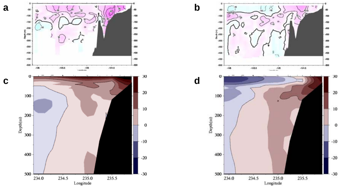
Fig. 89 – A Feb. 2000 comparison of northward velocity (cm/s) through a section at 44.6°N near Newport, Oregon. Sections from (a,b) ADCP surveys conducted as a part of the Northeast Pacific Long Term Observation Program at Oregon State University and (c,d) snapshots from the assimilative 1/8° global NCOM. Comparison of the ADCP surveys reveals a reversal in the offshore surface current between the (a) Feb. 1-2 section and (b) Feb. 2-3 section. A similar reversal is seen between the NCOM snapshots on (a) Feb 1 and (b) Feb 2. Note that the fine scale details of the bathymetry and currents are not resolved in the source bathymetry, the NOGAPS atmospheric forcing, or the 14-km grid spacing of global NCOM in this region.
