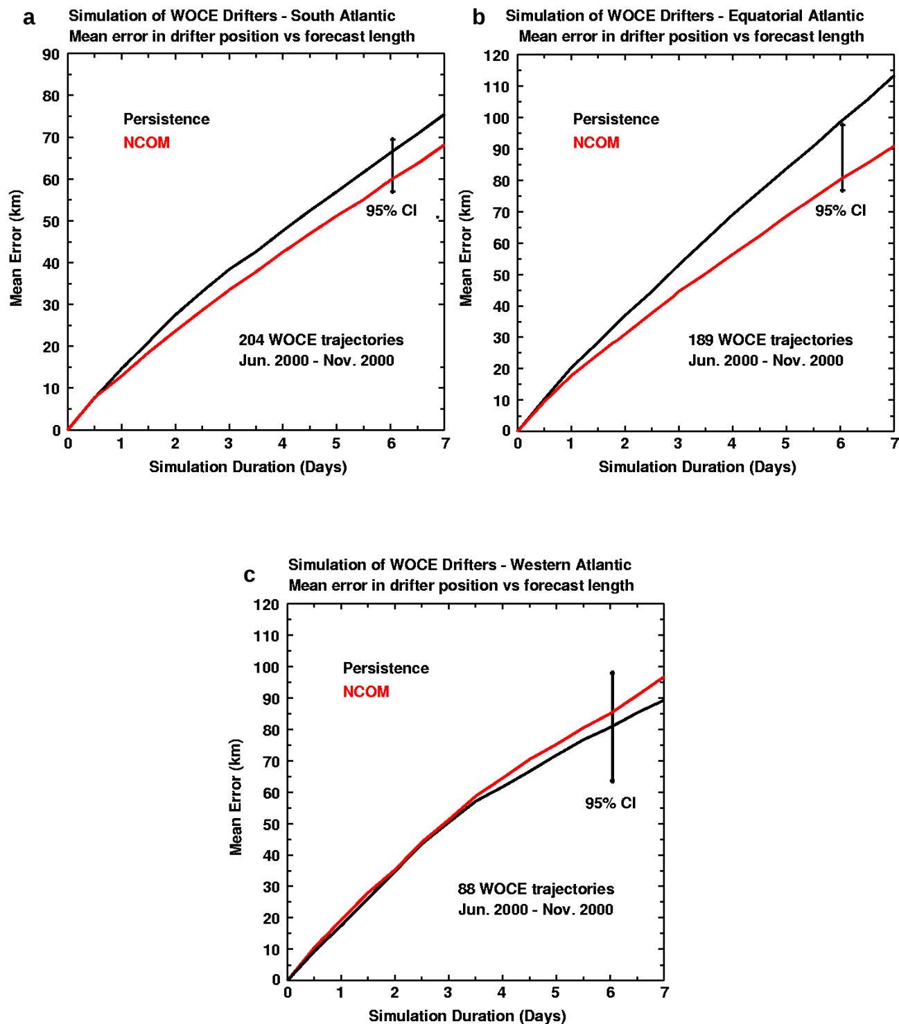
Fig. 61 – Summary of assimilative 1/8^\circ global NCOM validation using seven-day segments of WOCE drifter trajectories. The axes show mean separation between WOCE and NCOM drifters versus number of days of trajectory integration. These results are derived over (a) 204 drifter pairs in the South Atlantic, (b) 189 drifter pairs in the equatorial Atlantic, and (c) 88 drifter pairs in the western Atlantic. A 95% confidence interval for these statistics is indicated.
