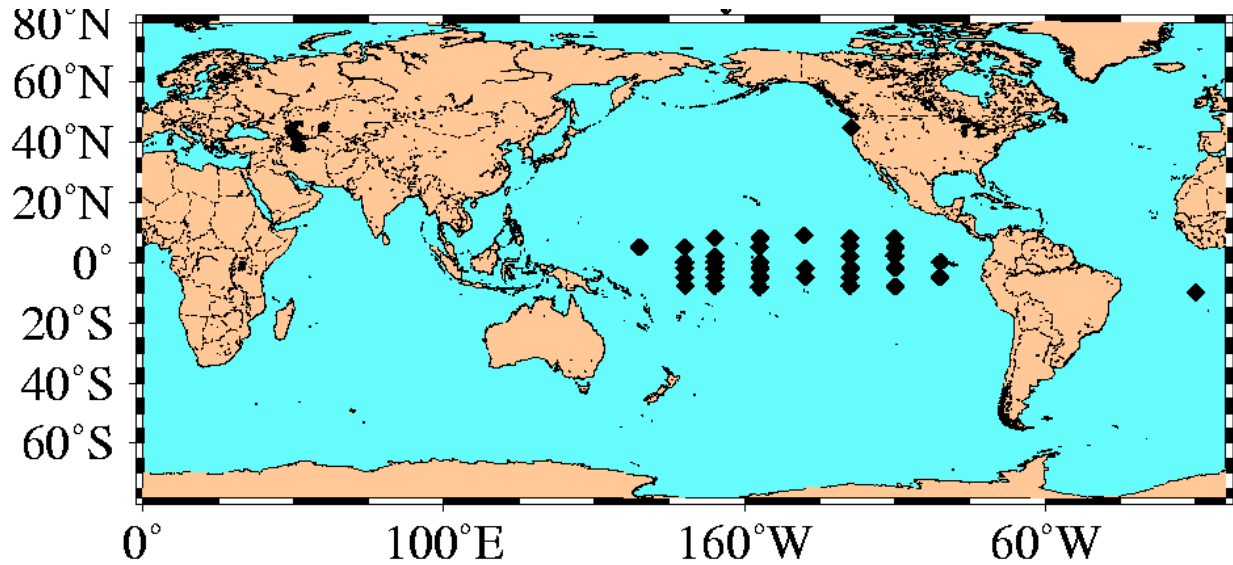
Fig. 57 – Locations of buoys providing 71 unassimilated, year-long buoy temperature profiles used for validation of NCOM mixed layer 1998-2000.
