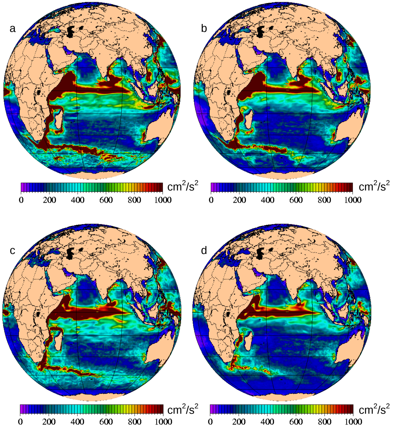
Fig. 14 – Indian hemispheric view of mean 1998-2000 surface kinetic energy (left; a, c) and surface EKE (right; b, d) for free-running (top; a, b) and assimilative (bottom; c, d) 1/8^\circ global NCOM. NCOM is forced with NOGAPS wind and thermal forcing. The assimilative case relaxes to MODAS synthetic temperature and salinity derived from 1/8^\circ MODAS2D SST and 1/16^\circ NLOM SSH.
