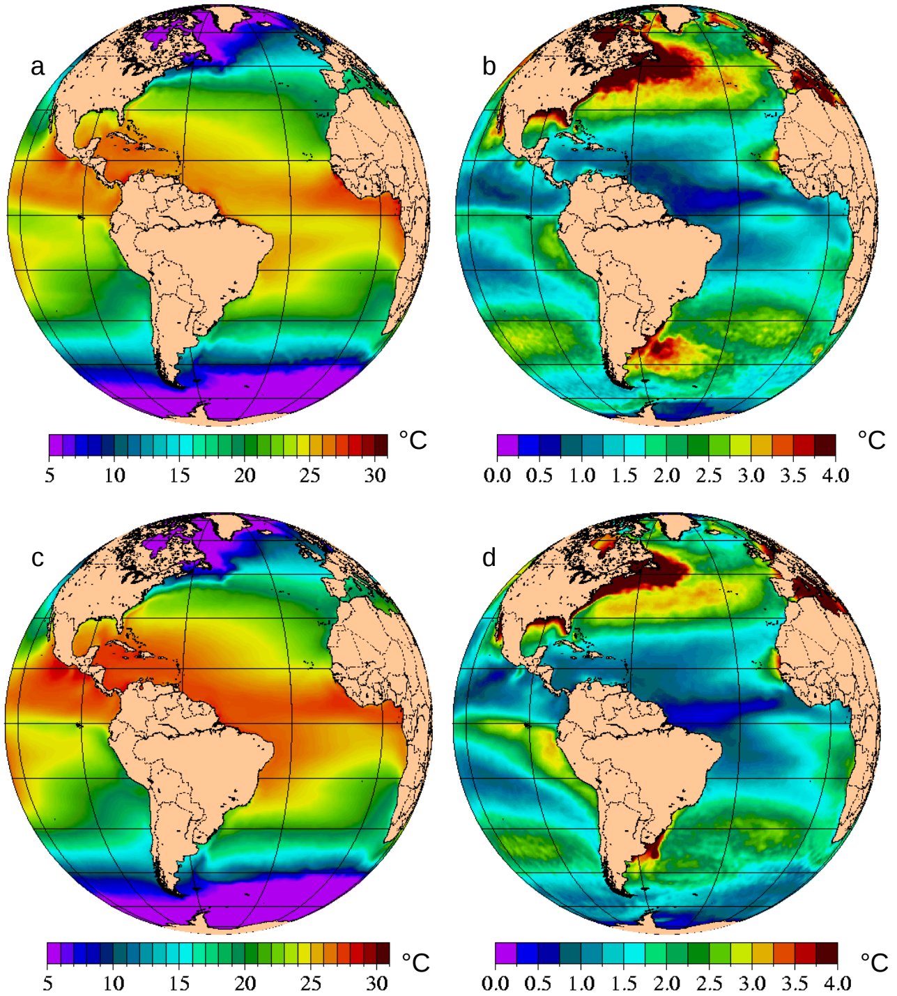
Fig. 6 – Atlantic hemispheric view of mean 1998-2000 SST (left;a,c) and SST standard deviation (right;b,d) for free-running (top;a,b) and assimilative (bottom;c,d) 1/8^\circ global NCOM. NCOM is forced with NOGAPS wind and thermal fluxes. The assimilative case relaxes to MODAS synthetic temperature and salinity derived from 1/8^\circ MODAS2D SST and 1/16^\circ NLOM SSH.
