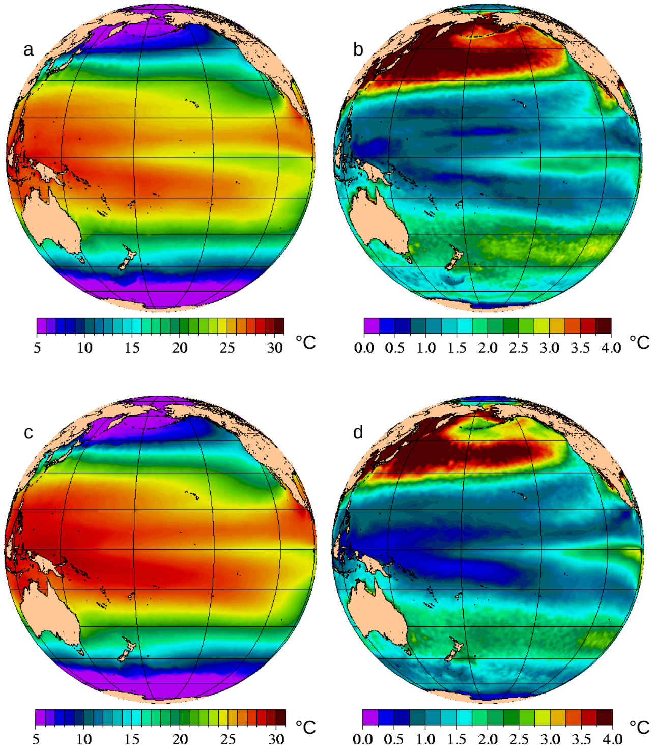
Fig. 16 – Pacific hemispheric view of mean 1998-2000 SST (left;a,c) and SST standard deviation (right;b,d) for free-running (top;a,b) and assimilative (bottom;c,d) 1/8° global NCOM. NCOM is forced with NOGAPS wind and thermal forcing. The assimilative case relaxes to MODAS synthetic temperature and salinity derived from 1/8° MODAS2D SST and 1/16° NLOM SSH.
