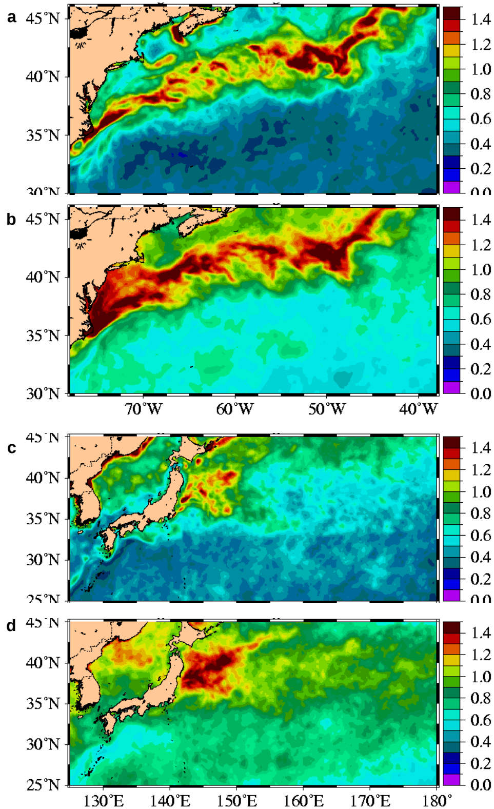
Fig. 84 – Mean 7-day 1/8° global NCOM (a,c) forecast and (b,d) persistence error in SST (°C) relative to subsequent global NCOM nowcasts for forecasts from 1998-2002 in the (a,b) Gulf Stream and (c,d) Kuroshio regions. The forecast has generally smaller errors than persistence except in narrow bands immediately adjacent to the coast, where forecast errors are quite high. We attribute these errors to inadequate land masking in the global atmospheric forcing, resulting in application of flux values appropriate for land areas near the land-sea boundary.
