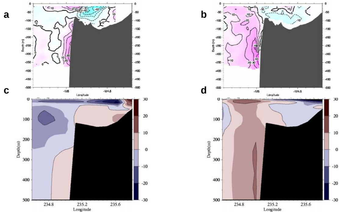
Fig. 92 – 2002 comparisons of northward velocity (cm/s) through a section at 44.0^{\circ}\text{N} near Heceta Head, Oregon. Sections from (a,b) ADCP surveys conducted as a part of the Northeast Pacific Long Term Observation Program and (c,d) snapshots from the assimilative 1/8^{\circ} global NCOM. The 9-10 Apr. observations (a) show a midsection eddy and a strong northward boundary layer jet along the slope are not present in the (c) 10 Mar. model results. The (b) 14-15 July observations and (d) 14 July NCOM snapshot are quite similar, but again the intense northward boundary layer jet along the slope is present in the observations but not resolved by the model.
