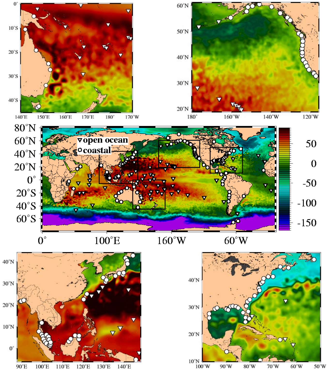
Fig. 40 – Tide gauge locations superimposed on a snapshot of SSH from the data-assimilative 1/8° global NCOM. All the tide gauges are maintained by the University of Hawaii JASL center and are located in both coastal and open ocean island regions of the Atlantic, Pacific and Indian Oceans. The tide gauges are separated into two categories located at (circles) coastal regions and (triangles) islands in the open ocean.
