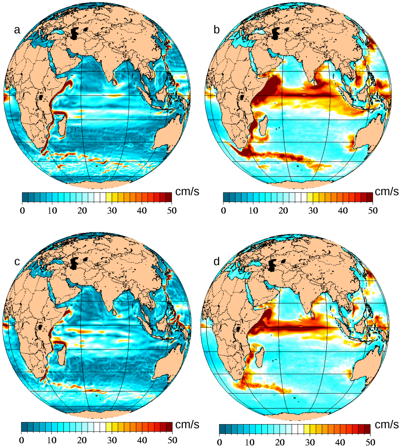
Fig. 13 – Indian hemispheric view of mean 1998-2000 surface speed (left; a,c) and surface speed standard deviation (right; b,d) for free-running (top; a,b) and assimilative (bottom; c,d) 1/8^\circ global NCOM. NCOM is forced with NOGAPS wind and thermal forcing. The assimilative case relaxes to MODAS synthetic temperature and salinity derived from 1/8^\circ MODAS2D SST and 1/16^\circ NLOM SSH.
