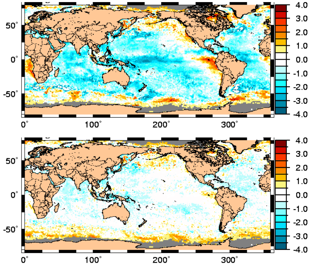
Fig. 52 – Global plots of differences between mean monthly SST for October 2000: (a) free-running 1/8° global NCOM – 9km Pathfinder, and (b) assimilative 1/8° global NCOM - 9km Pathfinder. NCOM tends to be warmer at high latitudes and along the eastern boundaries, and cooler over most of the central ocean. The deviations are much larger in the free-running case with similar distribution of the trends.
