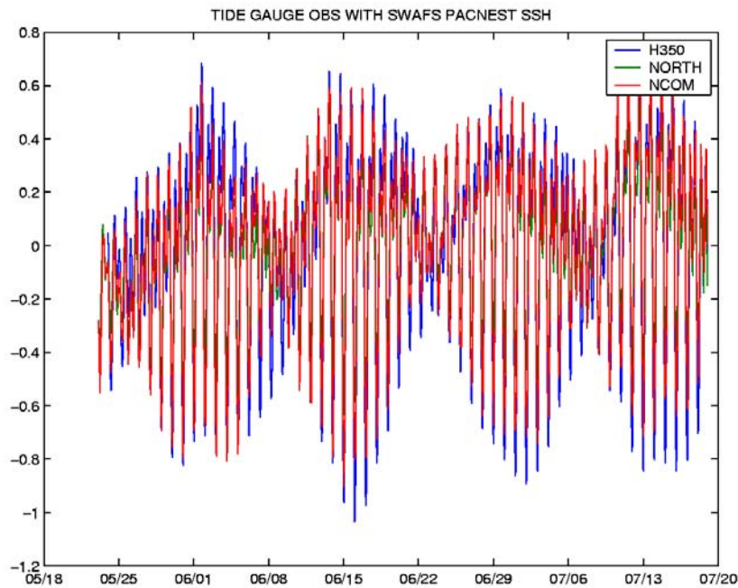
Fig. 111 – Example of the water level time series from station 350 (blue), with the corresponding time series from the SWAFS pacnest runs using SWAFS northworld boundary conditions (green) and NCOM/OSU boundary conditions (red), for the full time series 24 May to 19 July 2003. The time series have the means individually removed before plotting.
