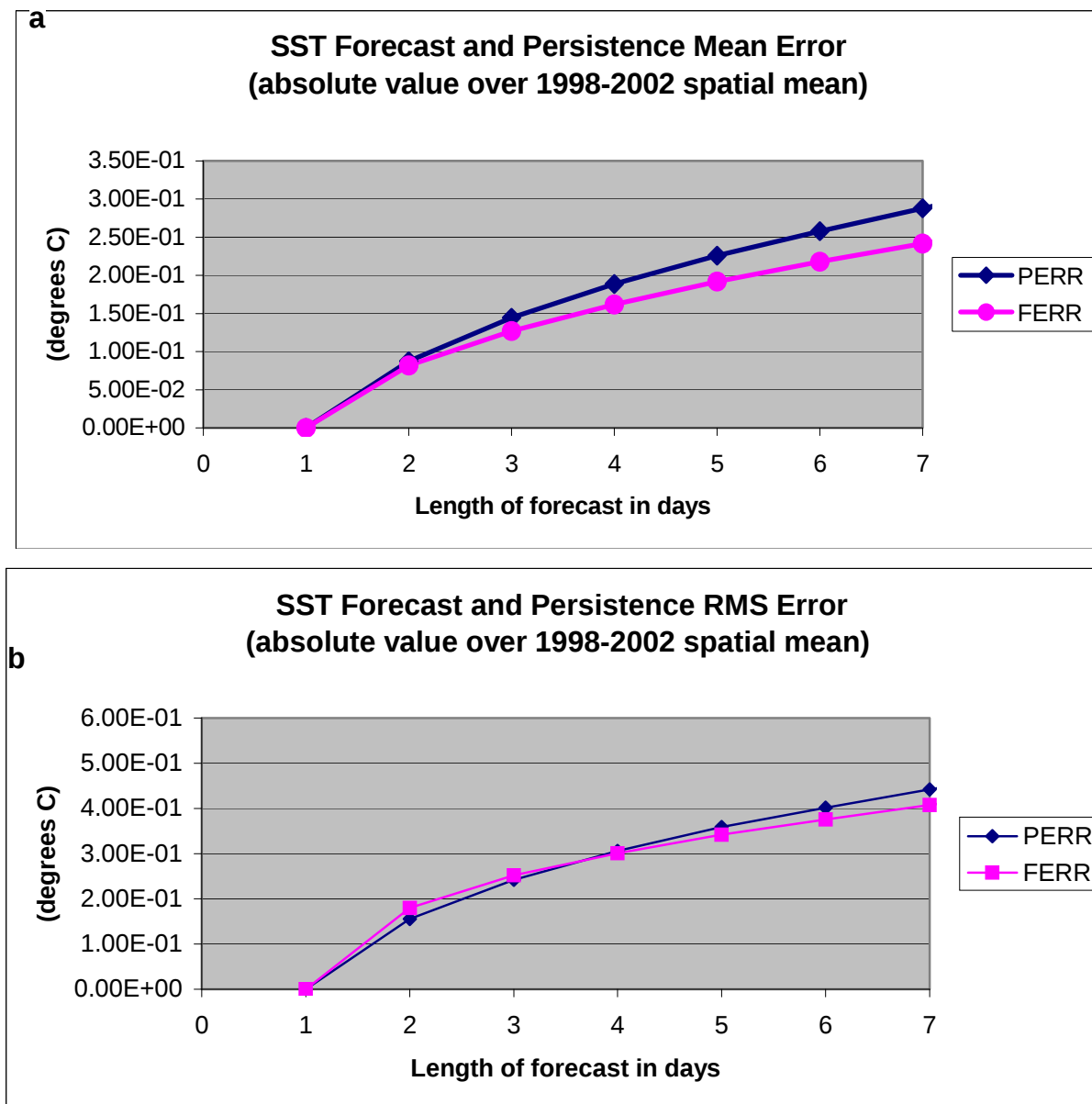
Fig. 81 – SST forecast and persistence error comparisons versus forecast length up to seven days for 1/8^\circ global NCOM. Calculated from bimonthly 7-day forecasts from 1998-2002. (a) mean absolute error in SST and (b) square root of mean squared error in SST. Means are calculated in space over the global ocean and in time over 1998-2002. Error is relative to the NCOM analysis valid on zero hours of each forecasted day. Forecast error is consistently smaller than persistence, but less so than for SSH. Relatively large forecasts errors adjacent to the coast and cold forecasts biases degrade the overall forecast performance.
