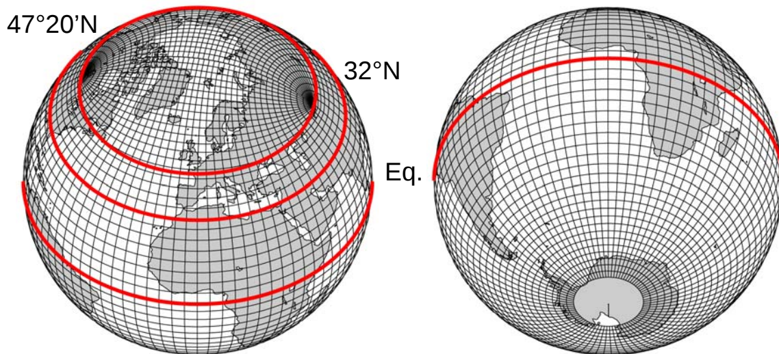
Fig. 2 – An illustration of the horizontal grid used in global NCOM. The equator is delineated in red, as are the limits of the transition zone between 32°N and 47°20'N. By placing poles in Russia and Canada, grid distortion is minimized over oceanic portions of the domain.
