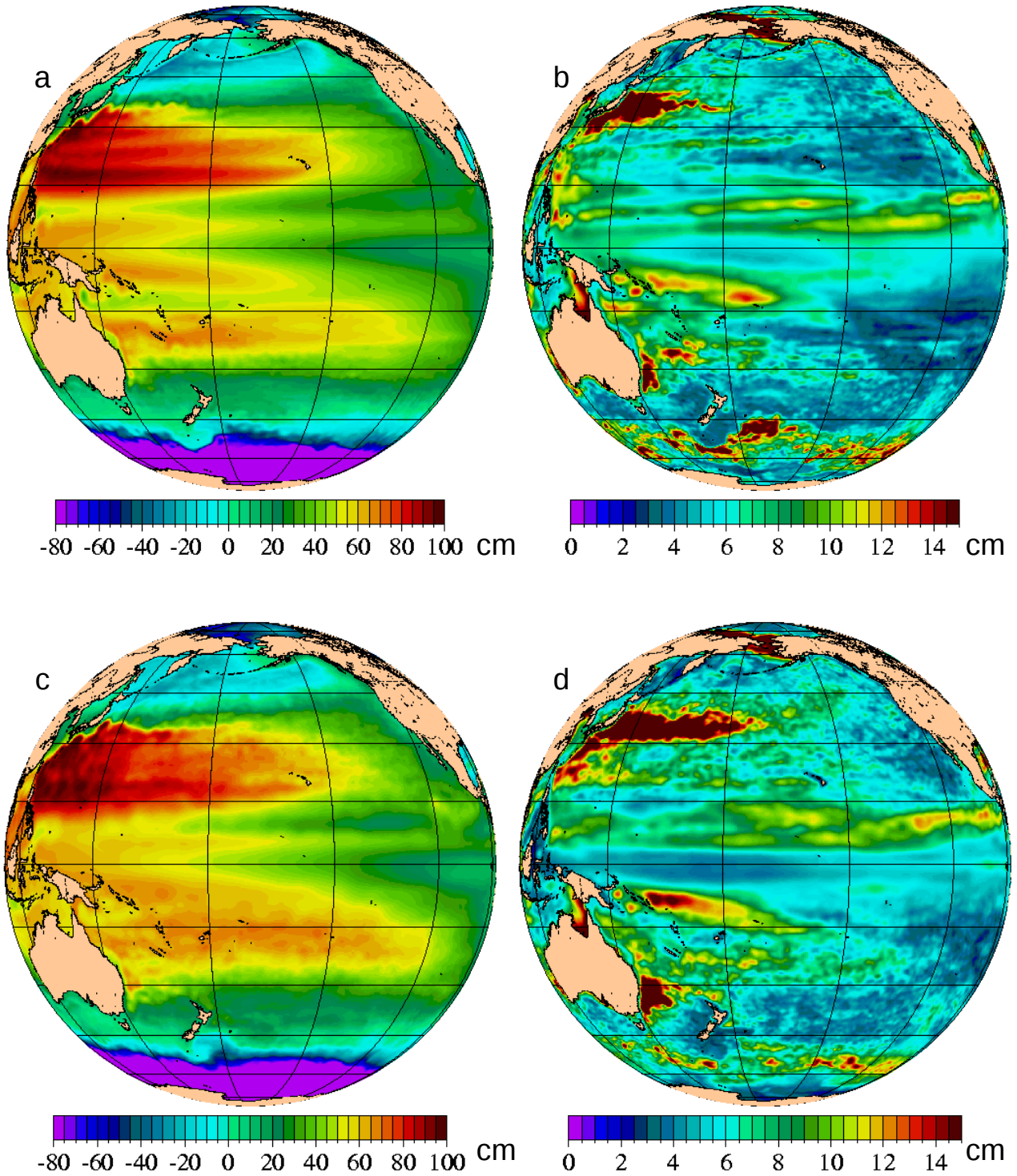
Fig. 15 – Pacific hemispheric view of mean 1998-2000 SSH (left;a,c) and SSH standard deviation (right;b,d) for free-running (top;a,b) and assimilative (bottom;c,d) 1/8^\circ global NCOM. NCOM is forced with NOGAPS wind and thermalforcing. The assimilative case relaxes to MODAS synthetic temperature and salinity derived from 1/8^\circ MODAS2D SST and 1/16^\circ NLOM SSH.
