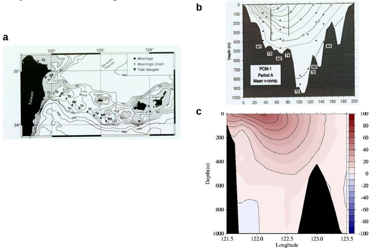
Fig. 74 – Velocity section along the WOCE PCM_1 line east of Taiwan. (a) Locations of the PCM-1 current meters. (b) Contours of northward speed from PCM-1 data September 1995 to May 1996. (c) Contours of northward speed from assimilative 1/8° global NCOM 1998-2000 mean. (a) and (b) are from Lee et al. (2001).
