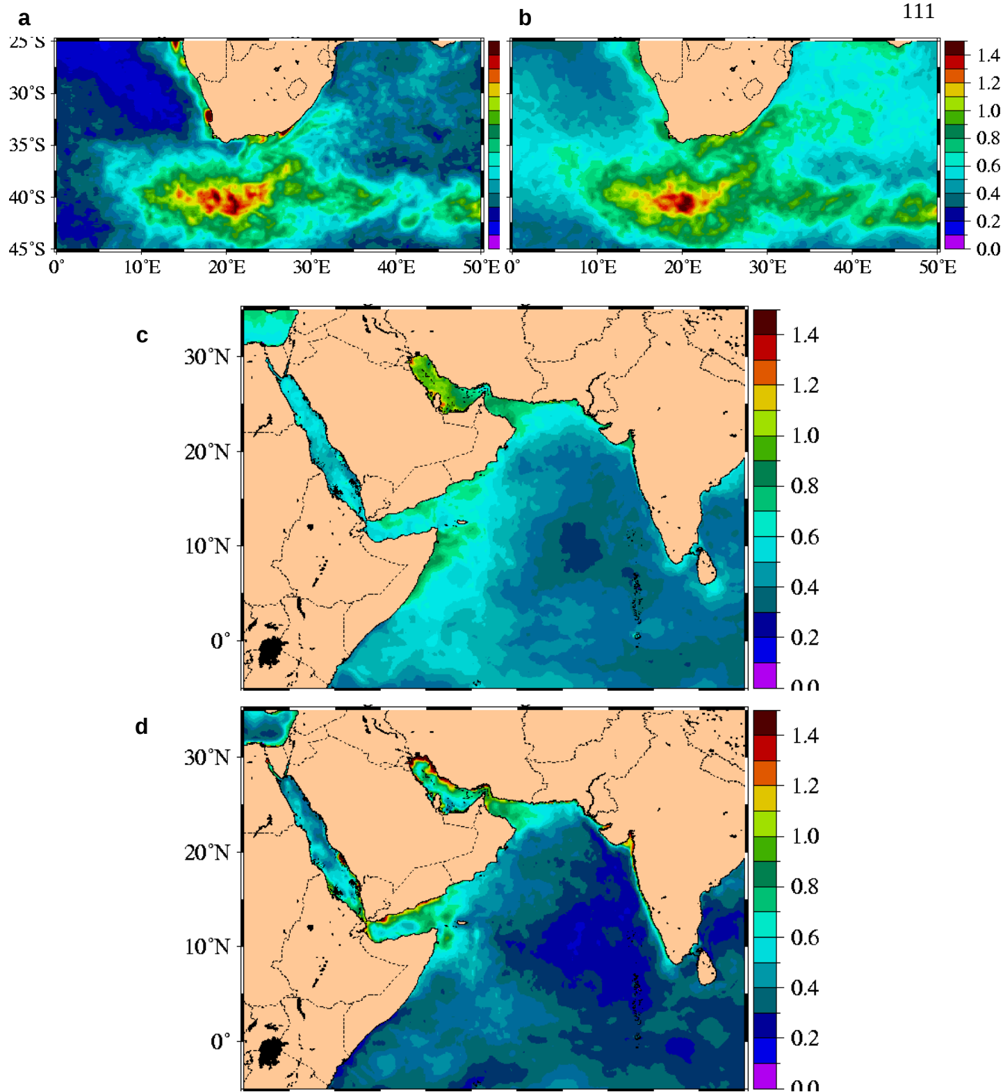
Fig. 85 – Mean 7-day 1/8^\circ global NCOM (a,c) forecast and (b,d) persistence error in SST ( ^\circ\text{C} ) relative to subsequent global NCOM nowcasts for forecasts from 1998-2002 in the (a,b) Agulhas and (c,d) Arabian Sea regions. The forecast has generally smaller errors than persistence except in narrow bands immediately adjacent to the coast, where forecast errors are quite high. We attribute these errors to inadequate land masking in the global atmospheric forcing, resulting in application of flux values appropriate for land areas near the land-sea boundary.
