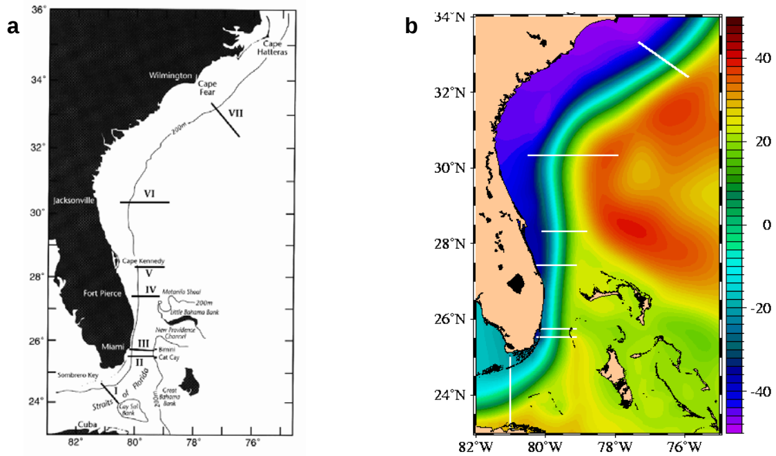
Fig. 62 – Locations of sections of downstream speed contours across the Florida Current. (a) Illustration from Schmitz (1996) based on dropsonde data and adapted from Richardson et al. (1969). (b) Global NCOM 1998-2000 SSH mean with several sections. Superimposed white lines locate vertical sections extracted from NCOM for validation.
