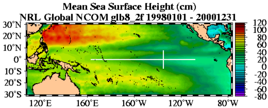
Fig. 75 – Global NCOM 1998-2000 SSH mean in the equatorial Pacific. White lines locate vertical current sections extracted from NCOM for comparison with historical observation means.
