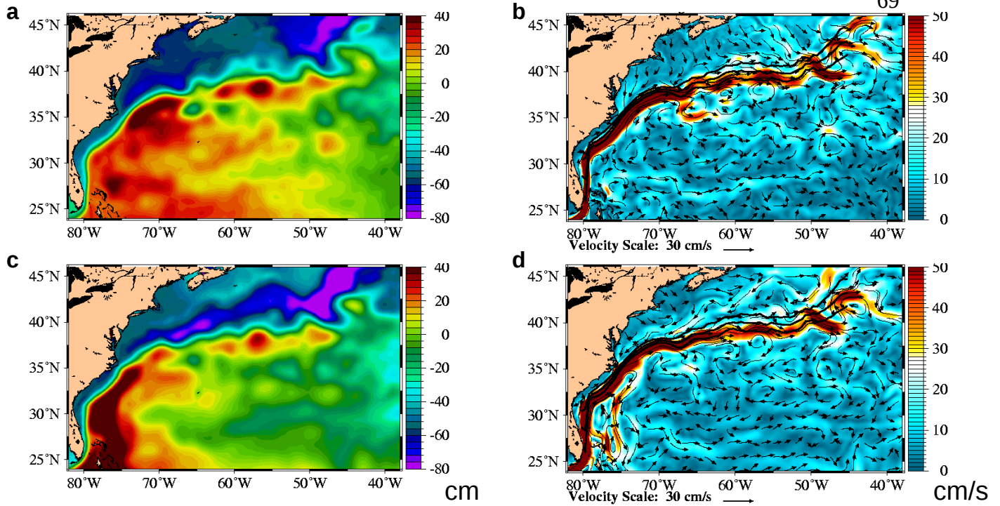
Fig. 26 – Gulf Stream zoom of mean SSH (left;a,c) and surface speed with superimposed currents (right;b,d) for assimilative 1/8^\circ global NCOM (top;a,b) and assimilative 1/4^\circ SWAFS Northworld (bottom;c,d). Superimposed black curves are the mean and mean \pm 1 standard deviation fronts from the NAVOCEANO Gulf Stream north wall boguses from archives over the same time period. Mean is over period of available SWAFS surface data, 9/1/2002-5/31/2003. To enable the same color bar and ranges to be used, mean SWAFS SSH is offset to equal mean NCOM SSH over this domain.
