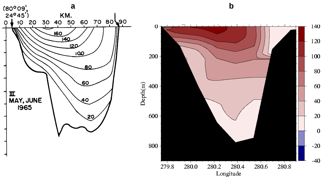
Fig. 65 – Comparison of mean currents through Florida Current section III. (a) downstream speed contours from Schmitz (1996) with observations from May-June 1965 and (b) northward speed contours from assimilative 1/8^{\circ} global NCOM 1998-2000 mean section at 25.75^{\circ}\text{N} , 80.0^{\circ}\text{W} - 79.1^{\circ}\text{W} .
