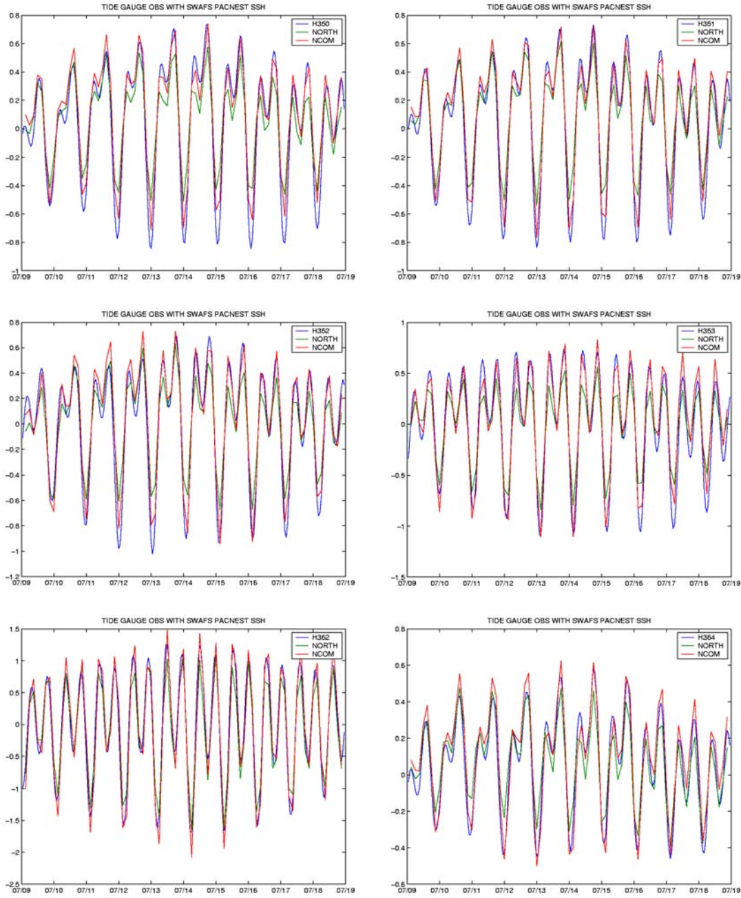
Fig. 112 – Water level time series from the six GLOSS stations used for this validation. For each station (a-f), the observed water level (blue), SWAFS pacnest run using SWAFS northworld boundary conditions (green), and SWAFS pacnest run using NCOM/OSU boundary conditions (red), are show for the last 10 d of the time series. The time series have the means individually removed before plotting.
