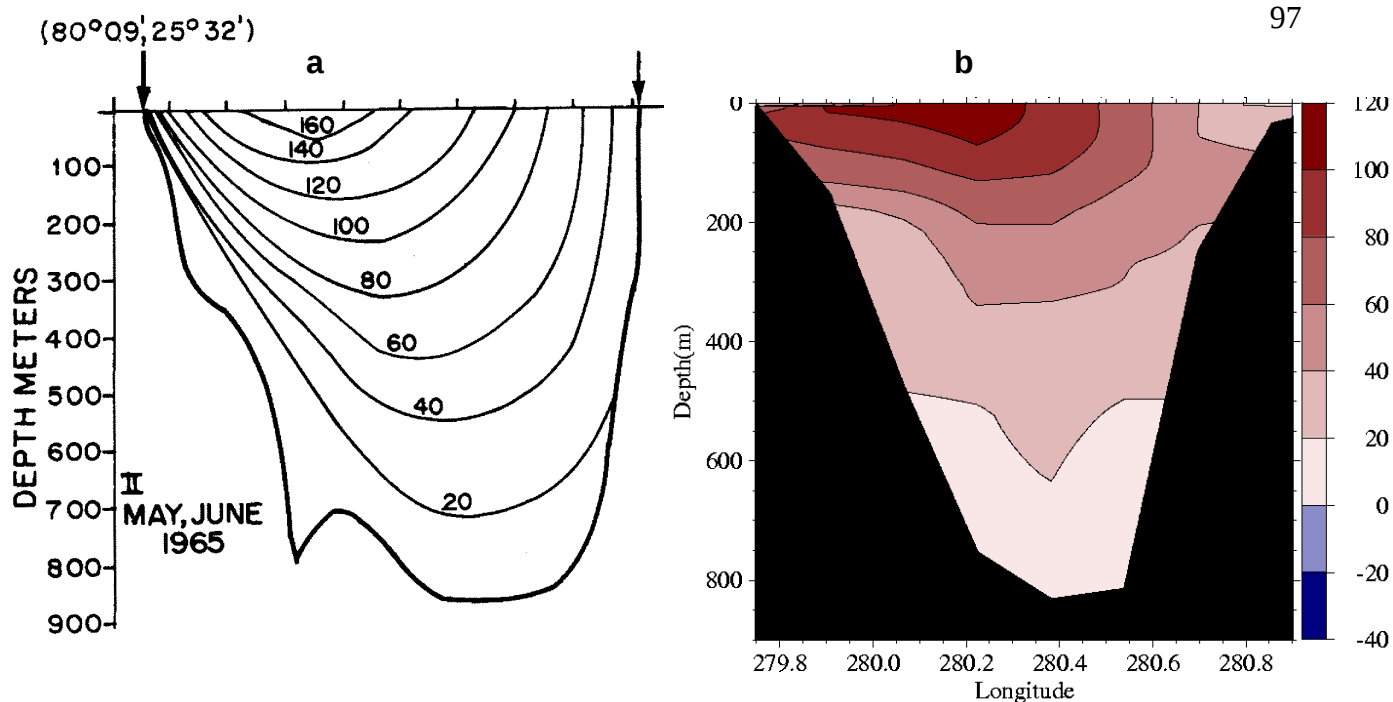
Fig. 64 – Comparison of mean currents through Florida Current section II. (a) downstream speed contours from Schmitz (1996) with observations from May-June 1965 and (b) northward speed contours from assimilative 1/8^{\circ} global NCOM 1998-2000 mean section at 25.5^{\circ}\text{N} , 80.0^{\circ}\text{W} - 79.1^{\circ}\text{W} .
