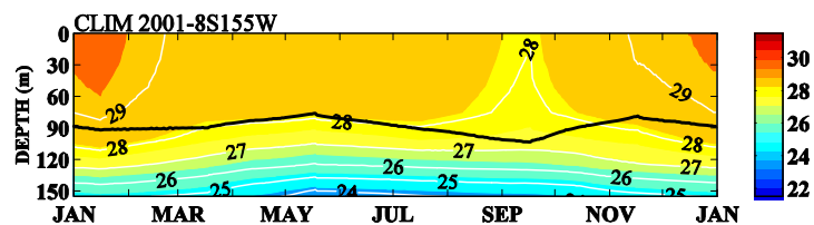
Fig. 58 – Time-series from 2001 at a TAO buoy location in the equatorial Pacific (8°S, 155°W). The bottom series indicates the MODAS climatological background. Using real-time MODAS SST and NLOM SSH, the MODAS dynamic climatology produces a field which is assimilated into global NCOM. The ability of global NCOM to resolve the mixed-layer dynamics allows it to produce a mixed-layer depth (black line on each series) in closer agreement with the variability measured in the observations.
