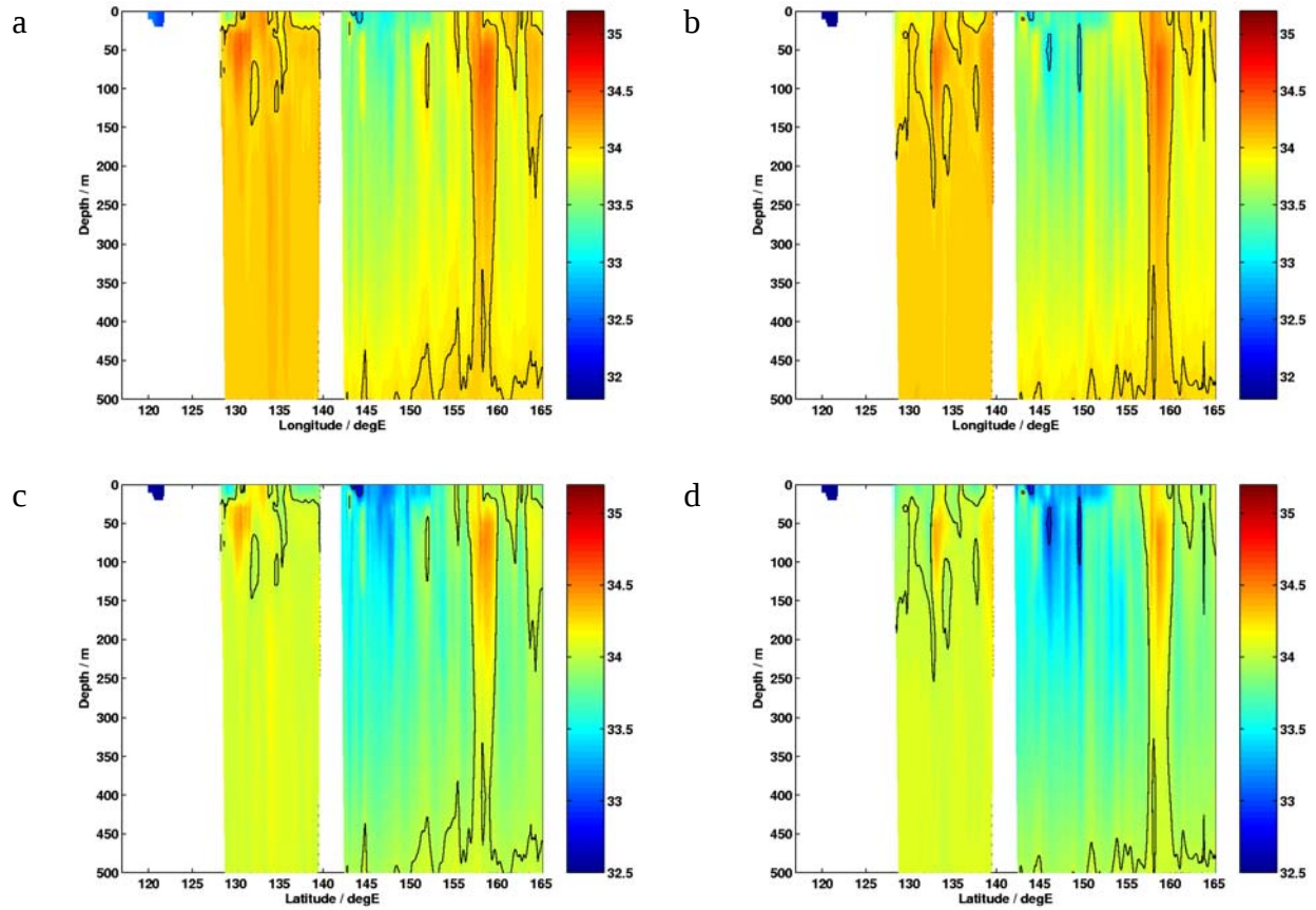
Fig. 101 Salinity from SWAFS pacnest restart files valid 19 July 2003 using SWAFS northworld boundary conditions (a,c) and NCOM/OSU boundary conditions (b,d) from the surface to 500m along 40N (a,b) and 150E (c,d).
