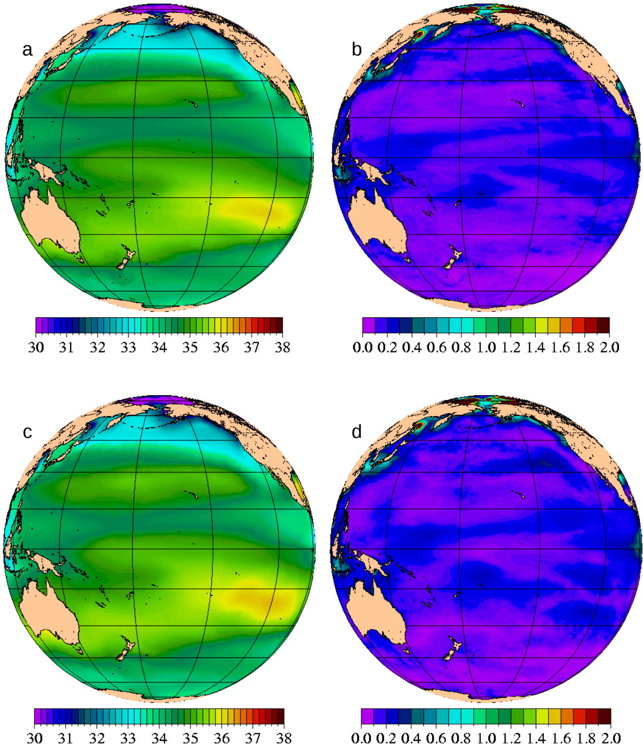
Fig. 17 – Pacific hemispheric view of mean 1998-2000 SSS (left; a, c) and SSS standard deviation (right; b, d) for free-running (top; a, b) and assimilative (bottom; c, d) 1/8^\circ global NCOM. NCOM is forced with NOGAPS wind and thermal forcing. The assimilative case relaxes to MODAS synthetic temperature and salinity derived from 1/8^\circ MODAS2D SST and 1/16^\circ NLOM SSH.
