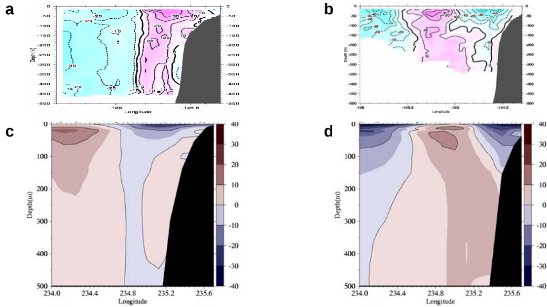
Fig. 93 – Northward velocity (cm/s) through Oregon coast sections from (a,b) ADCP surveys conducted as a part of the Northeast Pacific Long Term Observation Program and (c,d) snapshots from the (b) assimilative 1/8^\circ global NCOM. At 43.2^\circ\text{N} , the (a) 24-25 Sep. 1999 ADCP survey shows currents opposite to those seen in the (c) 24 Sep. 1999 NCOM snapshot. Good agreement is found on 13 Jul. 2002 at 41.9^\circ\text{N} , when both the (b) observations and (d) model indicate a deep, surface-intensified northward flow flanked by surface intensified southward currents.
