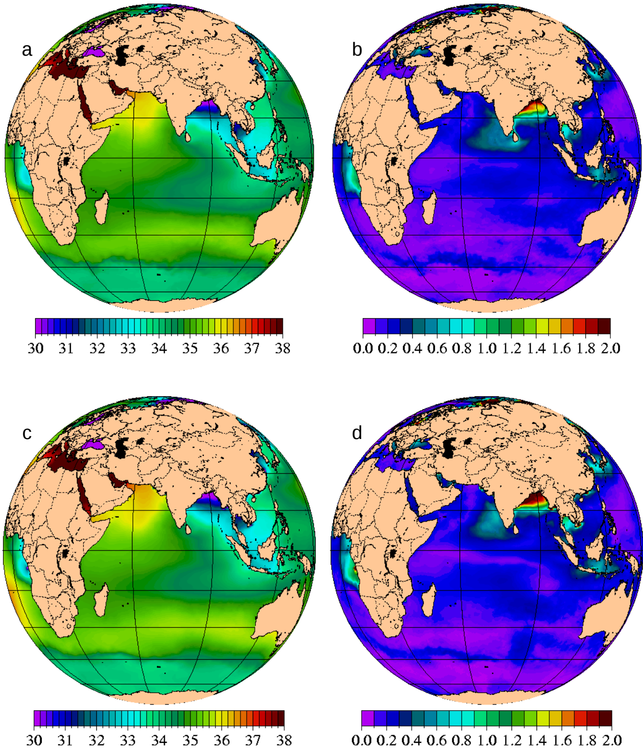
Fig. 12 – Indian hemispheric view of mean 1998-2000 SSS (left;a,c) and SSS standard deviation (right;b,d) for free-running (top;a,b) and assimilative (bottom;c,d) 1/8° global NCOM. NCOM is forced with NOGAPS wind and thermal forcing. The assimilative case relaxes to MODAS synthetic temperature and salinity derived from 1/8° MODAS2D SST and 1/16° NLOM SSH.
