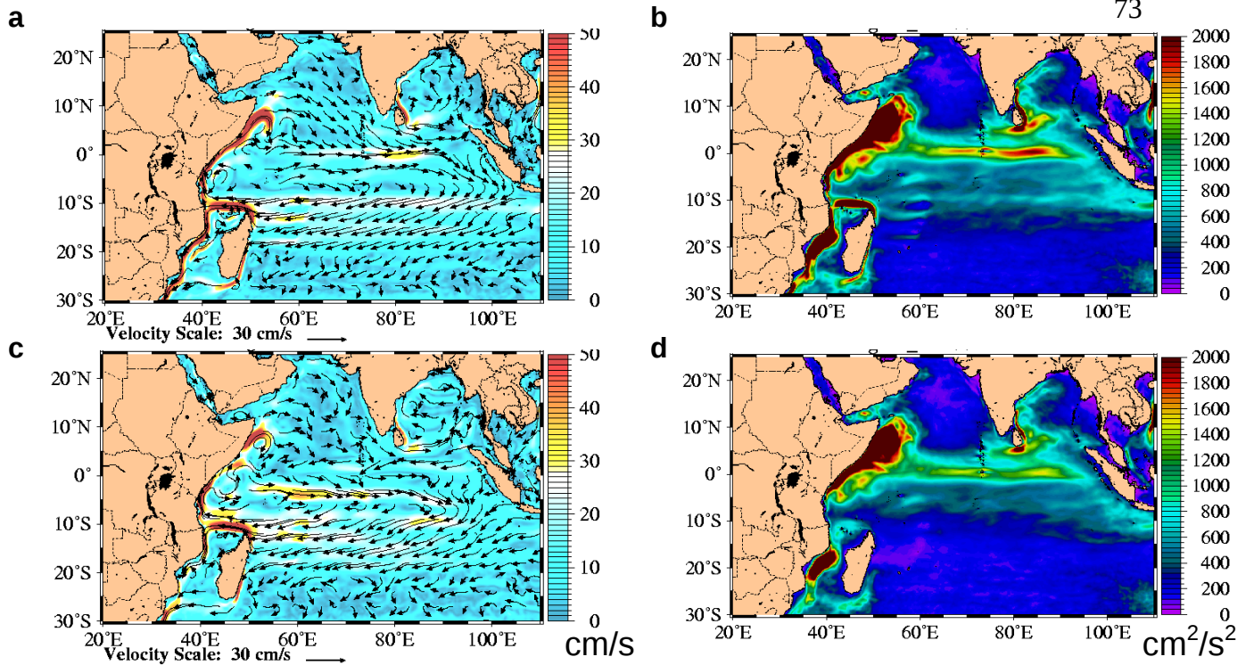
Fig. 33 – Indian Ocean zoom of mean 1998-2000 surface speed with superimposed currents (left; a, c) and surface EKE (right; b, d) for free-running (top; a, b) and assimilative (bottom; c, d) 1/8° global NCOM.
