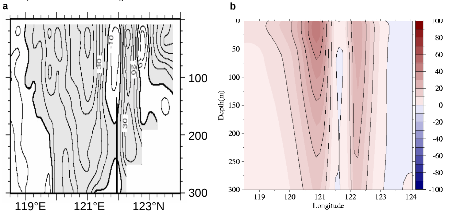
Fig. 71 – Velocity section across the upper 300m of the Luzon Strait, 120°75'E between Taiwan and Luzon. (a) Contours of eastward speed from Sb-ADCP observations from Liang et al. (2003) and (b) contours of eastward speed from assimilative 1/8° global NCOM 1998-2000 mean.
