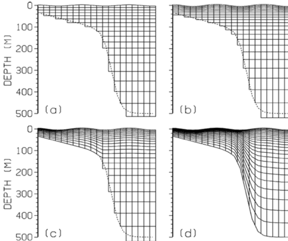
Fig. 1 – An illustration of the NCOM vertical grid: (a) a single \sigma -level at the surface and z-levels below, (b) several \sigma -levels at the surface with z-levels below, (c) \sigma -levels to a depth over most of the shelf and z-levels to the bottom over the slope and abyss, or (d) \sigma -levels everywhere. Global NCOM follows case c with a \sigma -z transition at 137m.
