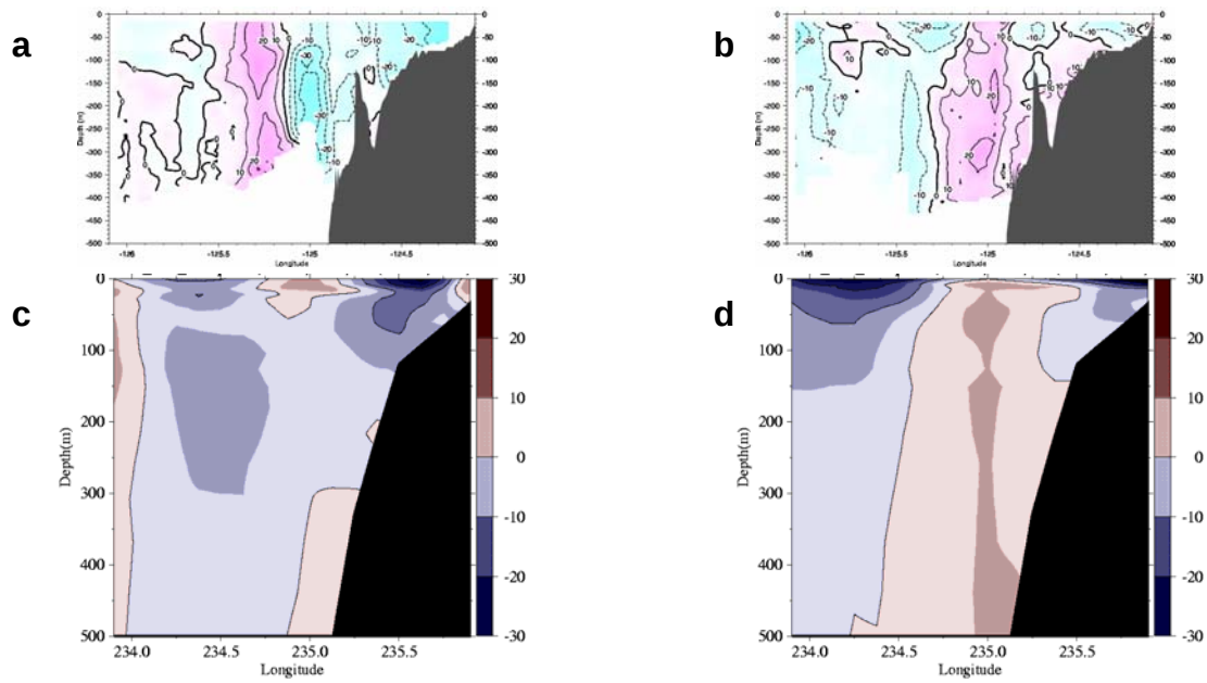
Fig. 91 – 2001 comparisons of northward velocity (cm/s) through a section at 44.6^{\circ}\text{N} near Newport, Oregon. Sections from (a,b) ADCP surveys conducted as a part of the Northeast Pacific Long Term Observation Program and (c,d) snapshots from the assimilative 1/8^{\circ} global NCOM. The midsection eddy in (a) the 20-21 Mar. ADCP line is missing at depth and misplaced at the surface in (b) the 20 Mar. NCOM results. In contrast, the 5 Sep. NCOM section (d) is in good agreement with the larger scale features in the (b) 4-6 Sep. survey, although there is more observed variation in the offshore southward surface jet.
