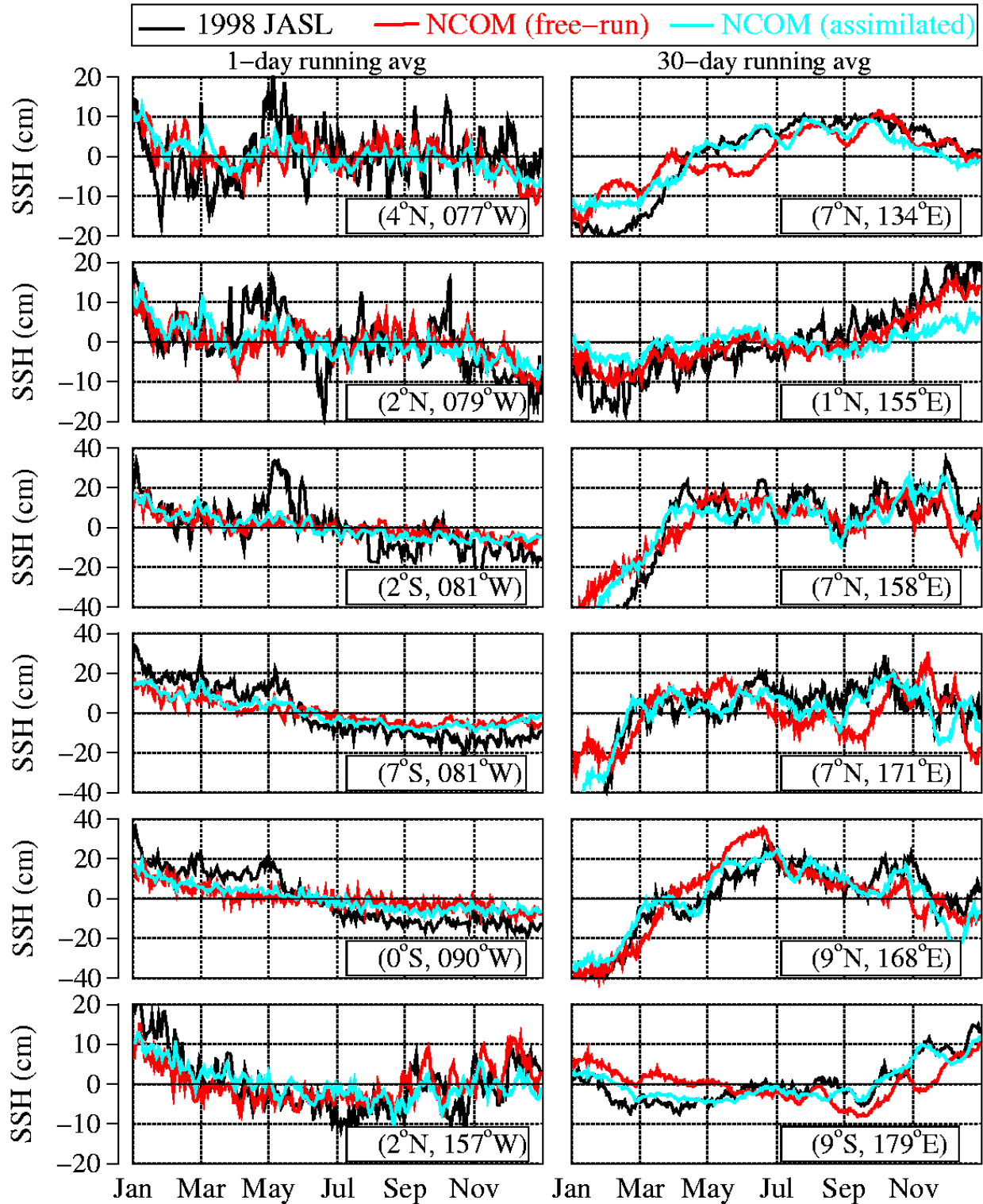
Fig. 42 – Daily SSH time series comparisons between the JASL and 1/8° NCOM values at various tide gauge locations in 1998. Note that the inverse barometer correction is already applied to SSH at each tide gauge. Model results are shown from free-running and data-assimilative NCOM simulations, separately. The right panels show results with a 30-day running average applied to daily SSH from tide gauges and NCOM simulations.
