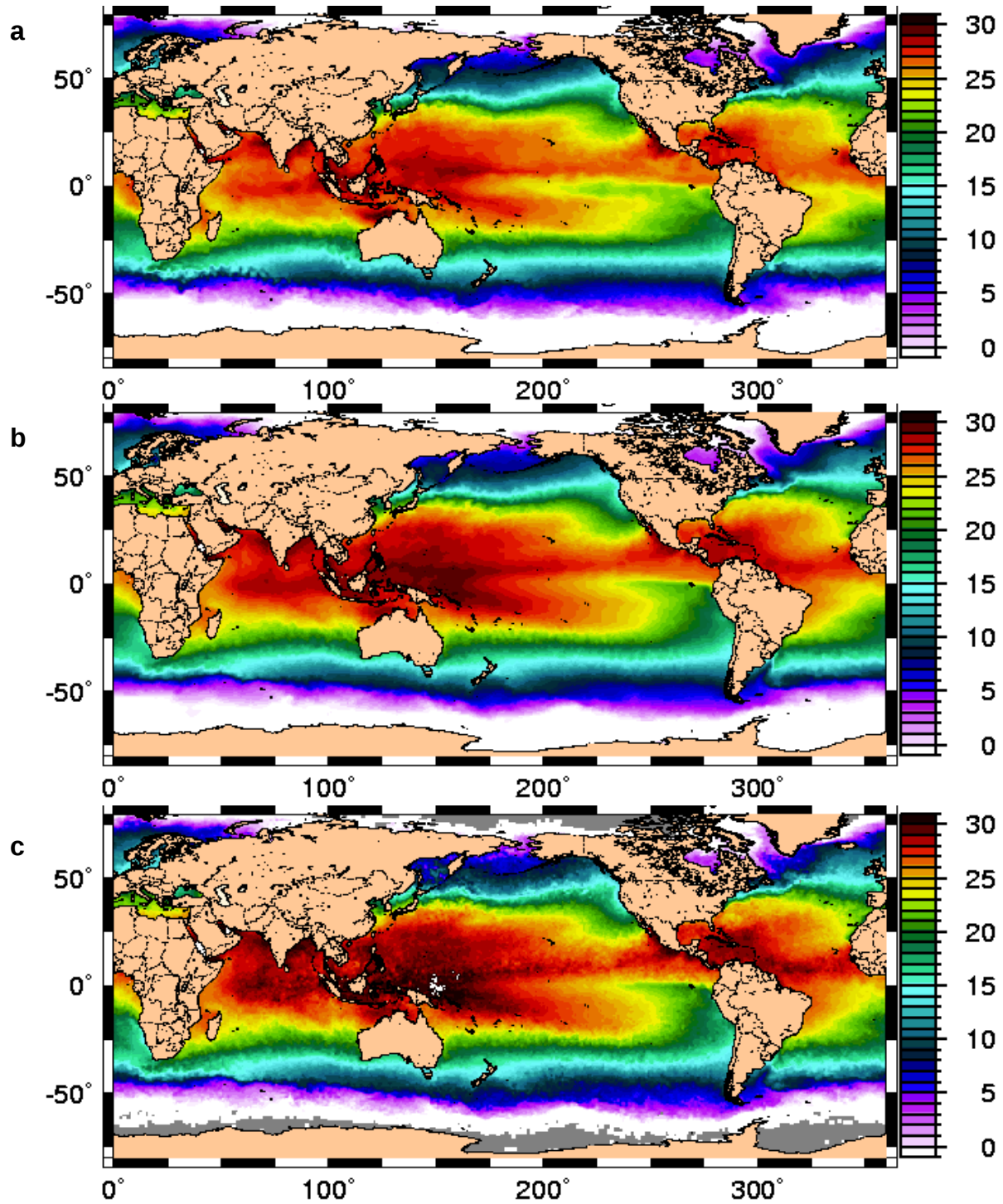
Fig. 51 – Global plots of mean SST for October 2000: (a) free-running 1/8° global NCOM, (b) assimilative 1/8° global NCOM, and (c) 9km Pathfinder. The NCOM means are calculated from daily snapshots, while the Pathfinder mean is a mean in each cell of the observations during the month in that cell. Grey areas have no observations during the month and are excluded further statistical analyses. Note that the NCOM means are noticeably smoother than the Pathfinder composite mean. Free running NCOM is noticeably cooler than the others.
