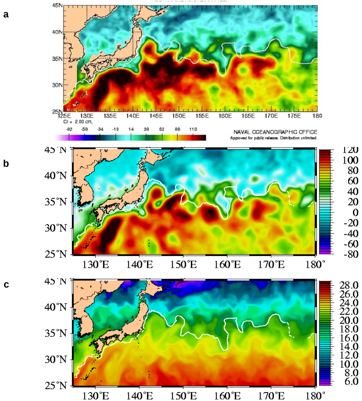
Fig. 86 – Surface plots from the Kuroshio region east of Japan for 22 November 2001. (a) SSH from operational 1/16° global NLOM, (b) SSH from assimilative 1/8° global NCOM, and (c) SST from assimilative 1/8° global NCOM. Superimposed on each plot in white is the NAVOCEANO IR frontal analysis of the Kuroshio north wall for the same date. Since the horizontal resolution of global NCOM is insufficient in some regions for skill in lengthy SSH forecasts, global NLOM depends on data assimilation to improve placement of fronts and eddies in regions such as the Kuroshio and Gulf Stream. Comparison between the front location and NCOM shows that the assimilation of synthetic T and S successfully transmits information from global NLOM necessary for global NCOM to accurately locate and forecast front and eddy location.
