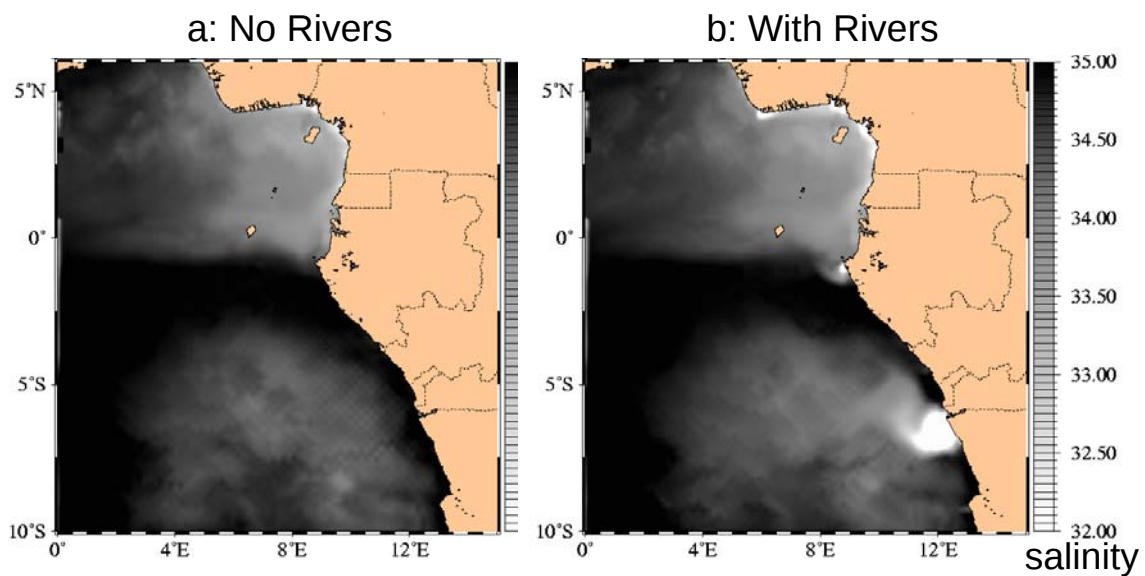
Fig. 4 – Snapshots of surface salinity along the coast of West Africa in June 1997 global NCOM simulations (a) without and (b) with rivers. Although relaxation to MODAS surface salinity does produce realistic distribution in the open ocean, in coastal regions, including major rivers significantly modifies nearshore salinity stratification.
