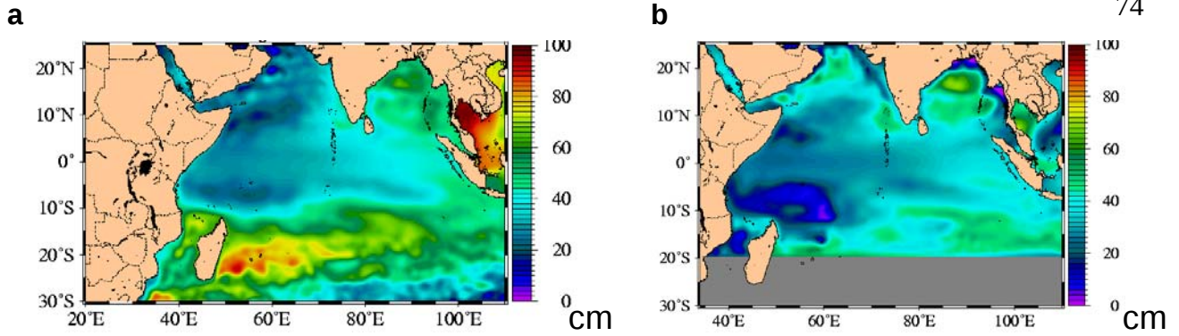
Fig. 35 – Indian Ocean zoom of mean SSH for assimilative 1/8° global NCOM (a) and assimilative 1/4° SWAFS Northworld (b). Mean is over winter monsoon period, 11/15/2002 – 3/15/2003. To enable the same color bar and ranges to be used, the mean SWAFS SSH is offset to equal the mean NCOM SSH over this domain.
