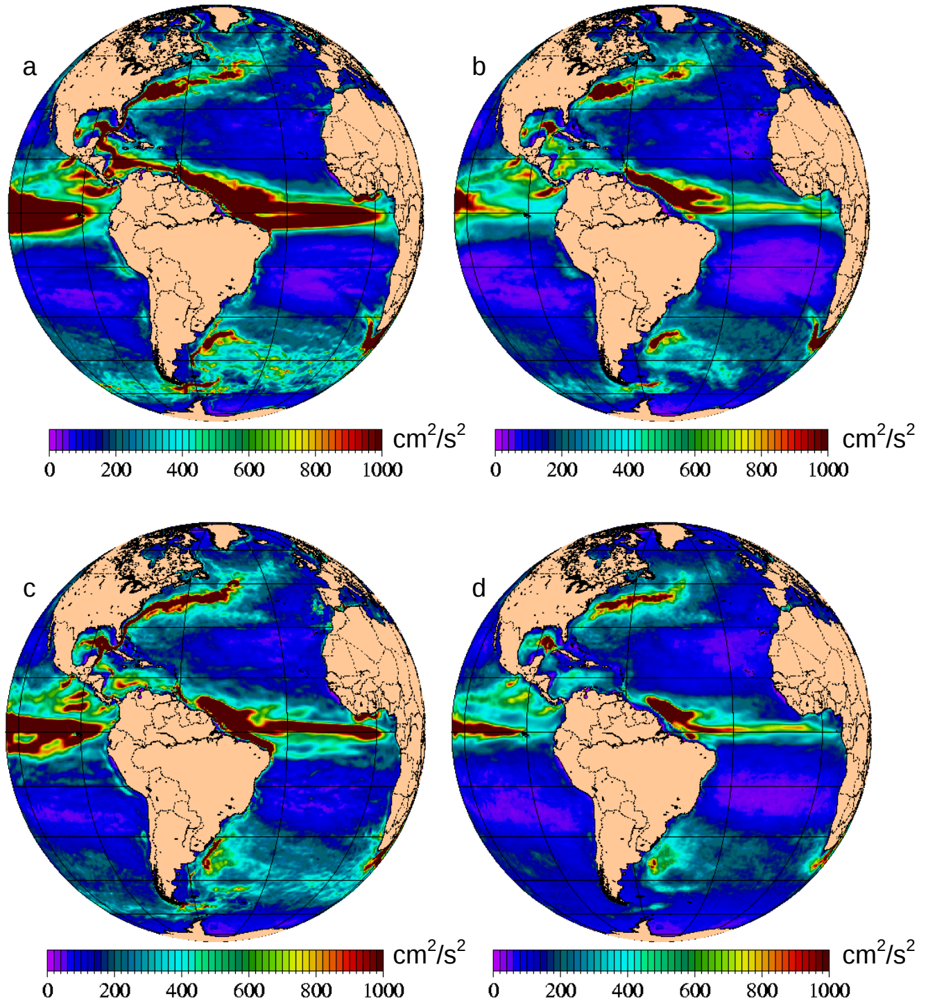
Fig. 9 – Atlantic hemispheric view of mean 1998-2000 surface kinetic energy (left; a,c) and surface EKE (right; b,d) for free-running (top; a,b) and assimilative (bottom; c,d) 1/8^\circ global NCOM. NCOM is forced with NOGAPS wind and thermal fluxes. The assimilative case relaxes to MODAS synthetic temperature and salinity derived from 1/8^\circ MODAS2D SST and 1/16^\circ NLOM SSH.
