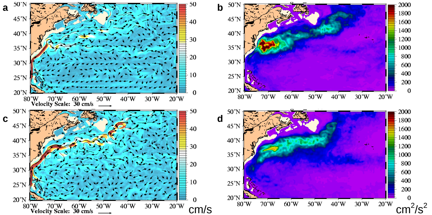
Fig. 21 – Gulf Stream zoom of mean 1998-2000 100m speed with superimposed currents (left;a,c) and 100m EKE (right;b,d) for free-running (top;a,b) and assimilative (bottom;c,d) 1/8° global NCOM.
