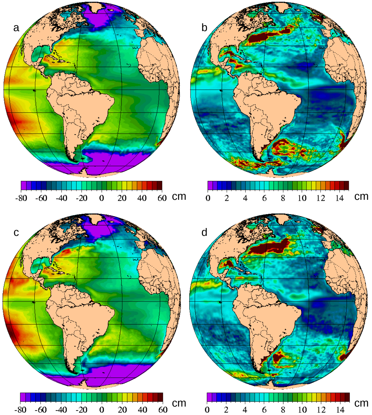
Fig. 5 – Atlantic hemispheric view of mean 1998-2000 SSH (left; a, c) and SSH standard deviation (right; b, d) for free-running (top; a, b) and assimilative (bottom; c, d) 1/8^\circ global NCOM. NCOM is forced with NOGAPS wind and thermal fluxes. The assimilative case relaxes to MODAS synthetic temperature and salinity derived from 1/8^\circ MODAS2D SST and 1/16^\circ NLOM SSH and the statistics of the historical hydrographic data base.
