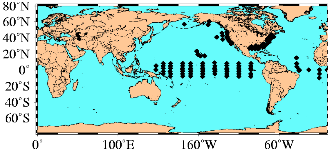
Fig. 47 – Locations of TAO, PIRATA and NDBC buoys providing 219 unassimilated, year-long buoy temperature profiles used for validation of NCOM SST 1998-2000.
