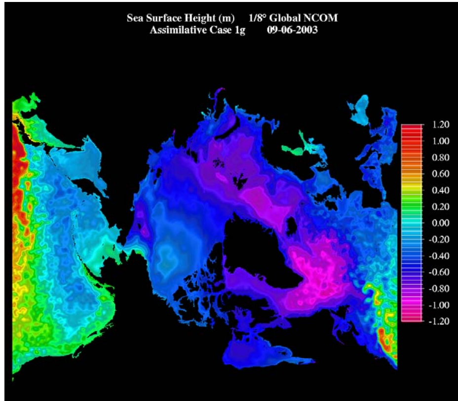
Fig. 3 – Snapshot of Arctic sea surface height. The plot is a rectangular dump of this portion of the domain and indicates the relative grid distortion of various Arctic features. Distortion is greatest in areas near the singularities, such as Hudson Bay.
