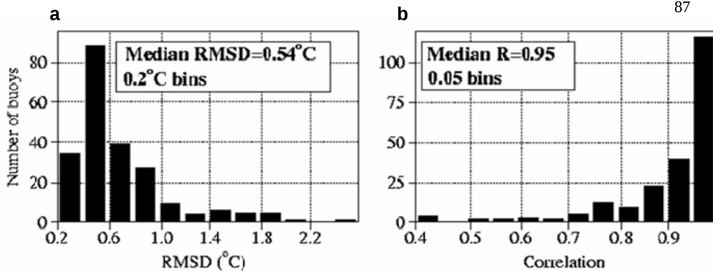
Fig. 50 – Histograms of (a) root-mean-squared difference and (b) correlation between buoy observed and assimilative 1/8° global NCOM SST over 219 unassimilated year-long time series over 1998-2000.
