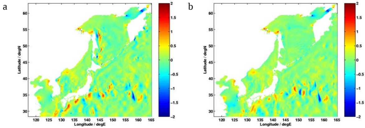
Fig. 104 – Meridional surface velocity (m/s) from the SWAFS pacnest restart files valid 19 July 2003 from the run using SWAFS northworld boundary conditions (a) and NCOM/OSU boundary conditions (b).
