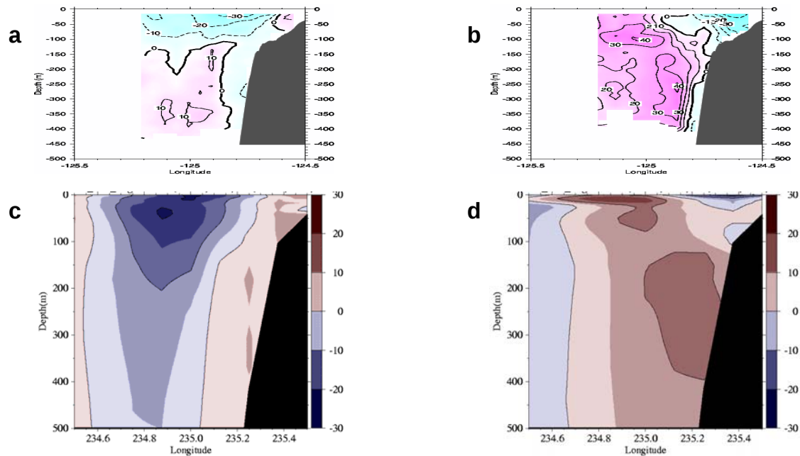
Fig. 94 – Comparisons of northward velocity (cm/s) through a sections near the Rogue River, Oregon. Sections from (a,b) ADCP surveys conducted as a part of the Northeast Pacific Long Term Observation Program and (c,d) snapshots from the assimilative 1/8^\circ global NCOM. The (a) 15-16 Apr. 2000 observations and (c) 16 Apr. 2000 NCOM snapshot both show northward flow in the upper 100m but opposite flow at depth. Agreement is close between the (b) 13-14 July 2002 survey and (d) 14 July 2002 model results, although the model structure shows less detail and lower extrema.
