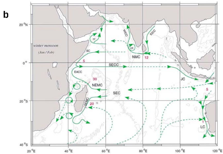
Fig. 9. As in Fig. 8, but for the Northeast Monsoon.
