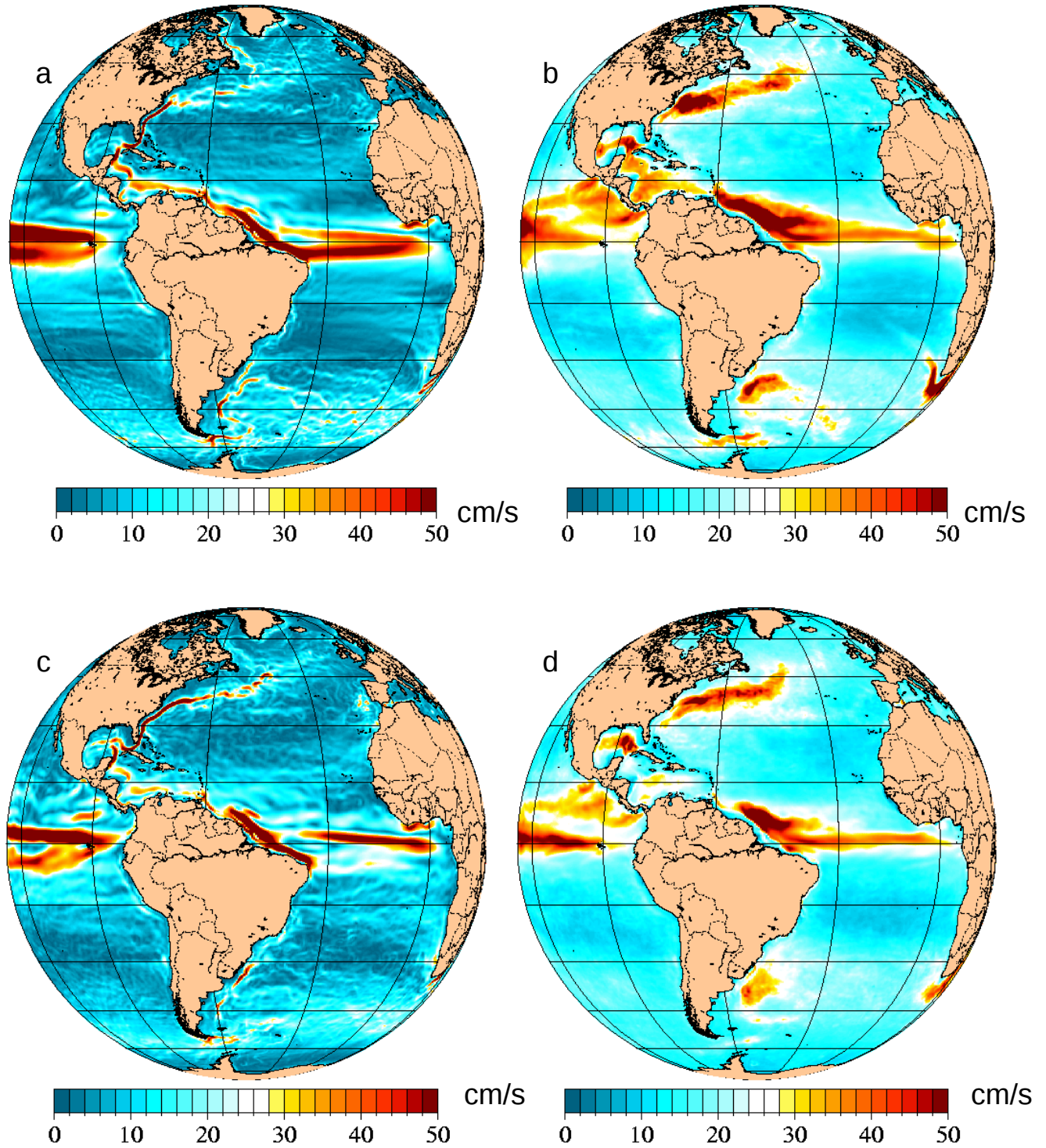
Fig. 8 – Atlantic hemispheric view of mean 1998-2000 surface speed (left; a,c) and surface speed standard deviation (right; b,d) for free-running (top; a,b) and assimilative (bottom; c,d) 1/8^\circ global NCOM. NCOM is forced with NOGAPS wind and thermal fluxes. The assimilative case relaxes to MODAS synthetic temperature and salinity derived from 1/8^\circ MODAS2D SST and 1/16^\circ NLOM SSH.
