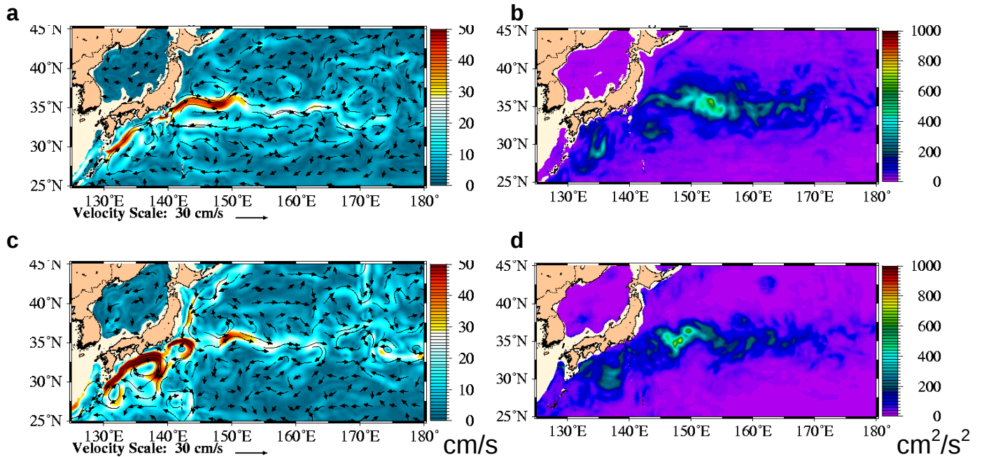
Fig. 32 – Kuroshio zoom of mean 500m speed with superimposed currents (left;a,c) and 500m EKE (right;b,d) for assimilative 1/8° global NCOM (top;a,b) and assimilative 1/4° SWAFS Northworld (bottom; c,d). Mean is over period of available SWAFS subsurface data, 11/15/2002 – 5/15/2003.
