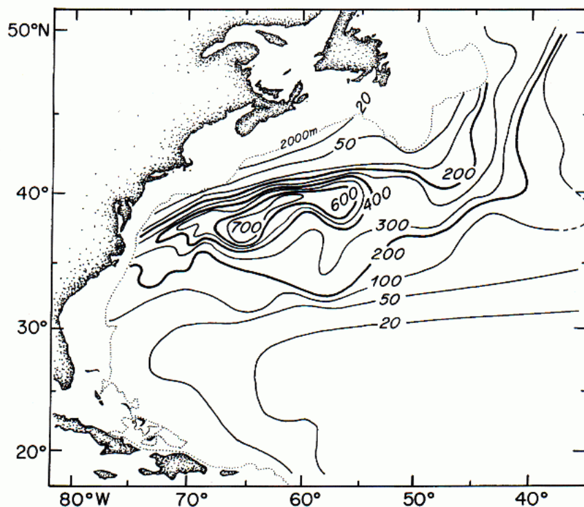
Fig. 25 – Climatological EKE near 700m depth in the western North Atlantic. Taken from Schmitz (1996) which adapted the data from Owens (1984,1991) and Richardson (1993).
