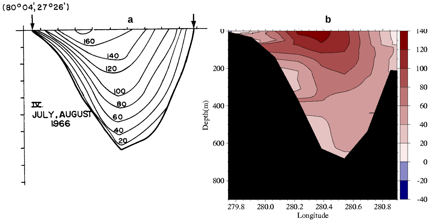
Fig. 67 – Comparison of mean currents through Florida Current section IV. (a) downstream speed contours from Schmitz (1996) with observations from July-August 1966 and (b) northward speed contours from assimilative 1/8° global NCOM 1998-2000 mean section at 27.43°N, 80.25°W-79.1°W.
