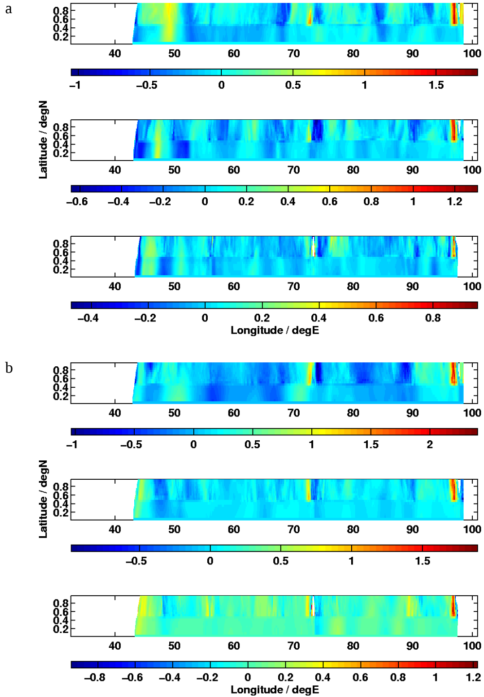
Fig. 120 – Meridional velocity (m/s) along the southern boundary of the SWAFS ionest domain restart files valid 07 Dec 2003 using the northworld (a) and NCOM/OSU (b) boundary conditions, each at 0 (top), 200 (middle), 1000 (bottom) m.
