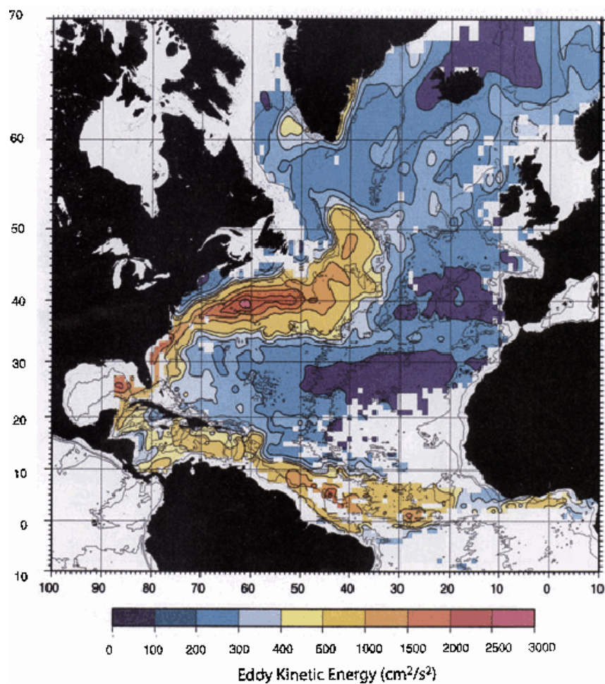
Fig. 23 – North Atlantic surface EKE calculated using Lagrangian velocities derived from satellite drifter observations during the 1990s. Taken from Fratantoni (2001).
