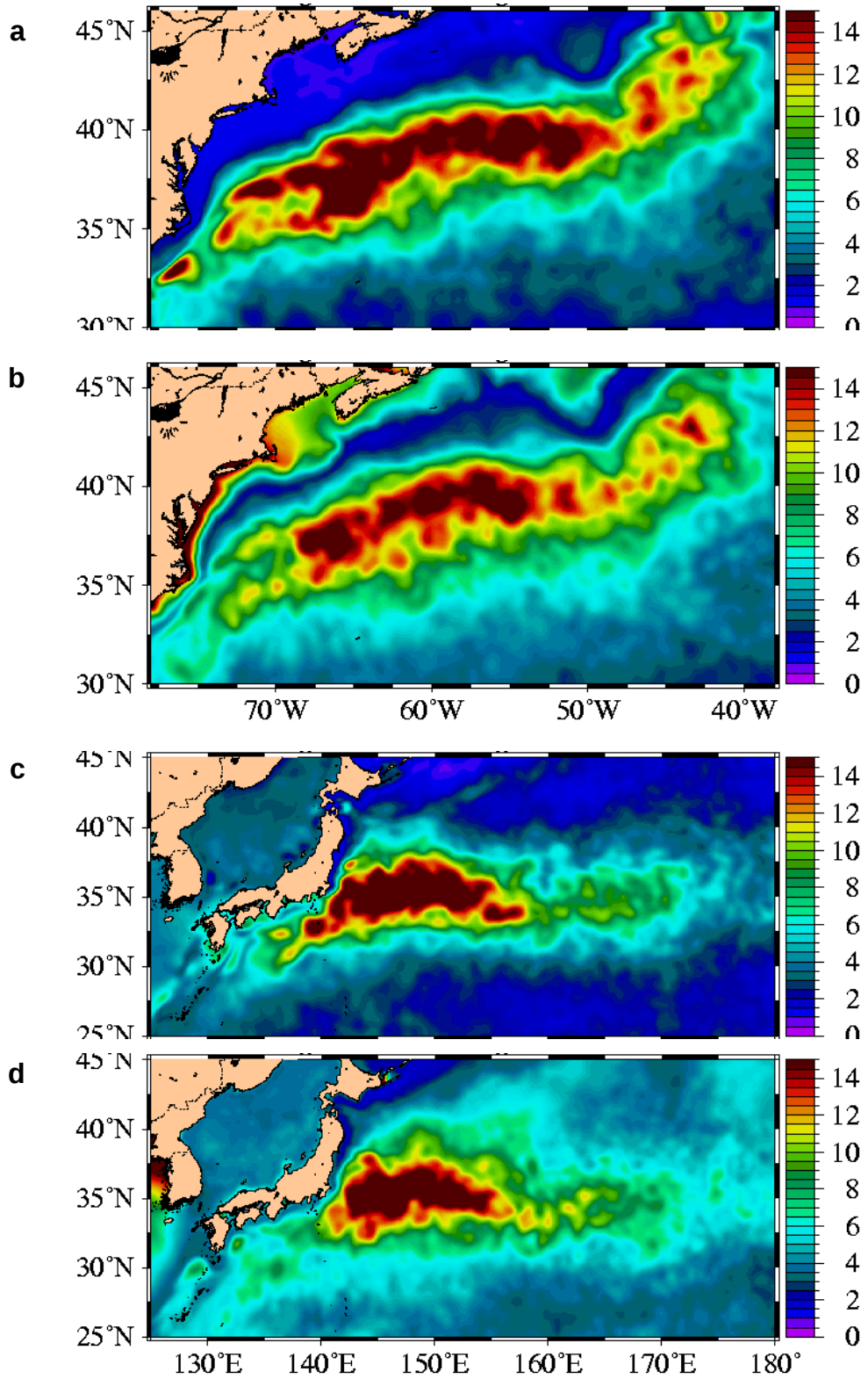
Fig. 82 – Mean 7-day 1/8^\circ global NCOM (a,c) forecast and (b,d) persistence error in SSH (cm) relative to subsequent global NCOM nowcasts for forecasts from 1998-2002 in the (a,b) Gulf Stream and (c,d) Kuroshio regions. Relative forecast errors are particularly good on the continental shelves. Relative forecast skill is lower along the main fronts, reflecting the free-running difficulty in representing these frontal dynamics at 1/8^\circ resolution.
