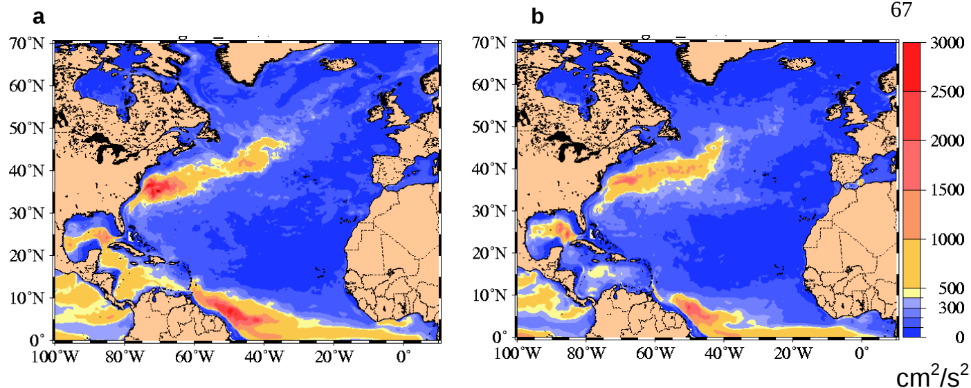
Fig. 22 – North Atlantic zoom of mean 1998-2000 5m EKE for free-running (a) and assimilative (b) 1/8° global NCOM. While similar to the assimilative case in most respects, the free-running case in the Caribbean Sea and north of 60°N has higher surface EKE, in better agreement with observations (below).
