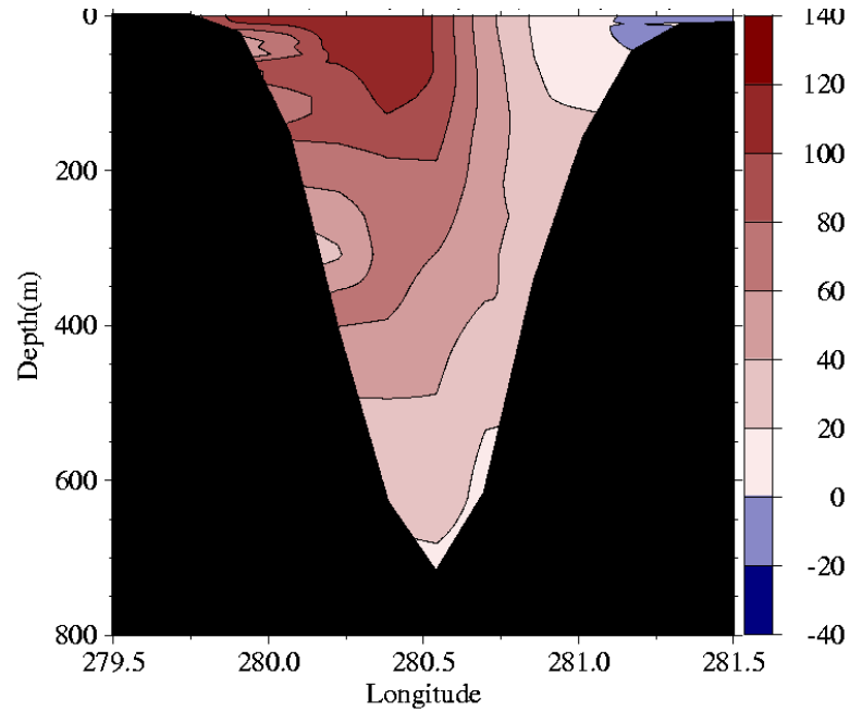
Fig. 66 – Mean currents through Florida Current at 27°N, 80.5°W-78.5°W from assimilative 1/8° global NCOM 1998-2000.
