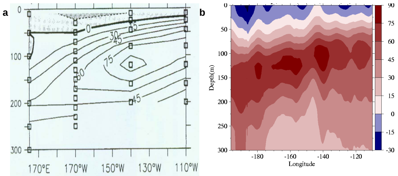
Fig. 76 – Velocity section along the equator ( 0^{\circ}\text{N} ) between 165^{\circ}\text{E} and 110^{\circ}\text{W} . (a) Contours of eastward speed derived from 1991-1999 shipboard observations (Yu and McPhaden, 1999) and (b) contours of eastward speed from assimilative 1/8^{\circ} global NCOM 1998-2000 mean.
