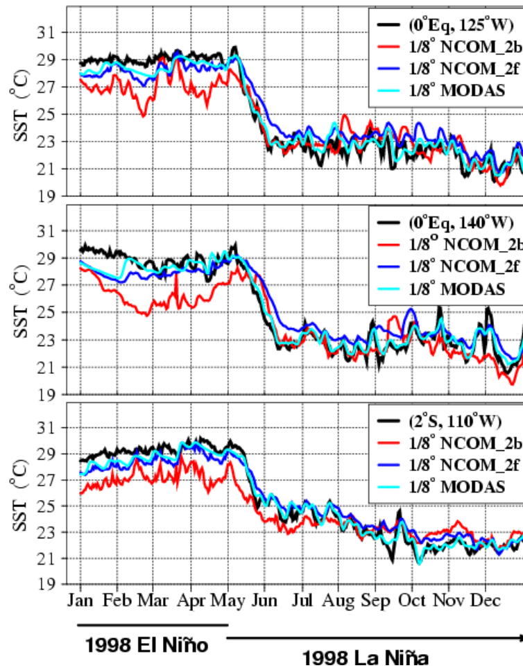
Fig. 48 – Comparison between observed (black), free-running NCOM (red), assimilative NCOM (blue) and MODAS analyses (SST) at three TAO equatorial Pacific stations during the 1998 El Niño to La Niña transition.
