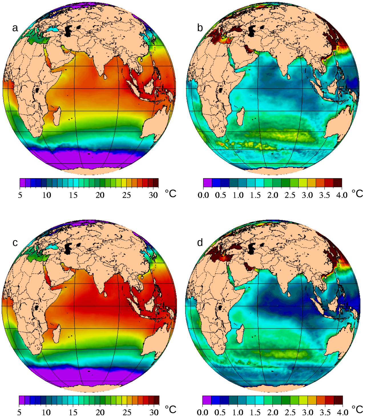
Fig. 11 – Indian hemispheric view of mean 1998-2000 SST (left;a,c) and SST standard deviation (right;b,d) for free-running (top;a,b) and assimilative (bottom;c,d) 1/8° global NCOM. NCOM is forced with NOGAPS wind and thermal forcing. The assimilative case relaxes to MODAS synthetic temperature and salinity derived from 1/8° MODAS2D SST and 1/16° NLOM SSH.
