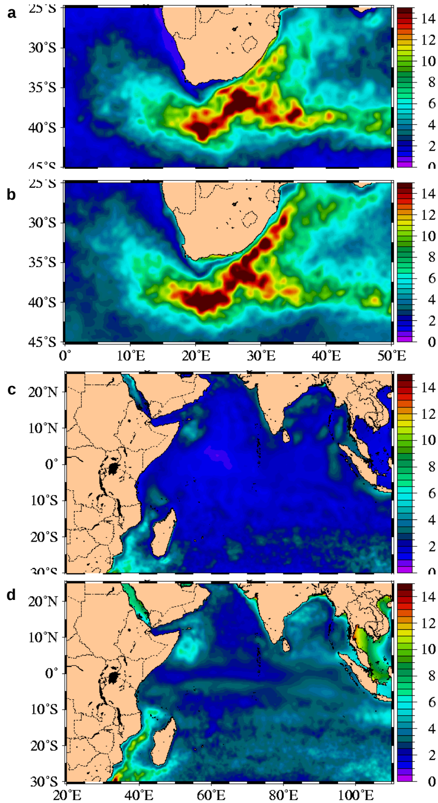
Fig. 83 – Mean 7-day 1/8° global NCOM (a,c) forecast and (b,d) persistence error in SSH (cm) relative to subsequent global NCOM nowcasts for forecasts from 1998-2002 in the (a,b) Agulhas and (c,d) Indian Ocean regions. Relative forecast errors are generally low and better than persistence. Skill is lower in the Agulhas Retroflection, reflecting the free-running difficulty in representing these frontal dynamics at 1/8° resolution.
