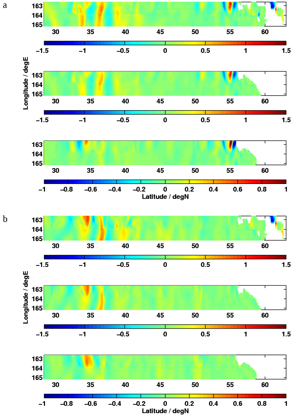
Fig. 108 – Zonal velocity (m/s) along the eastern boundary of the SWAFS pacnest domain restart files valid 17 July 2003 using the northworld (a) and NCOM/OSU (b) boundary conditions, each at 0 (top), 200 (middle), 1000 (bottom) m.
