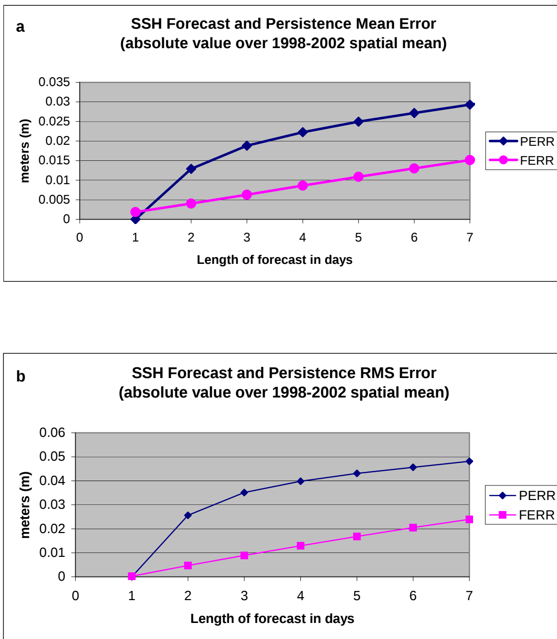
Fig. 80 – SSH forecast and persistence error comparisons versus forecast length up to seven days for 1/8° global NCOM. Calculated from bimonthly 7-day forecasts from 1998-2002. (a) mean absolute error in SSH and (b) square root of mean squared error in SSH. Means are calculated in space over the global ocean and in time over 1998-2002. Error is relative to the NCOM analysis valid on zero hours of each forecasted day. Forecast error is consistently smaller than persistence. The forecast is particularly better in shallow water.
