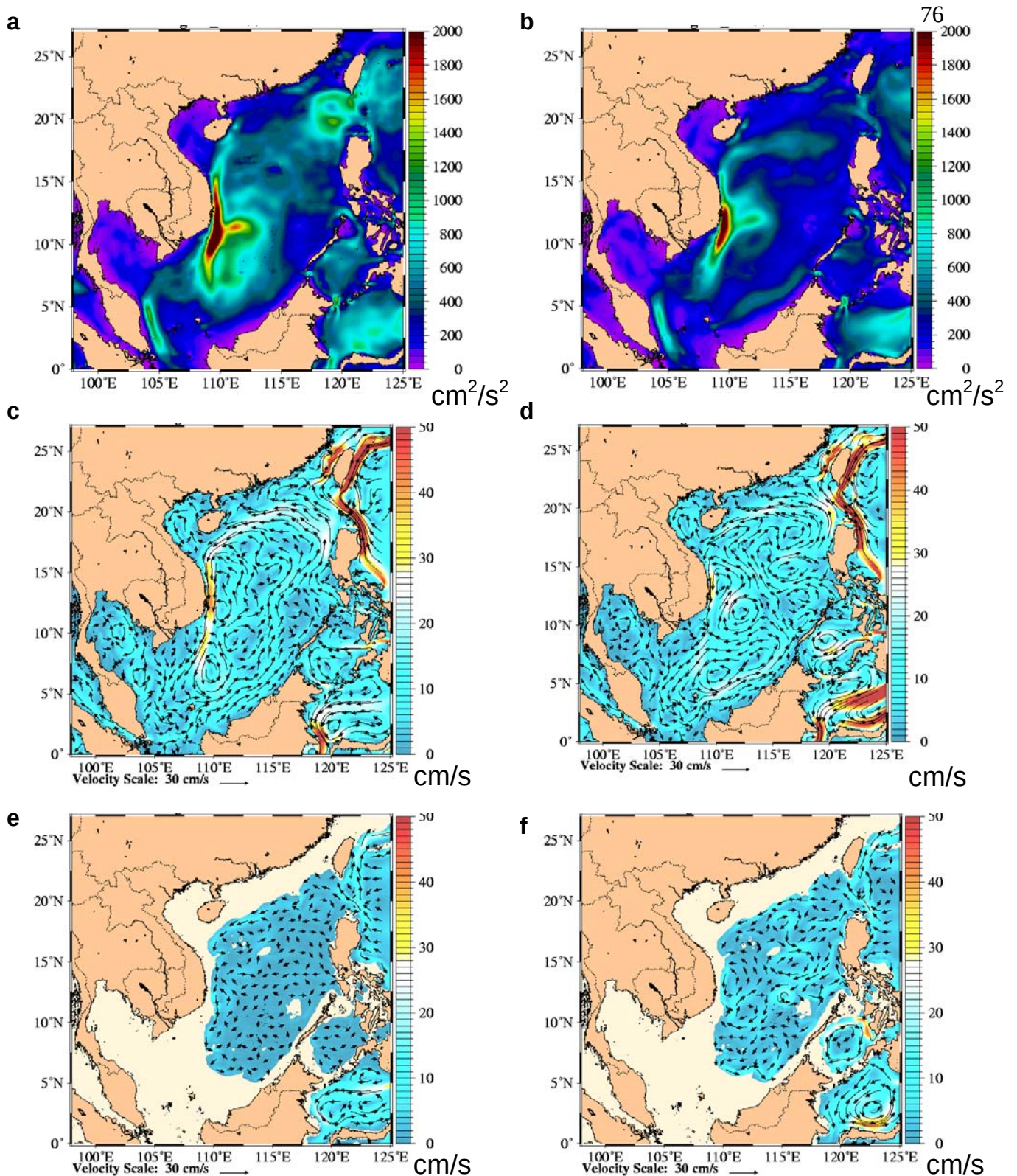
Fig. 38 – South China Sea zoom of mean 1998-2000 surface EKE (a,b) and surface (c,d) and 500m (e,f) speed with superimposed currents for free-running (left;a,c,e) and assimilative (right;b,d,f) 1/8° global NCOM. Assimilation reduces surface EKE south of Taiwan and increases surface current penetration into the Suluwesi Sea. At 500m, assimilation introduces anticyclonic circulation in the Sulu Sea and strengthens cyclonic circulation in the Suluwesi Sea.
