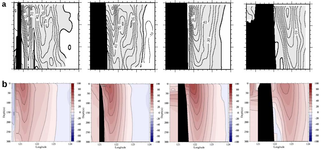
Fig. 73 – Four velocity sections across the upper 300m east of Taiwan, 120°30'E-124°00'E, at 22°N, 23°N, 24°N and 25°N. (a) contours of northward speed from ADCP observations from (Liang et al. , 2003) and (b) contours of northward speed from assimilative 1/8° global NCOM 1998-2000 mean.
