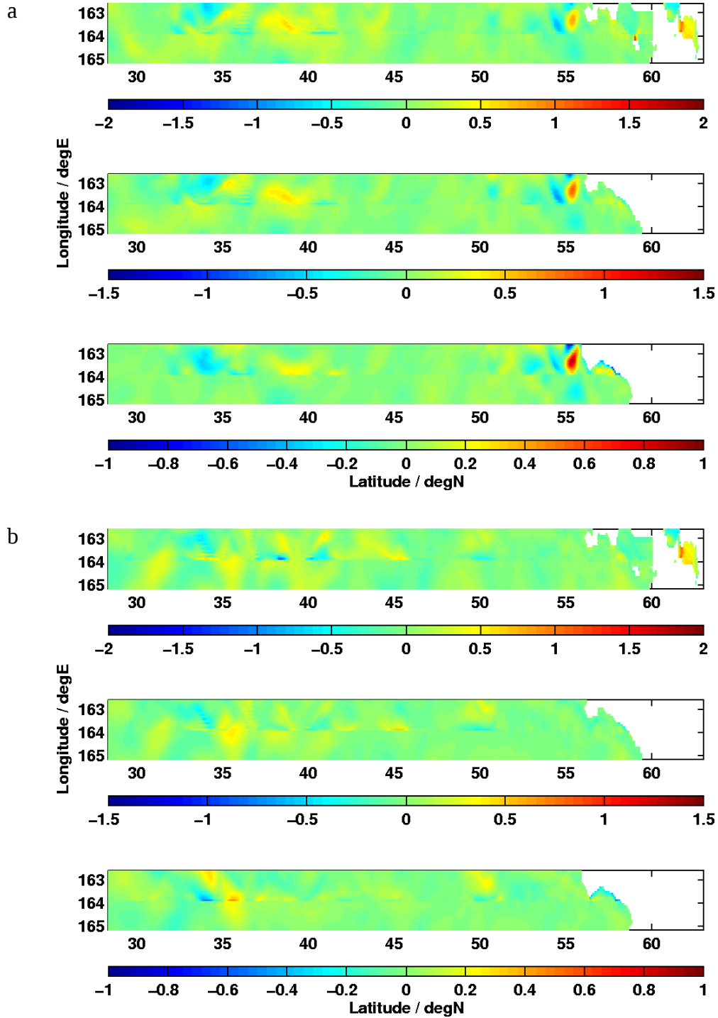
Fig. 109 – Meridional velocity (m/s) along the eastern boundary of the SWAFS pacnest domain restart files valid 17 July 2003 using the northworld (a) and NCOM/OSU (b) boundary conditions, each at 0 (top), 200 (middle), 1000 (bottom) m.
