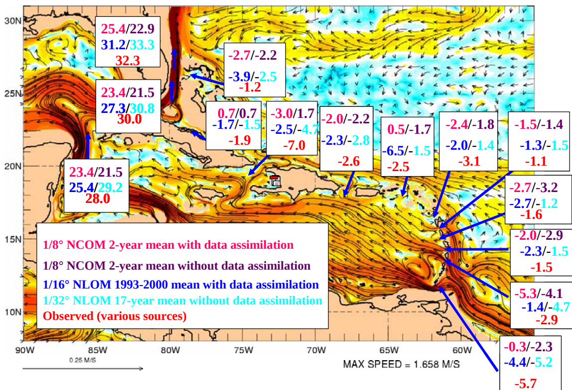
Fig. 79 – Annual mean Caribbean and Bahamas passage transports from the 1/8 ° NCOM, 1/16 ° (blue) and 1/32 ° (cyan) global NLOM compared to observations. Background plot shows the 1/32 ° NLOM annual mean upper layer current vectors superimposed on their strength (log of the kinetic energy of the mean flow) in color. Major currents are indicated relatively long vectors that are collocated with areas of high kinetic energy (red and yellow).
