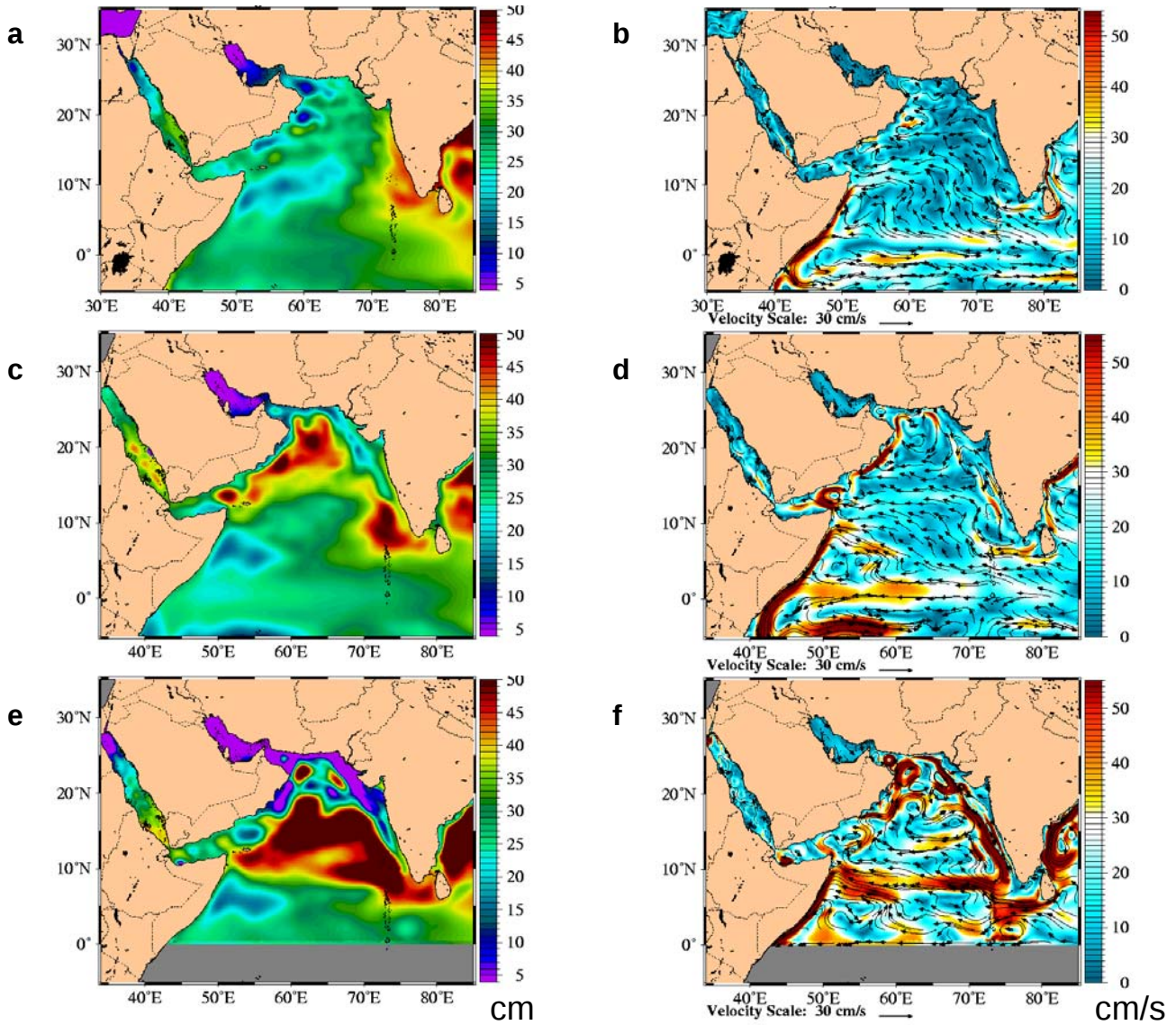
Fig. 36 – Arabian Sea zoom of SSH (left; a,c,e) and speed with superimposed currents (right; b,d,f) for assimilative 1/8° global NCOM (a,b), 1/4° SWAFS Northworld (c,d) and SWAFS IO nest (e,f). Mean is over winter monsoon period, 11/15/2002 – 3/15/2003. SSH mean is offset in SWAFS to equal NCOM SSH mean over the plot area.
