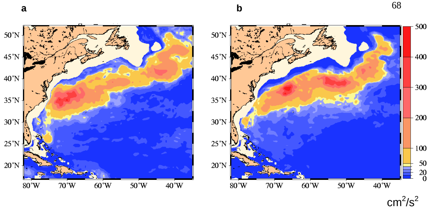
Fig. 24 – Gulf Stream zoom of mean 1998-2000 EKE at 700m from free-running (a) and assimilative (b) 1/8^\circ global NCOM. In comparison to the free-running case, EKE at 700m in the assimilative case is generally higher and in closer agreement to historical observations (below), showing the two regions of relatively high EKE south of Nova Scotia and Newfoundland.
