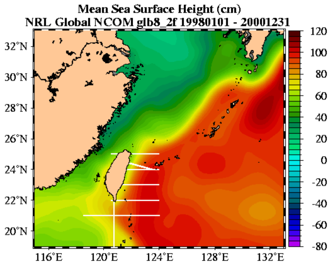
Fig. 70 – Global NCOM 1998-2000 SSH mean in the Taiwan area. Superimposed white lines locate vertical sections extracted from NCOM for comparison with sections of mean currents from historical observations.
