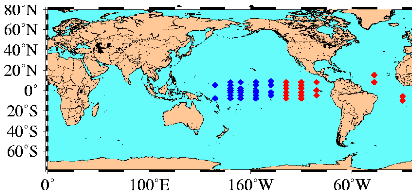
Fig. 55 – Locations of buoys providing 95 unassimilated, year-long time series of buoy temperature profiles used for validation of NCOM temperature profiles for 1998-2001. Stations are of two types, distinguished by the set of standard depths for placement of temperature measurements. Type I is shown in red; type II is shown in blue.
