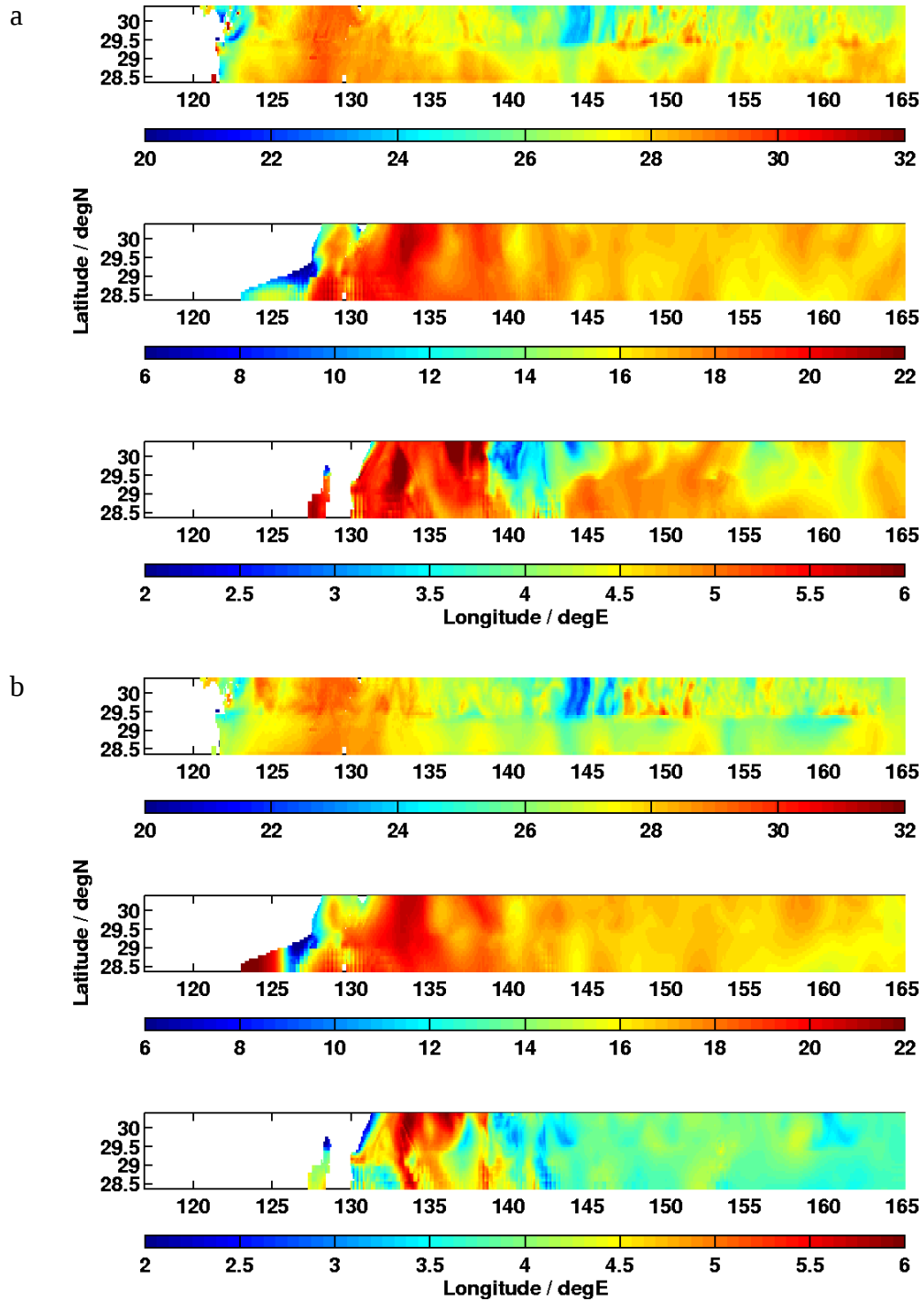
Fig. 107 – Temperature ( ^{\circ}\text{C} ) along the southern boundary of the SWAFS pacnest domain restart files valid 17 July 2003 using the northworld (a) and NCOM/OSU (b) boundary conditions, each at 0 (top), 200 (middle), 1000 (bottom) m.
