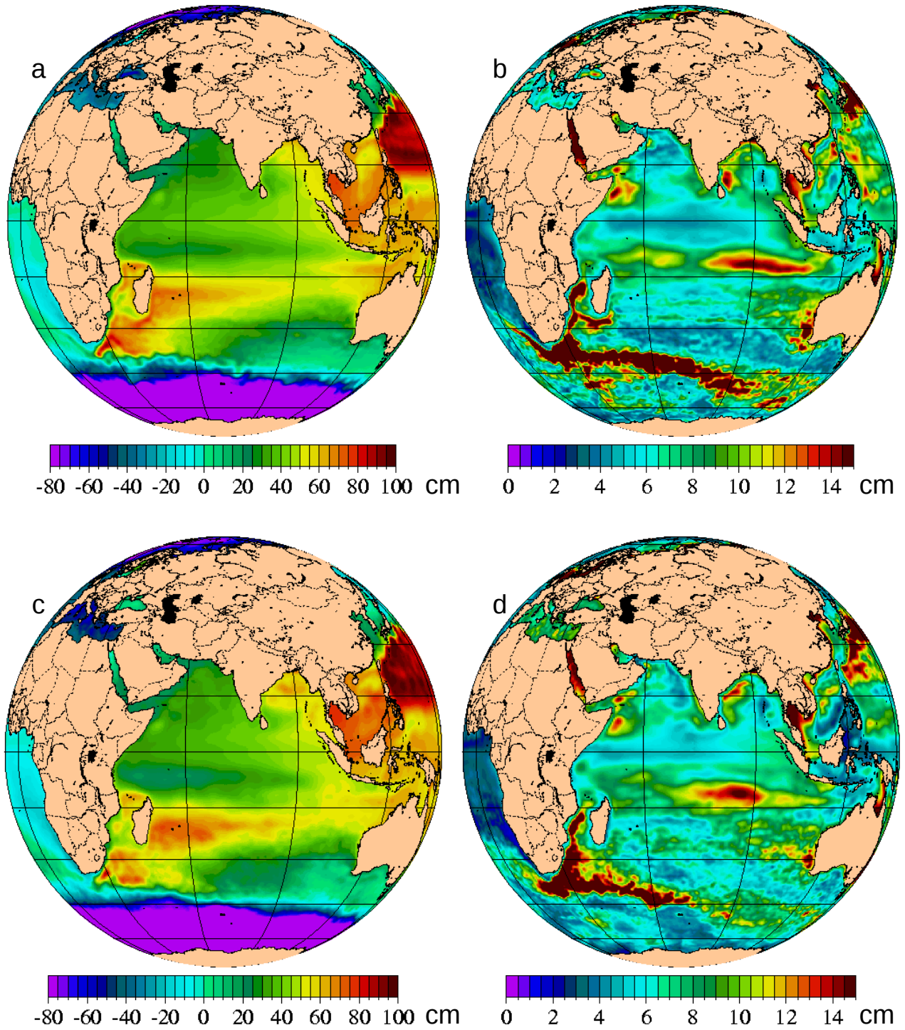
Fig. 10 – Indian hemispheric view of mean 1998-2000 SSH (left; a, c) and SSH standard deviation (right; b, d) for free-running (top; a, b) and assimilative (bottom; c, d) 1/8° global NCOM. NCOM is forced with NOGAPS wind and thermal forcing. The assimilative case relaxes to MODAS synthetic temperature and salinity derived from 1/8° MODAS2D SST and 1/16° NLOM SSH.
