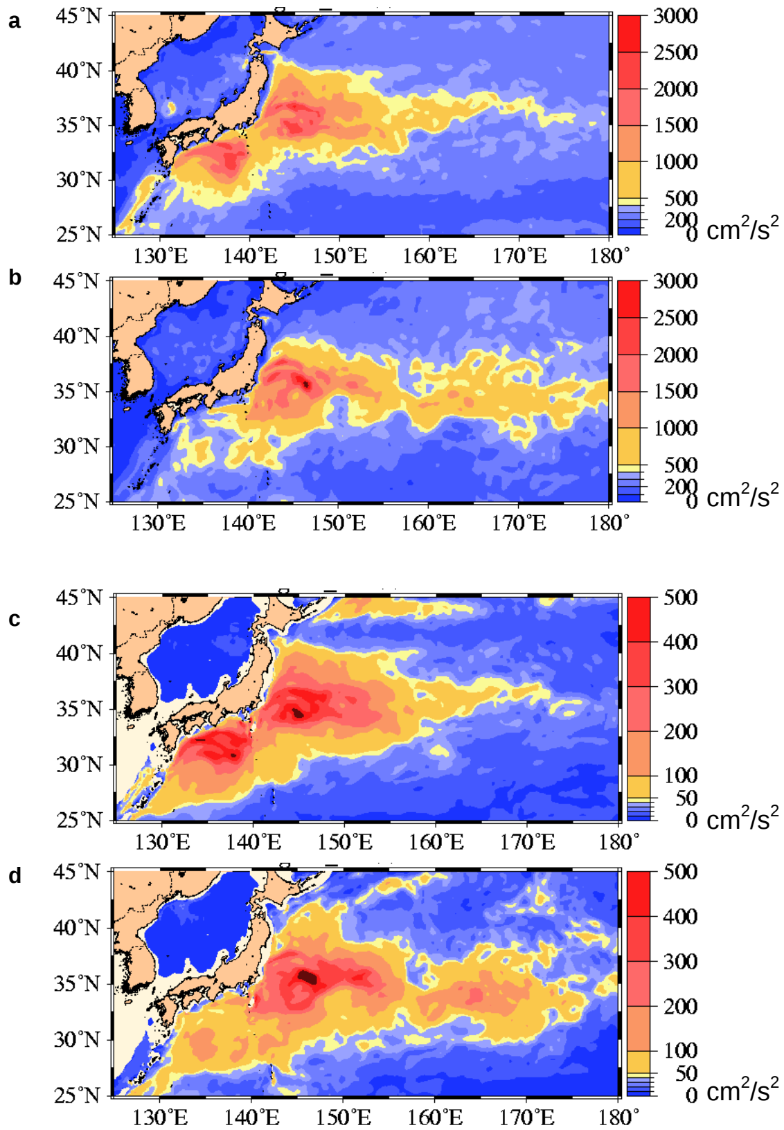
Fig. 30 – Kuroshio zoom of mean 1998-2000 EKE at 5m (a,b) and 500m (c,d) from free-running (a,c) and assimilative (b,d) 1/8° global NCOM. Assimilation produces a more realistic eastward extension of the Kuroshio and more tightly constrains the current east of 140°E.
