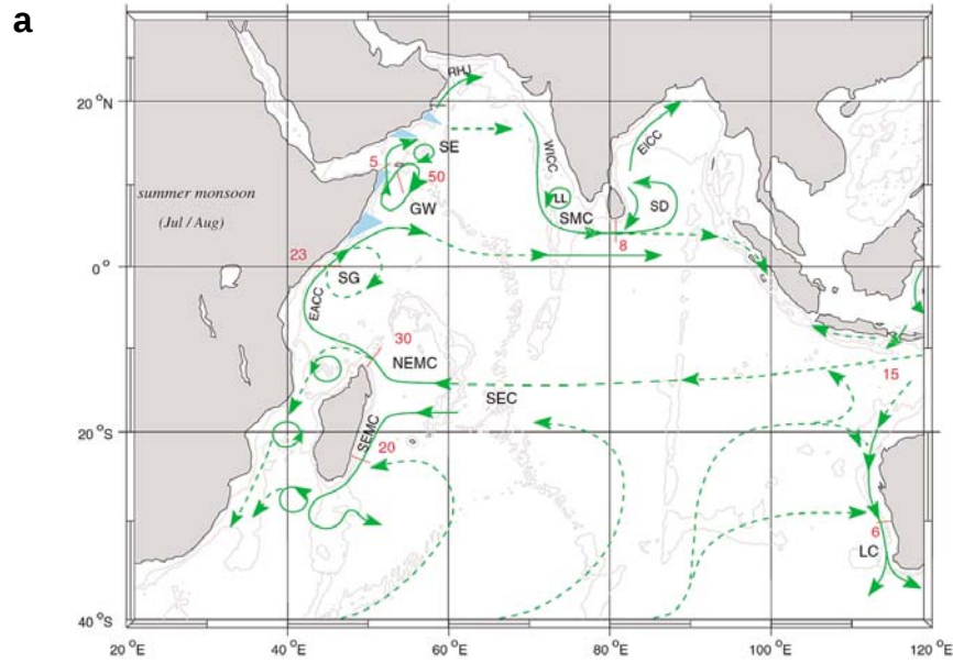
Fig. 8. A schematic representation of identified current branches during the Southwest Monsoon, including some choke point transport numbers ( Sv=10^6 m^3 s^{-1} ). Current branches indicated (see also Fig. 9) are the South Equatorial Current (SEC), South Equatorial Countercurrent (SECC), Northeast and Southeast Madagascar Current (NEMC and SEMC), East African Coast Current (EACC), Somali Current (SC), Southern Gyre (SG) and Great Whirl (GW) and associated upwelling wedges, Socotra Eddy (SE), Ras al Hadd Jet (RHJ) and upwelling wedges off Oman, West Indian Coast Current (WICC), Laccadive High and Low (LH and LL), East Indian Coast Current (EICC), Southwest and Northeast Monsoon Current (SMC and NMC), South Java Current (JC) and Leeuwin Current (LC). See text for details.
