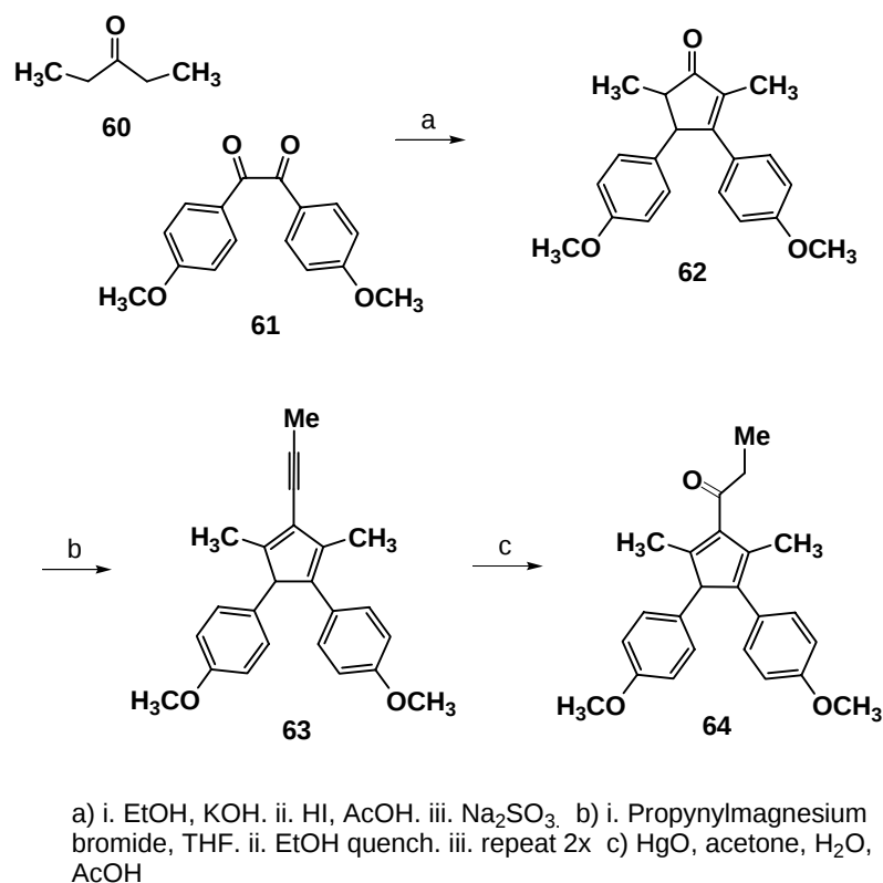
Scheme 19 Model Hydration System
