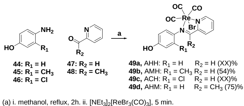
Scheme 13 Synthesis of Monohydroxy Imines
