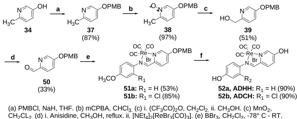
Scheme 14 Synthesis of Bis-Hydroxy Imines
