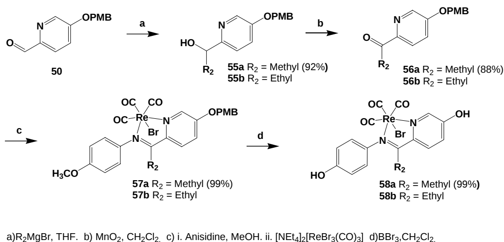
Scheme 16 Synthesis of Keto-imine Complexes
