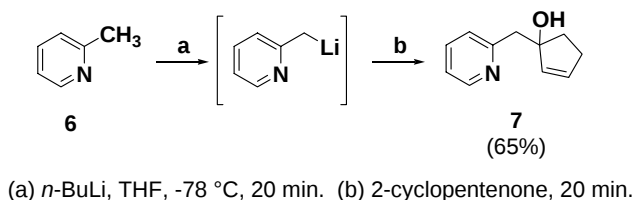
Scheme 2 Anionic Synthesis of Core
