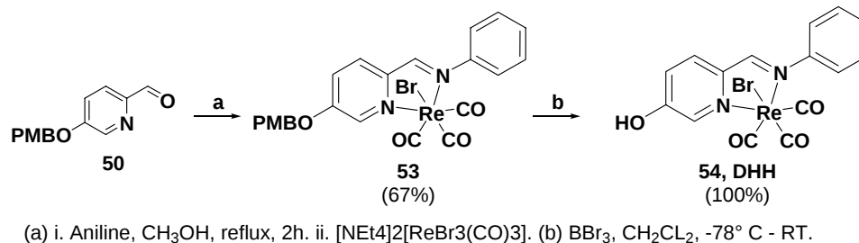
Scheme 15 Synthesis of Isomeric Monohydroxy Imine
