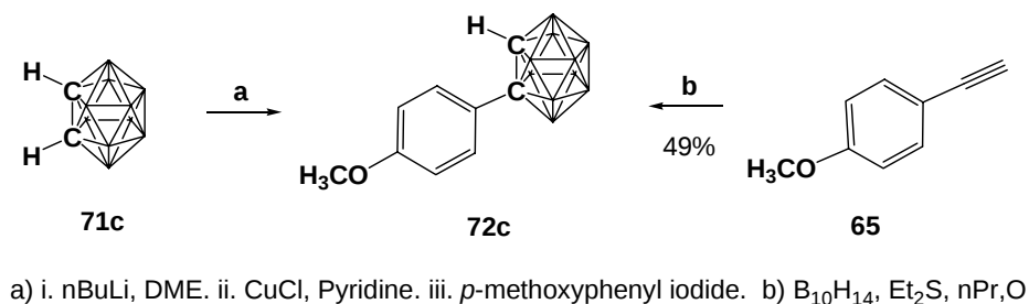
Scheme 22 Synthesis of Mono Aryl Carborane
