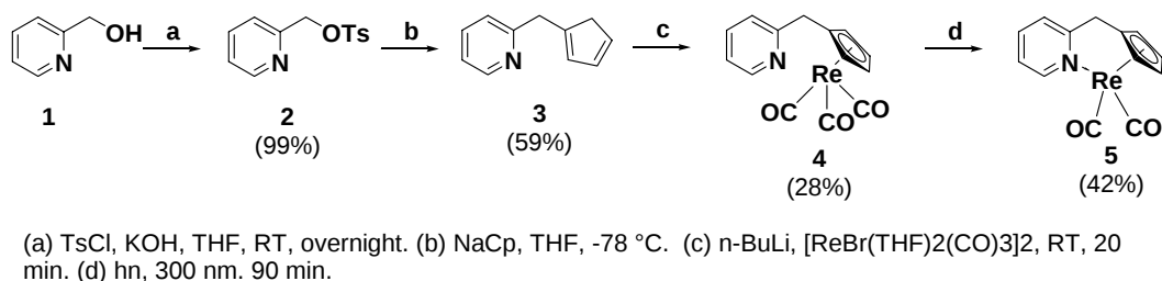
Scheme 1 Synthesis of Pyridyl-Cyclopentadienyl Core
