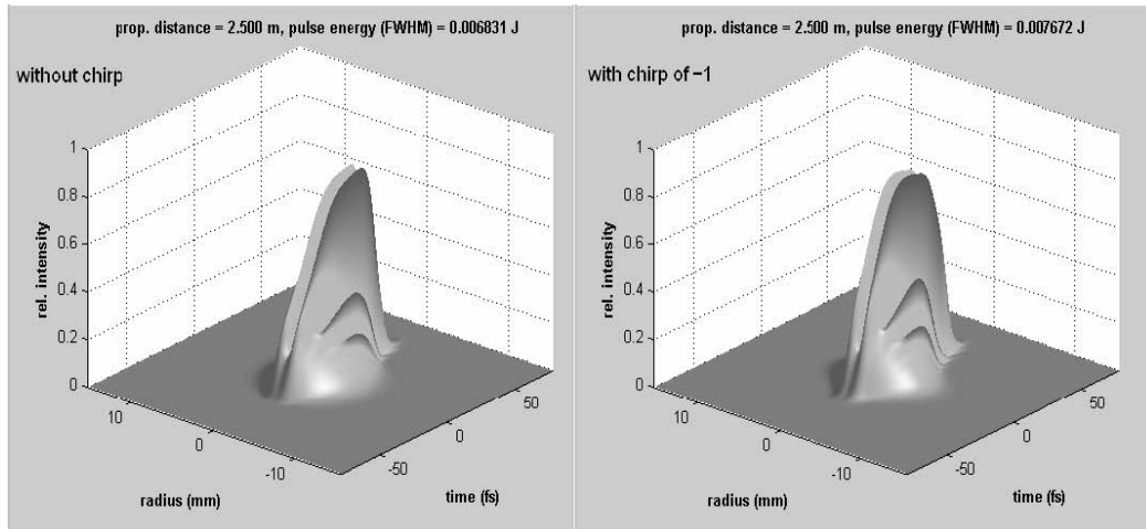
Figure 56: pulse at 2.5 m. (a) without and (b) with chirp of -1.0
