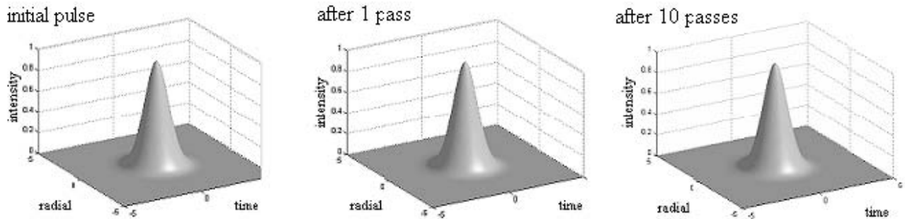
Figure 5: test result for IMSL FFT
