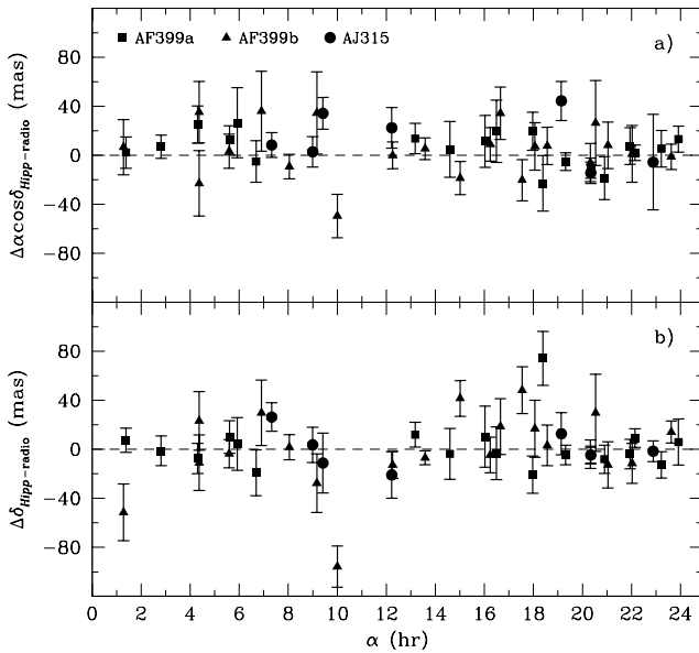
FIG. 2.— Differences between the Hipparcos positions updated to the epoch of our observations and our VLA+PT measured positions as a function of source right ascension \alpha for the 46 radio stars observed. Differences in \alpha \cos \delta are plotted in (a), and differences in \delta are plotted in (b). Error bars are the rss combined uncertainties listed in Table 3.
