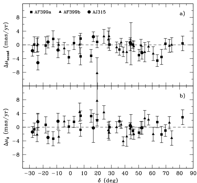
FIG. 5.—Differences between the Hipparcos proper motions and our radio-derived proper motions as a function of source declination \delta for the 46 radio stars observed. Differences in \mu_{\alpha \cos \delta} are plotted in (a), and differences in \mu_{\delta} are plotted in (b). Error bars are the rss combined uncertainties listed in Table 5.
