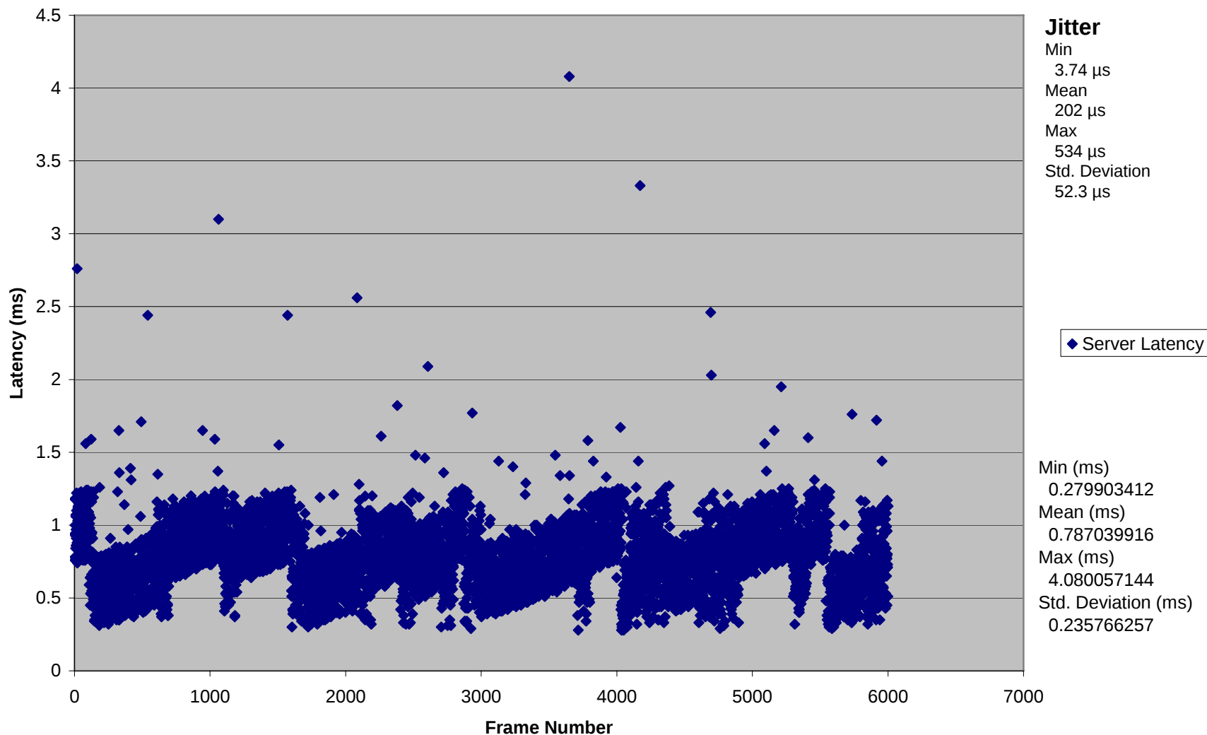
Server Latency
