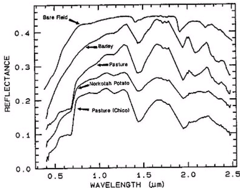
Figure 1: Spectral Signatures Constructed From AVIRIS Sensor
