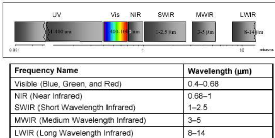
Figure 2 Wavelength Groupings for HSI Sensors
