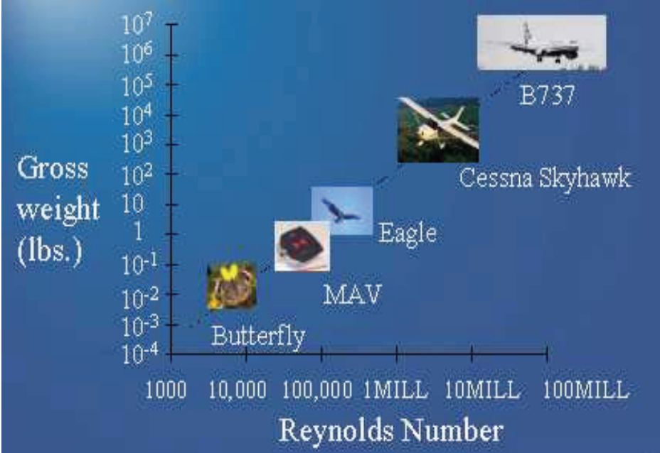
Figure 7.2 Reynolds Number 29
