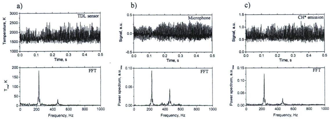
Fig. 15. Measured signals in a propane-air flame with FFT power spectra for: a) TDL sensor; b) microphone; c) CH* chemiluminescence.
