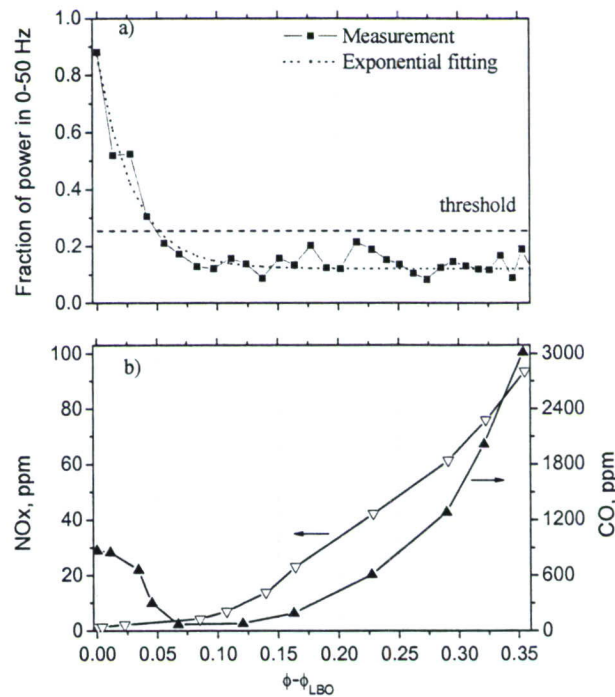
Fig. 24. a) Fraction of FFT power in 0-50 Hz of the TDL sensor output; b) extractive sampling of CO and NOx concentrations (dry-based) in the exhaust gas as a function of equivalence ratio for an air flow rate=25.7 SCFM.
