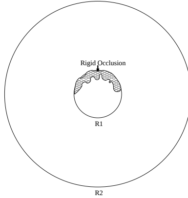
Figure 7: Geometry with occlusion along inner radius.
