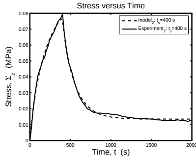
Figure 4: Stress calculation and comparative data for cartilage simulation with ramp strain.
