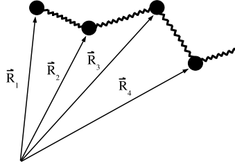
Figure 3: Representation of vectors for a bead-spring polymer molecule.
