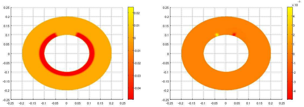
Figure 8: Results for v_1 (left) and v_2 (right) for the geometry with an occluded inner radius, t=0.0039 .
