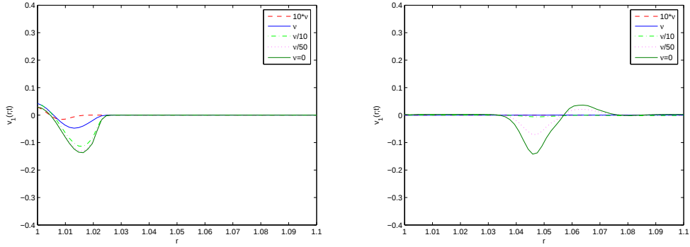
Figure 6: Results for v_1 for the varying values of the relaxation parameter, \nu at t=0.0032 (left) and t=0.0504 (right).
