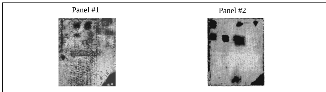
Figure 9: Through-transmission ultrasound images of Panels #1 and #2.
