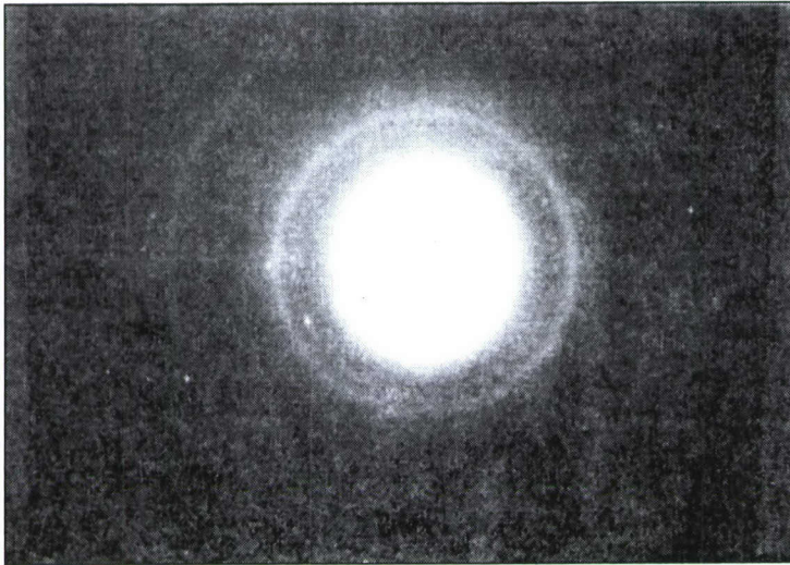
Fig. 7. Diffraction pattern for carbon attenuator film on beryllium oxide substrate. From Wachi, Ref. 5
