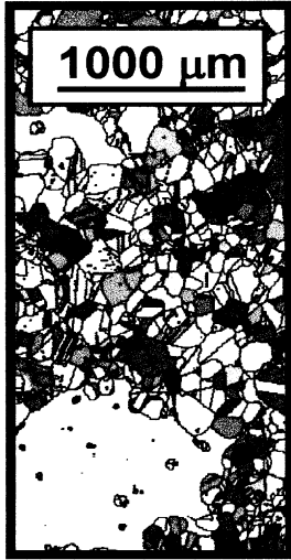
Fig. 10. Microstructure developed in a double-cone sample of Waspaloy ingot material upset to a 2:1 reduction at 1066^\circ\text{C} , 0.1 \text{ s}^{-1} and then held at temperature for 30 min. prior to water quenching. The FEM-predicted local strain for the region shown was 0.6.
