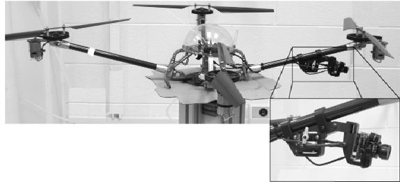
Figure 1: A ‘Draganflyer’ quad-rotor aircraft with an on-board pan-tilt camera.
