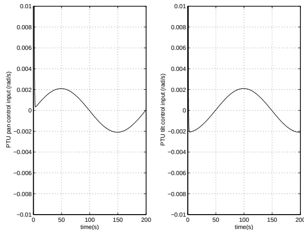
Figure 6: The PTCU angular velocity inputs on the lower UAV.
