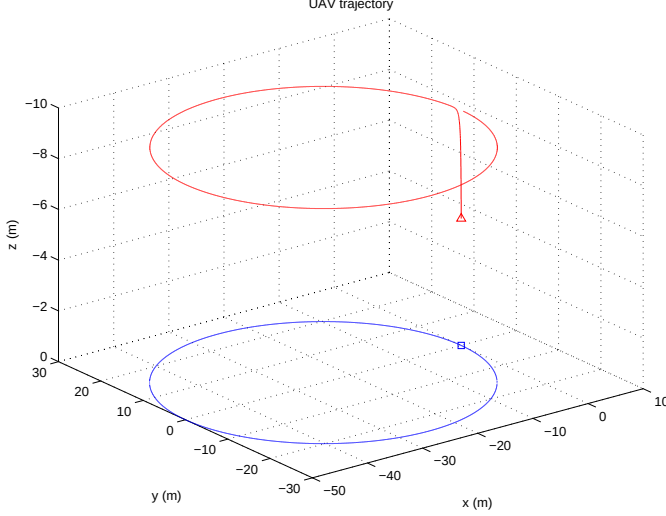
Figure 3: The leader ( \square ) and follower ( \triangle ) trajectories.
