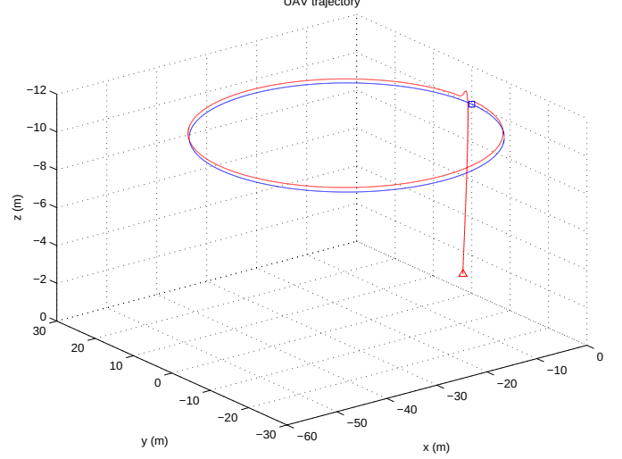
Figure 8: The desired ( \square ) and actual trajectories ( \triangle ).
