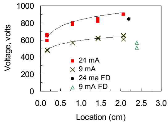
Figure 16. Discharge voltage versus cathode size where the size of the cathode is increasing from the leading edge of the model downstream.
