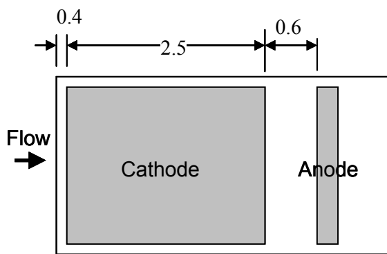
Figure 6. Drawings of different size electrodes where the cathode becomes bigger in the streamwise direction starting from the middle of the model getting bigger in the upstream direction.
