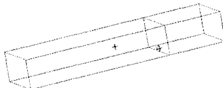
Figure 5. CFD-GEOM model of a single cell, modeled as a 10 \mu\text{m} diameter sphere, bound to the wall of a 50 \mu\text{m} \times 50 \mu\text{m} square channel. The channel inlet is to the left. About 57,000 elements are used to mesh the fluid; about 3,000 are used for the elastic sphere.
