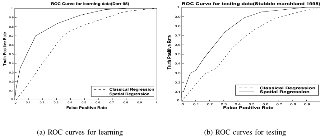
Fig. 3. (a) Comparison of the classical regression model with the spatial autoregression model on the Darr learning data. (b) Comparison of the models on the testing data.
