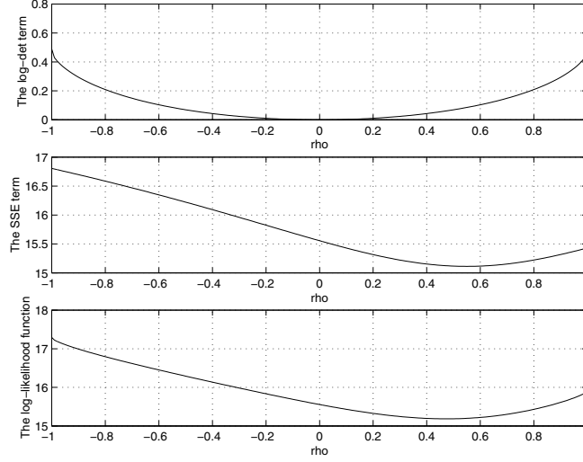
Fig. 7. The components of the log-likelihood function for a thematic class of satellite dataset with 2500 observation points and the log-likelihood function = log-det + SSE . "rho" stands for the SAR parameter \rho .
