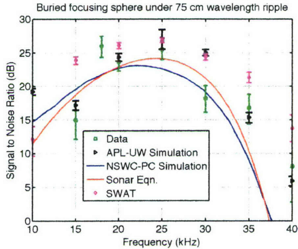
Figure 1. Subcritical angle detection of a buried sphere. The data are from a NSWC-PC test pool experiment. The NSWC-PC simulation (blue curve) and sonar equation (red curve) assume plane wave incidence. The finite range to the target in the experiment allows more penetration than these plane wave models predict and is taken into account in the APL-UW simulation and in the Navy applied simulation code SWAT.
