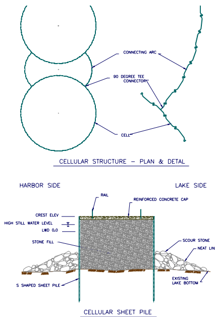
Figure 7a. Cellular sheet pile.
