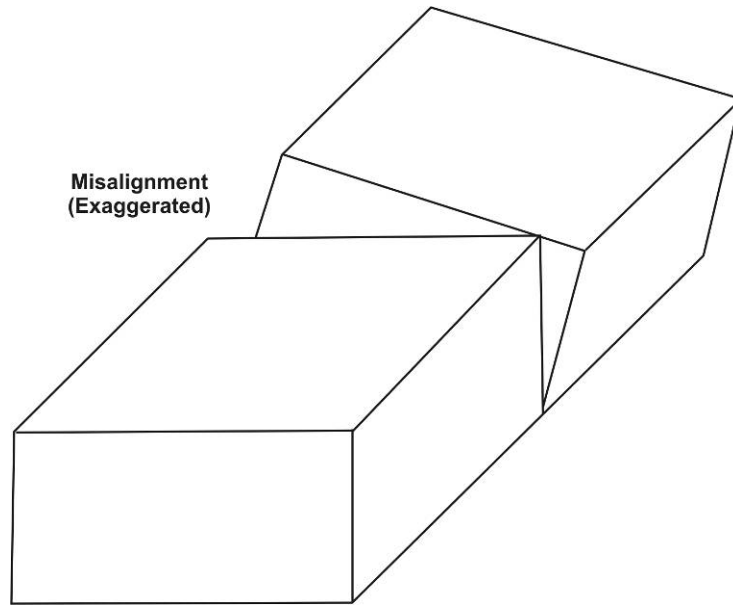
Figure 17. Misalignment caused by settlement, external loads, or a combination of both.
