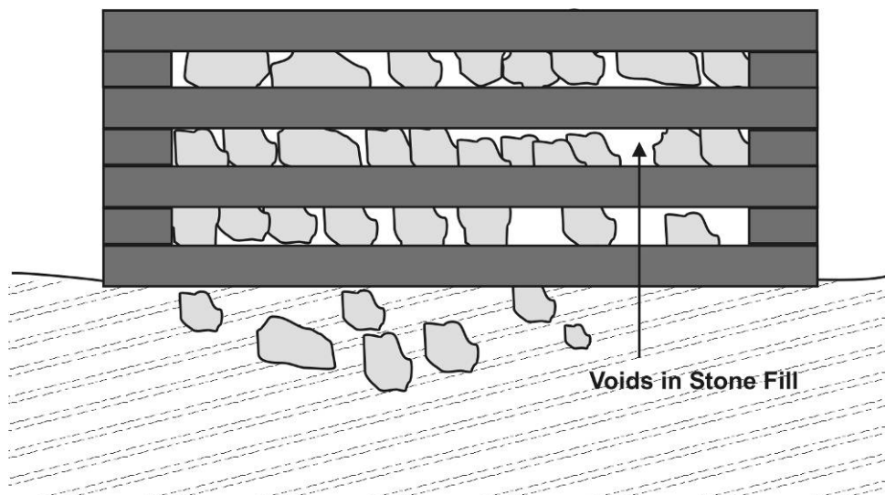
Figure 30. Loss of stone fill leaves gaps in the structure.
