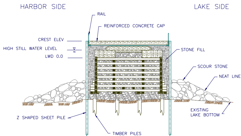
Figure 9c. Steel sheet pile encapsulation.
