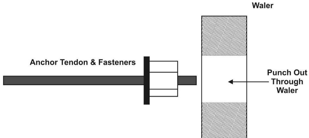
Figure 18. Connection lost between fastener and waler.
