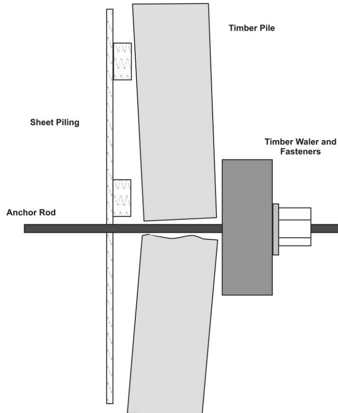
Figure 20. Fracture caused by external load.
