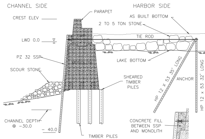
Figure 9d. Monolithic structure reinforced after failure.
