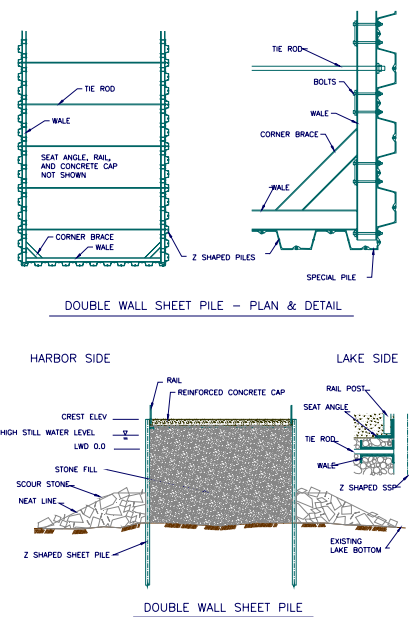
Figure 7b. Double wall sheet pile.
