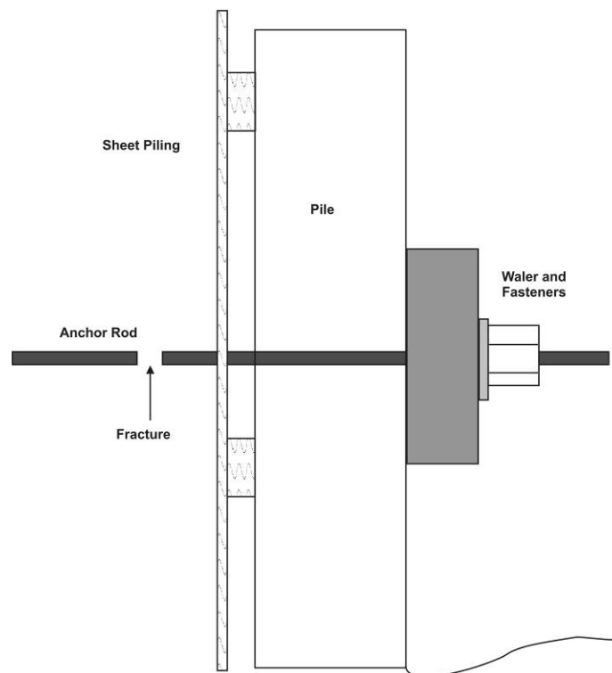
Figure 21. Fracture caused by remote external load.
