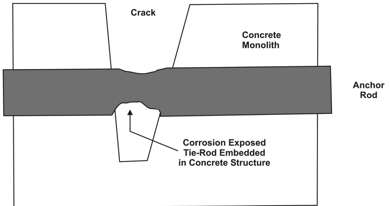
Figure 27. Deteriorated embedded tie-rod exposed by crack in concrete structure.
