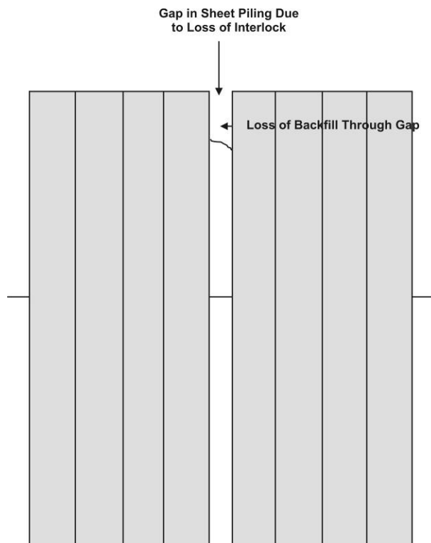
Figure 32. Gap in sheet piling causes loss of backfill.
