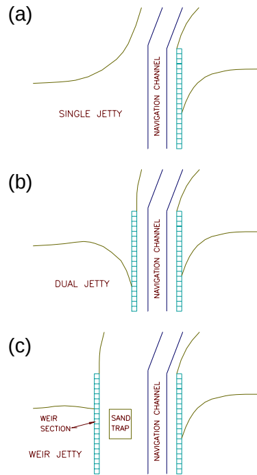
Figure 5. Jetty configurations.
