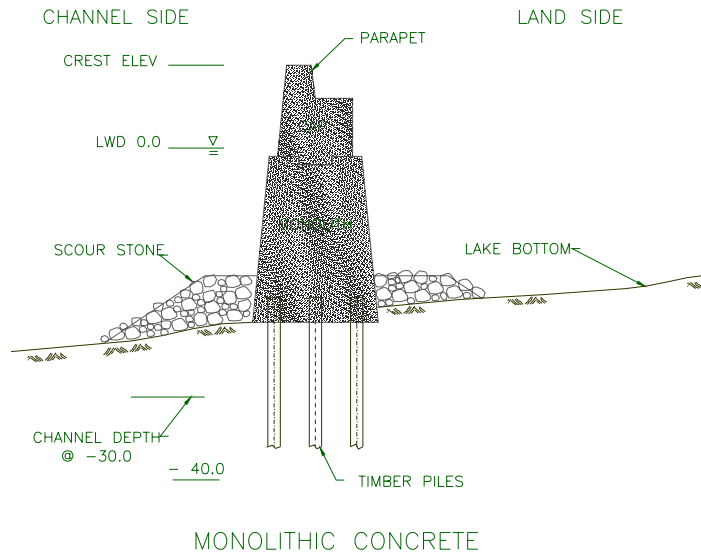
Figure 7g. Monolithic concrete.
