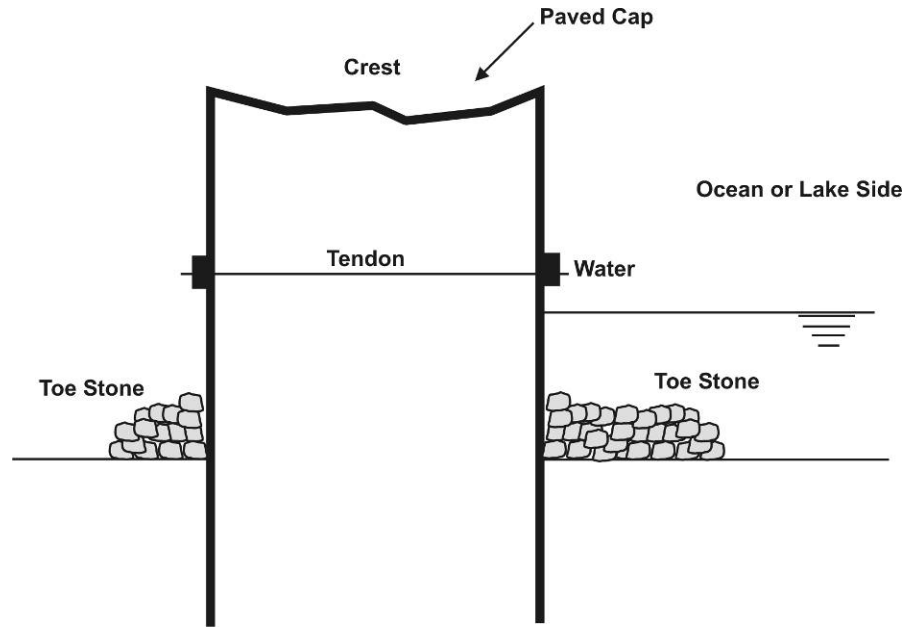
Figure 31. Loss of fill material leaves voids causing crest collapse.
