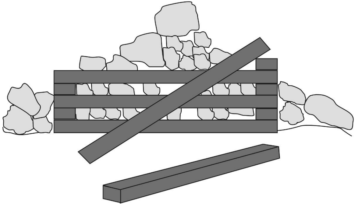
Figure 33. Retained stone fill can be lost if timber crib fails.
