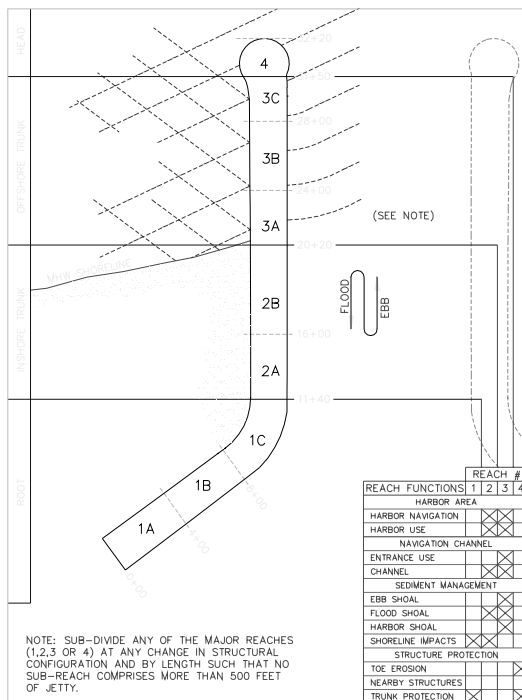
Figure 10. Typical reaches of a jetty.
