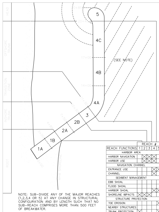
Figure 11. Typical reaches of a shore-connected breakwater.
