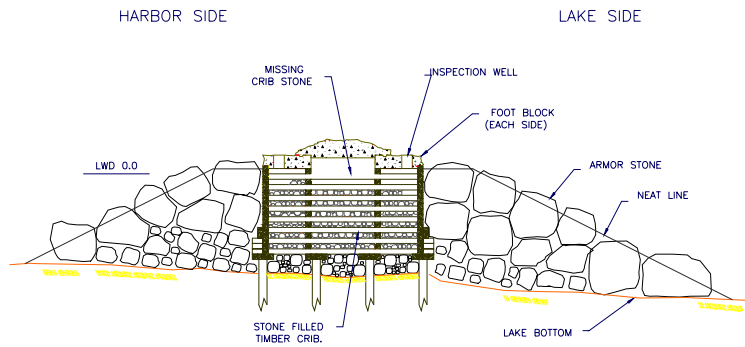
Figure 9b. Stone encapsulation.
