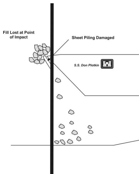
Figure 23. Impact damage.
