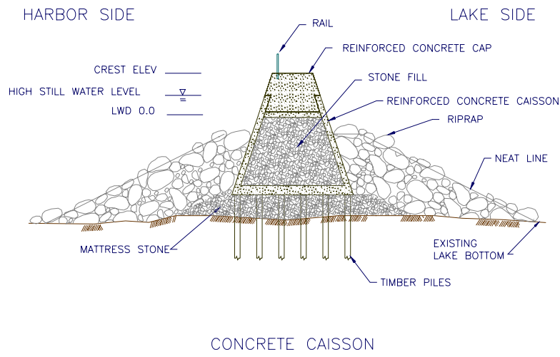
Figure 7f. Concrete caisson.
