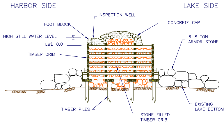
Figure 9a. Timber crib in need of repair.
