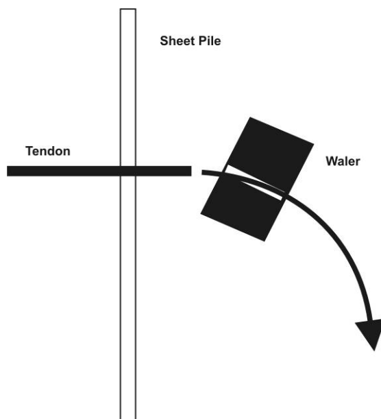
Figure 22. Waler lost from the structure.
