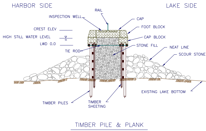
Figure 7e. Timber pile and plank.
