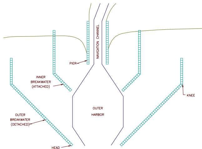
Figure 6. Breakwater configurations.
