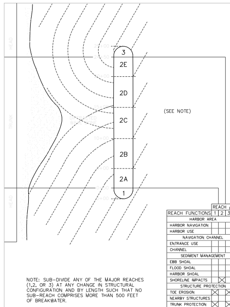
Figure 12. Typical reaches of a detached breakwater.
