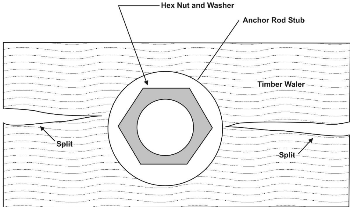
Figure 28. Longitudinal splitting of timber waler.
