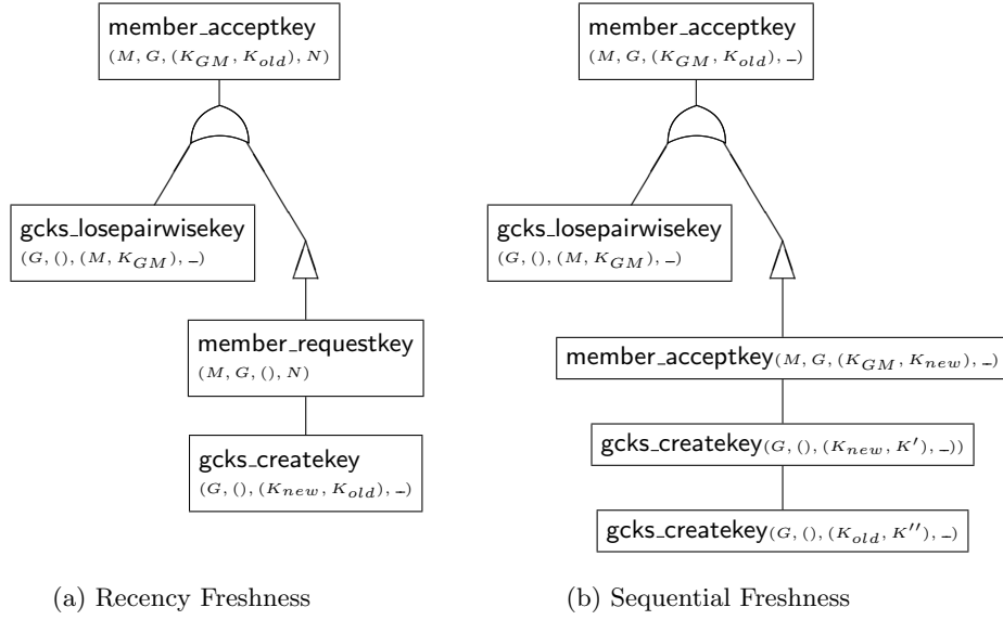
Fig. 2. Freshness Requirements for the GDOI Pull Protocol
