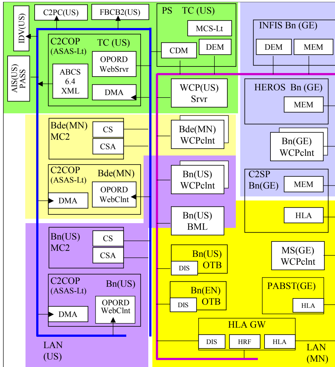
Figure 5. SINCEx1b Coalition Network Connectivity Architecture
