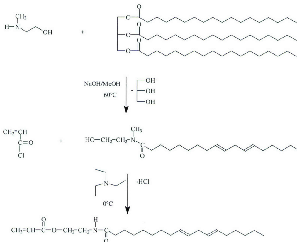
Figure 3. Linseed macromonomer synthesis.
