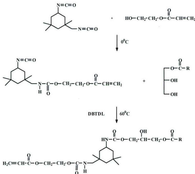
Figure 2. Linseed macromonomer synthesis.
