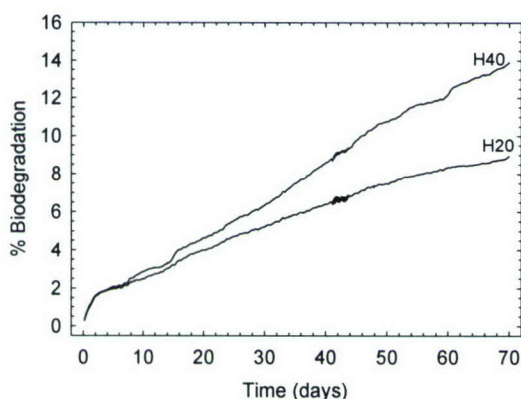
Fig 8. Biodegradation behavior of pure polyols.
