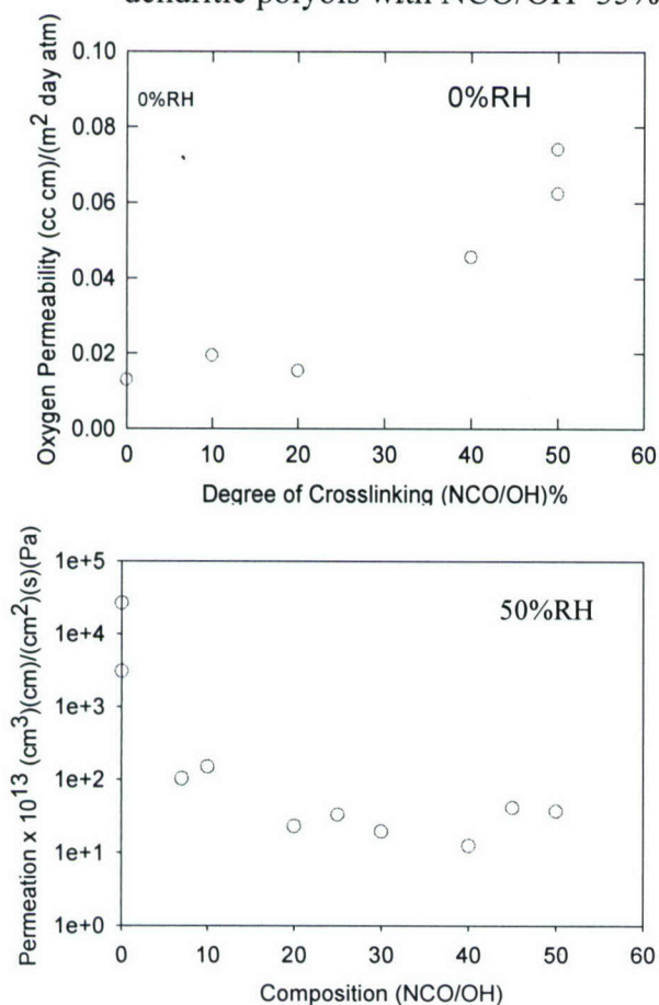
Fig11. Oxygen at 0%RH and water at 50%RH permeability of cross-linked Boltorn™ polyols
