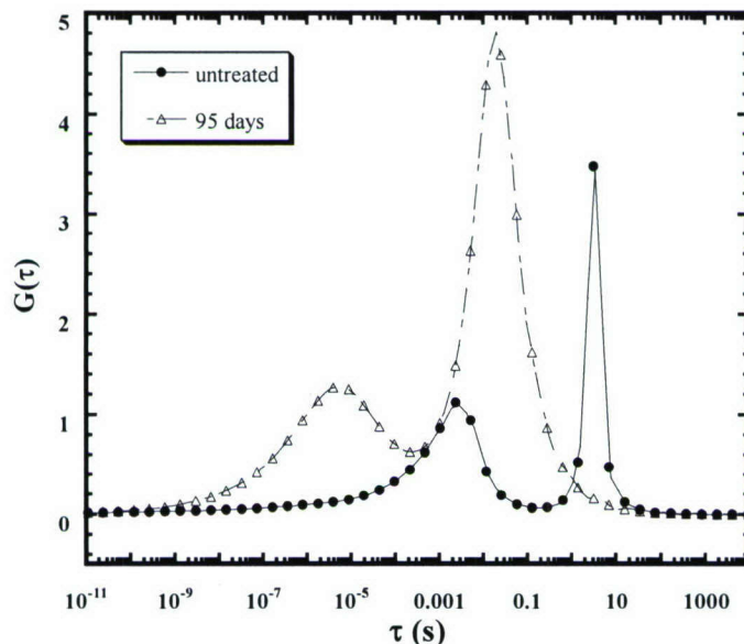
Figure 5. Distribution of dielectric relaxation times at 60° C for dry untreated and 95 d degraded samples.
