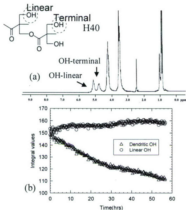
Fig4. (a) 1 H NMR of Boltorn™ in DMF at RT; (b) The kinetics of consumption of terminal and linear OH groups of H40 upon reaction with HDI at RT;
