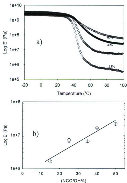
Fig6. (a) DMTA ( \text{Log } E' versus T ) curves for cross-linked systems characterized by different NCO/OH; (b) \text{Log } E' as a function of NCO/OH ratio;
