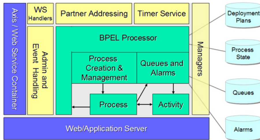
Figure 5: Engine Architecture
