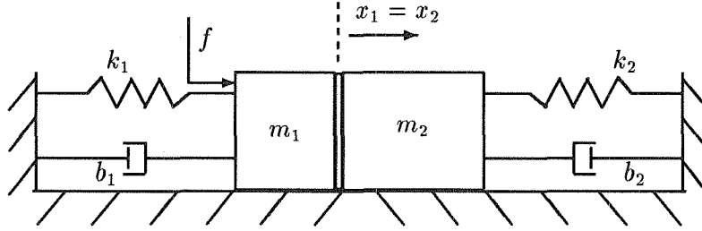
Figure 6: Interconnected system
