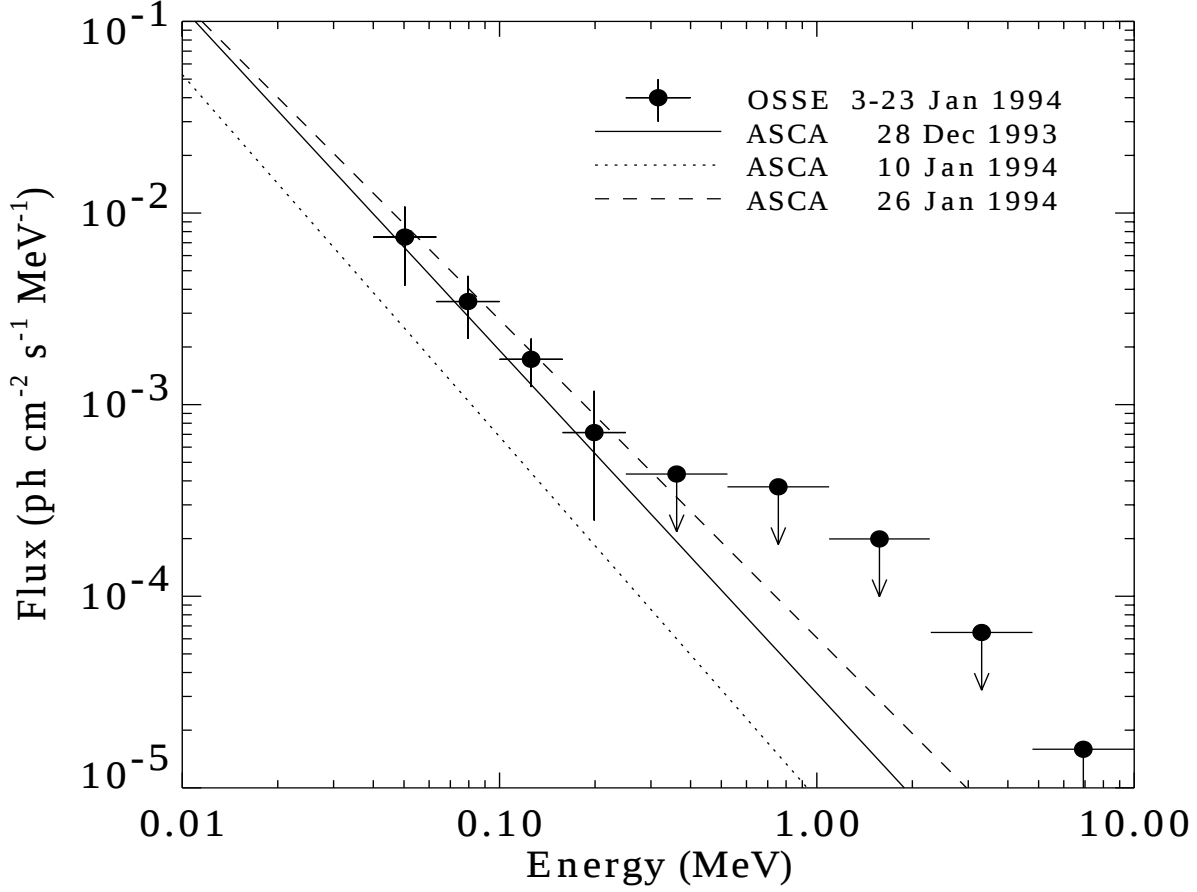
Fig. 1.— OSSE spectrum of emission from the region of PSR B1259-63. Schematic extrapolations to the power-law spectra of ASCA observations from 1993 December 28 (solid line), 1994 January 10 (dotted line), and 1994 January 26 (dashed line) are also shown. ASCA extrapolations obtained from the analysis of Kaspi et al. (1995).
