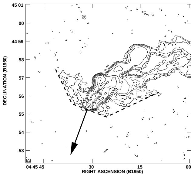
FIG. 2.—Closer look at the 90 cm map near the head of 3C 129, showing the Crosspiece feature extending to both sides. Contour levels are multiples of the 3\sigma noise in the map. The dashed line sketches the suggested location of the shock wave, which would have a Mach cone opening angle of \theta_{\text{Mach}} \approx 90^\circ . If this is correct, the arrow indicates the motion of 3C 129 within the plane of the sky. As argued in the text, the three-dimensional motion should not differ more than \sim 10^\circ from this. Note that the radio trails of 3C 129 are likely buoyant in the cluster ICM, so that their orientation need not be exactly parallel to the galaxy motion. This is supported by the strong bending of the large-scale morphology of the trails (Cowie & McKee 1975). Contour peak flux is 2.1954\text{E}-01 \text{ Jy beam}^{-1} , and contours are at 2.145\text{E}-03 times -2, -1, 1, 2, 4, 8, 16, 32 , and 64 .
