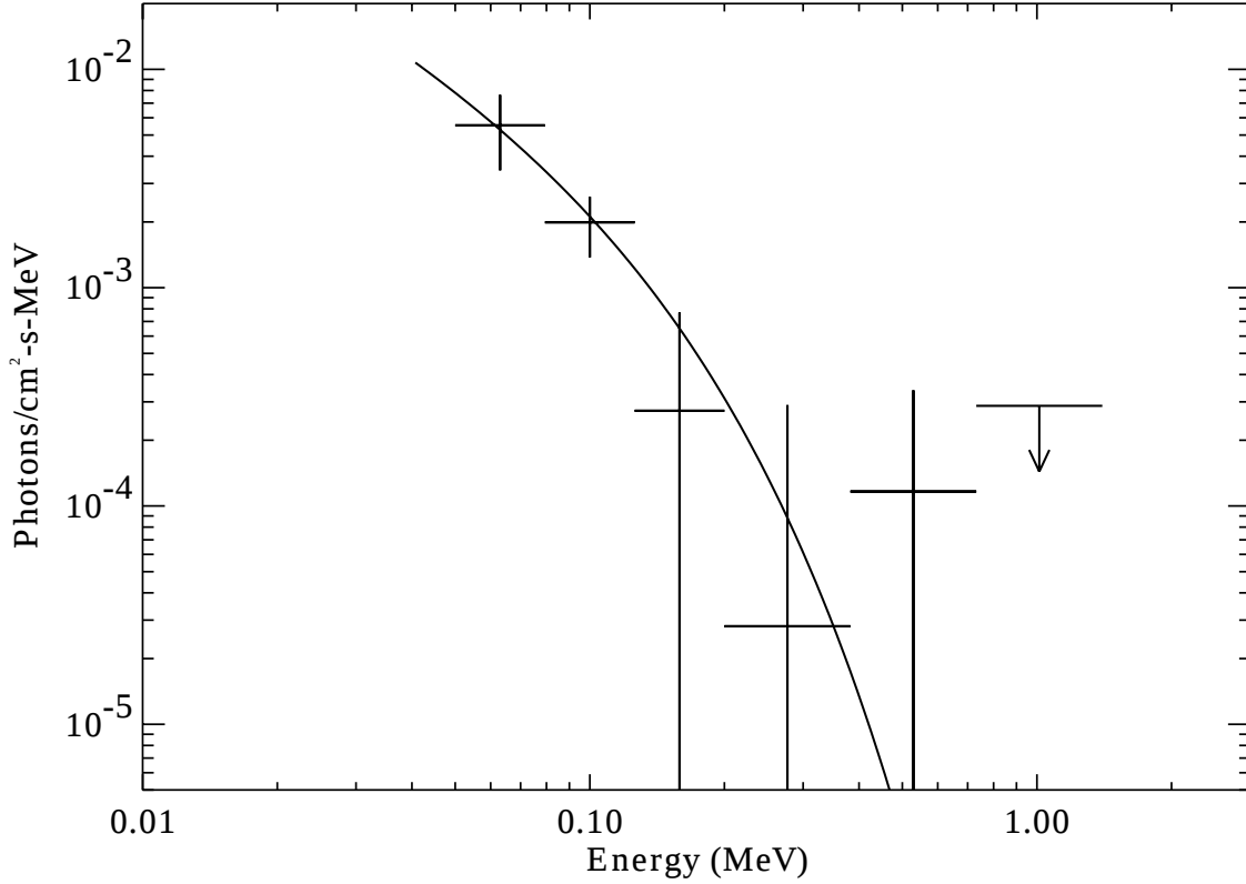
Fig. 1.— The SN 1993J photon spectrum observed by OSSE during the interval 9.9 to 15.4 days after the explosion (assumed 28.0 March). Error bars are 1\text{-}\sigma and the upper limit is the 2\text{-}\sigma limit. The solid line shows the best-fit thermal bremsstrahlung model used in the model-dependent deconvolution.
