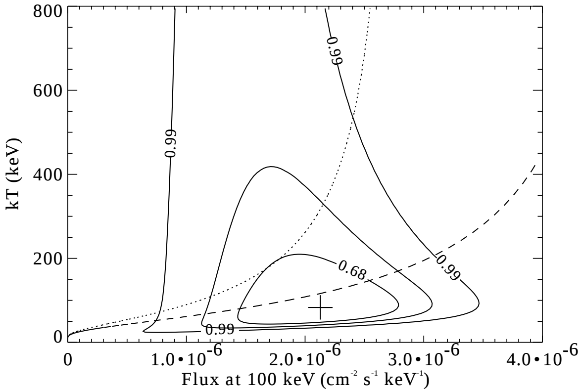
Fig. 2.— Confidence levels (68%, 90%, and 99%) for various values of the two parameters of the thermal bremsstrahlung model fit to the OSSE spectrum from the interval 9.9 to 15.4 days. The cross shows the position of the best fit. The temperature is well constrained on only the low side. The dashed line shows the combinations of parameter values that extrapolate to the absorption corrected total flux observed from 0.1–2.4 keV by ROSAT on day 12 (Zimmermann et al. 1994). Similarly, the dotted line shows parameter combinations that agree with the reported ASCA total flux (1–10 keV) on day 8 (Tanaka 1993).
