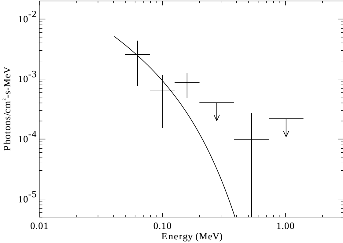
Fig. 3.— The SN 1993J photon spectrum observed by OSSE during the interval 23.7 to 37.0 days after the explosion (assumed 28.0 March). The solid line shows the best-fit thermal bremsstrahlung model.
