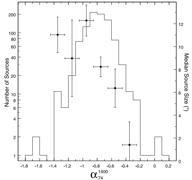
FIG. 9.—Spectral histogram along with median sources sizes as a function of spectral index. Source sizes are determined with the FIRST images, while spectral indices are determined using the 74 MHz integrated flux density and the NVSS flux densities. Not enough sources were detected with \alpha_{74}^{1400} < -1.45 or \alpha_{74}^{1400} > -0.25 for meaningful statistics in those regions.
