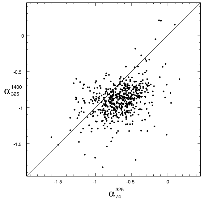
FIG. 8.—Radio color-color diagram of the 545 of 949 sources with both an NVSS and a WENSS counterpart. The diagonal line represents the location of sources for which \alpha_{74}^{325} = \alpha_{325}^{1400} . For most sources, the spectrum flattens considerably in the lower frequency interval.
