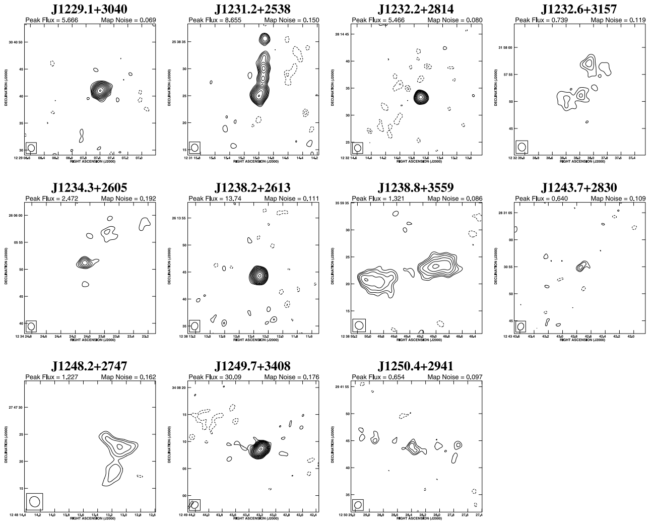
FIG. 11.—Images of the 11 detections from the 18 USS sources observed with the VLA A configuration at 1.4 GHz. The remaining seven are diffuse enough to be resolved out at this resolution of roughly 1''.4 .
