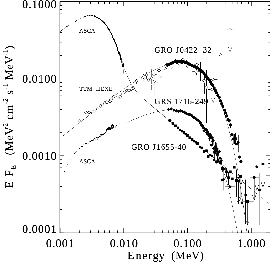
Fig. 3.— Luminosity per logarithmic energy interval for those transient BHCs with best-quality broadband spectral data. Contemporaneous TTM and HEXE data (open diamonds) and ASCA data (crosses) are shown for GRO J0422+32 and GRS 1716-249, respectively. Non-contemporaneous ASCA data are shown for GRO J1655-40 (crosses), scaled as indicated in the text.
