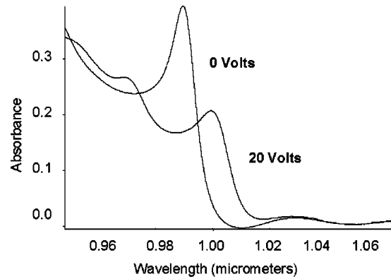
Fig. 2 Absorbance versus wavelength is shown for a 987-nm device. In its quiescent state, in this case, the MQW shutter blocks the transmission of incident light. When a moderate voltage is applied, the absorbance shifts and light is transmitted through to the retroreflector.
