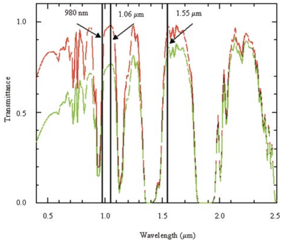
Fig. 7 Transmission curves are shown for a clear day (red) and for a misty day (green). These are two-way transmission data through the entire atmospheric channel and include losses from absorption and from Rayleigh and Mie scattering. It can be seen that at 1.06 and 1.55 \mu\text{m} , there is a transmission “window” for viable data links.
