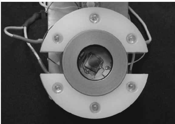
Fig. 10 The payload is shown. A modulating retroreflector mounted and ringed by standard LEDs. The LEDs were used for tracking and acquisition for first tests and are replaced with modulating retros in subsequent tests.
