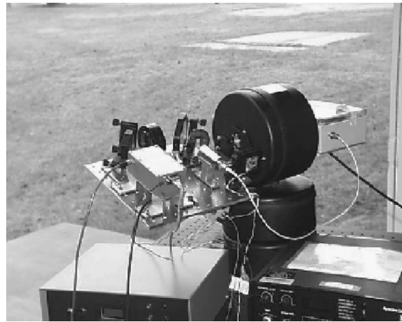
Fig. 11 The transmit/receive assembly used in the NRL MQW field tests is shown. The laser diode light is coupled into a fiber, which is connected to the lens system. The transmitted then retroreflected light is returned using a beamsplitter and the signal is captured by a standard avalanche photodiode.
