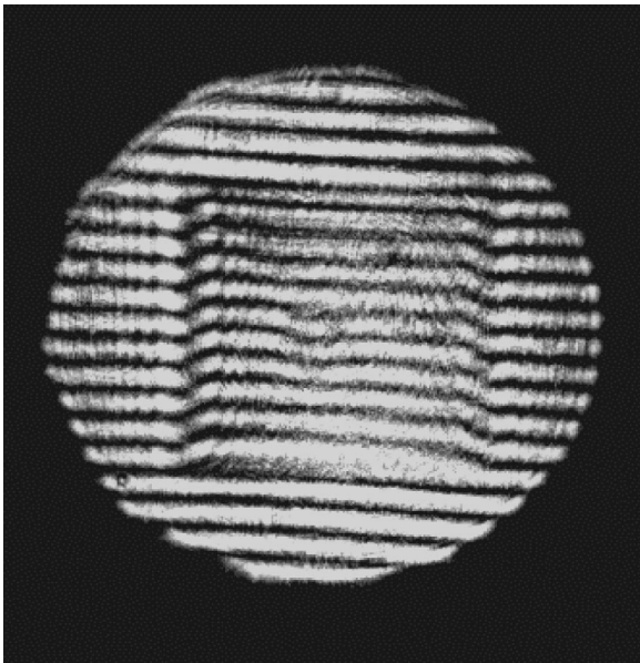
Fig. 5 An interferogram of an InGaAs transmissive MQW modulator is shown. The ripples around the square are edge effects around the sample. It can be seen that the surface is relatively good and should not deleteriously impact system performance.
