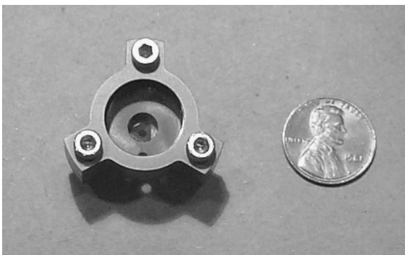
Fig. 13 The new mount for upcoming tests is shown. The unit that houses the retro, MQW shutter, cover plate, leads, and bolts is 10 g. The unit will be configured with several more into an array to increase the payload FOV and further relax onboard pointing and tracking requirements.
