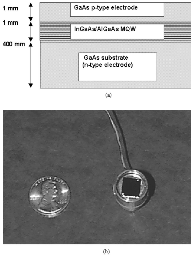
Fig. 3 Wide aperture MQW shutter: (a) schematic of a MQW modulator, with the GaAs material grown in alternating layers with active regions about 1\ \mu\text{m} thick; and (b) a fabricated 0.5-cm transmissive device. The NRL large aperture MQW devices operate between 850 nm and 1.06\ \mu\text{m} to date.
