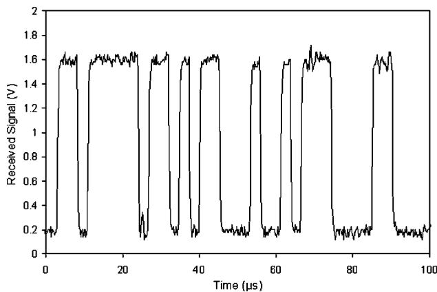
Fig. 12 A sample of the return from data captured in flight using the NRL MQW retroreflector is shown. As long as the link was maintained through accurate pointing and tracking, signal amplitudes were high enough to maintain a robust communications link.
