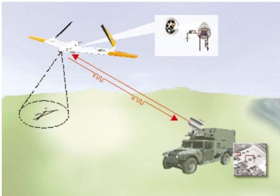
Fig. 8 The MQW modulating retroreflector incorporated into an airborne reconnaissance concept using a UAV is shown. When configured into an array, the MQW modulating retroreflector concept significantly reduces the parasitic payload requirements for the onboard communications system.
