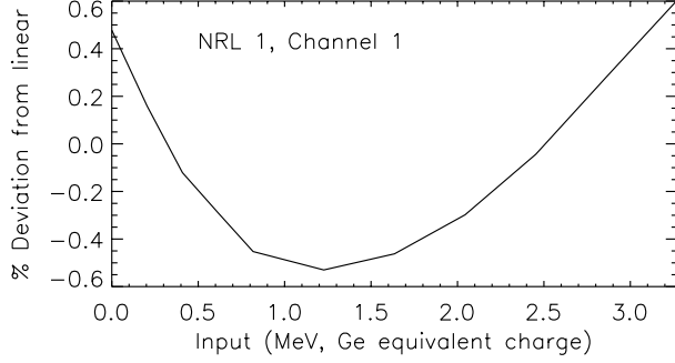
Figure 1: Integral linearity measurement of the CMOS preamplifier and shaping amplifier, NRL-1 . Plotted are the residuals from a best-fit linear model, relative to the full scale response at 3.3 MeV.
