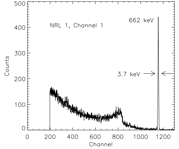
Figure 4: Energy spectrum using one strip from a germanium strip detector and channel 1 of NRL-1 . A uniform illumination of 662 keV gamma-rays was used. Detector and parasitic capacitance to ground in this system is 33 pF. The peak width is electronics dominated, and is consistent with the noise measurements presented in Figure 2.
