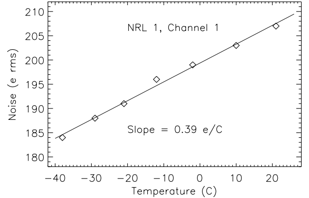
Figure 5: ENC measured for channel 1 of NRL-1 as a function of device temperature with a 1 pF capacitive load. Measurements were made with both increasing and decreasing temperature to ensure accuracy of the results. If the noise slope continues to 100 K, a potential improvement in energy resolution of 0.5 keV FWHM would be possible.
