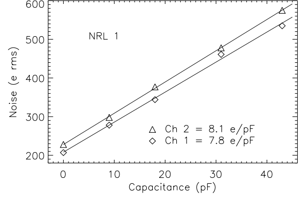
Figure 2: ENC vs. detector capacitance for NRL-1 . The front end p-channel MOSFET for channel 2 has twice the gate area as channel 1. The curves suggest that the smaller gate area provides slightly better performance.
