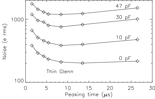
Figure 3: Noise vs. peaking time for the Thin Glenn preamplifier. The Thin Glenn is nearly identical to channel 1 of NRL-1 , except for a somewhat higher bandwidth. These measurements established the optimum peaking time used in the shaping amplifier stage of NRL-1 .
