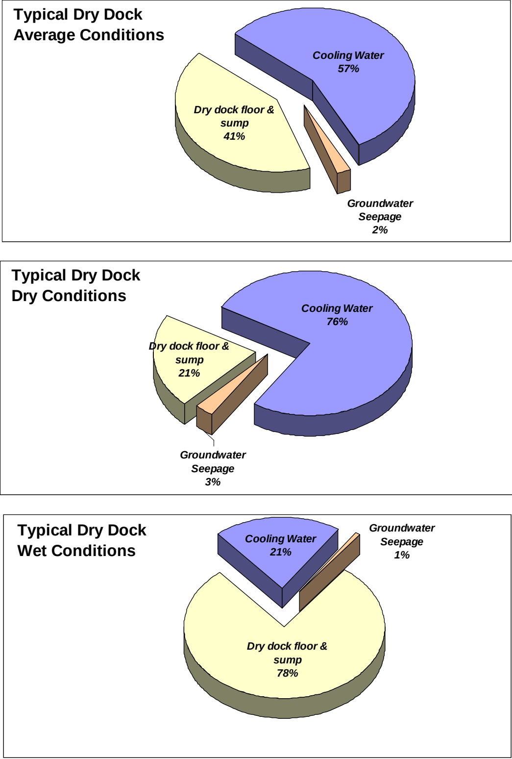
Figure 5. Mass balance calculations for typical dry dock conditions at PHNSY&IMF.
