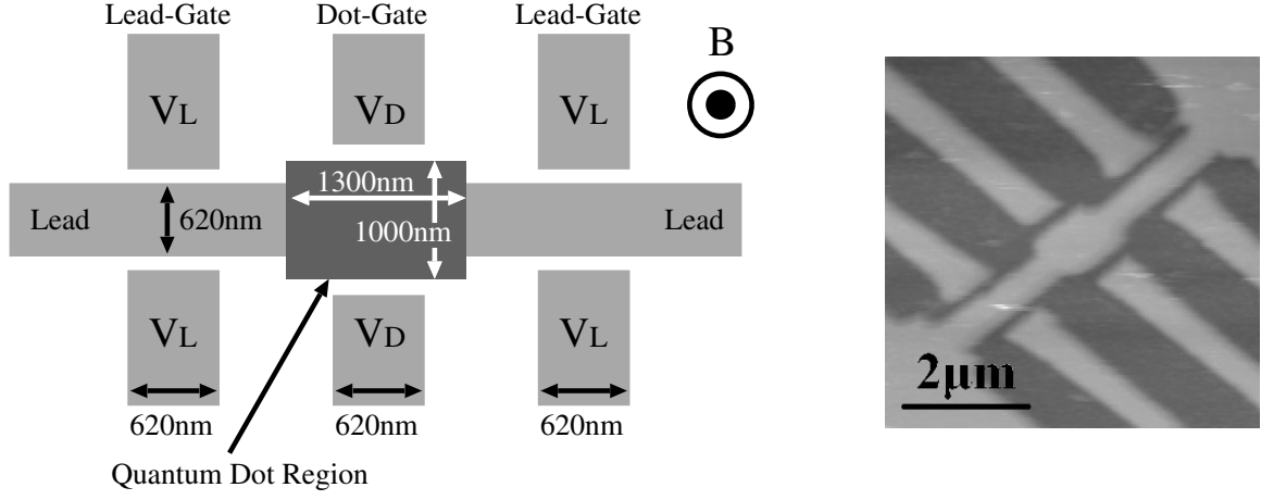
Figure 1. Schematic diagram of the side-gated quantum-dot structure (left) and AFM image of the sample (right).
