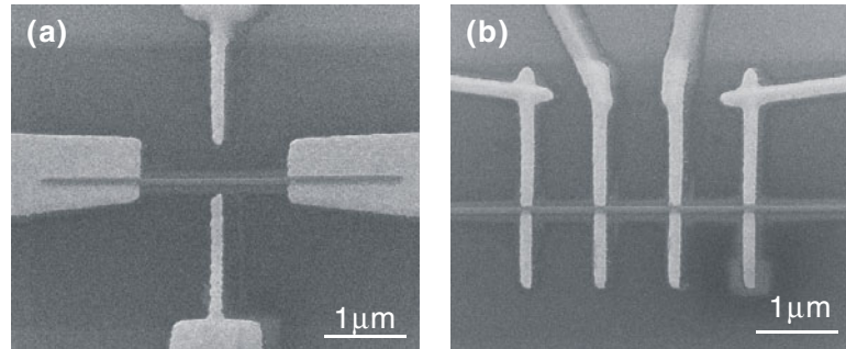
Fig. 1: SEM micrographs of typical specimens for (a) two-terminal configuration with gate electrodes and (b) four-terminal configuration. The bright regions are the Au/Ti electrodes on the SiO 2 /Si surface. The horizontal thin lines in the middle are the FIB-deposited Pt wire.
