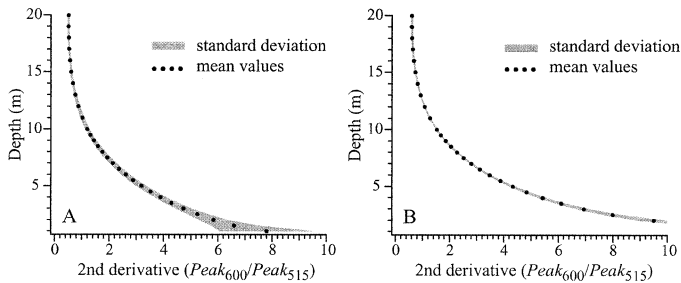
Fig. 8. Mean of second derivative peak ratio (Peak 600 /Peak 515 ) versus depth for spectral library. (A) Sediment and seagrass. (B) Pavement/reef.
