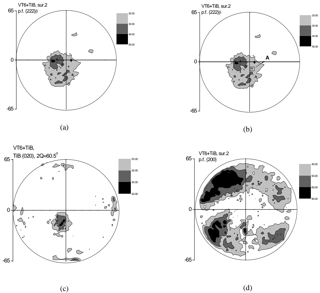
Fig.1. (a, b) Central part of \{222\}\beta pole figures taken from two neighboring locations on the plane orthogonal to ingot axis; \{222\} orientations are slightly inclined to the ingot axis. (c, d) – Central part of \{020\} TiB and \{200\}\beta pole figures respectively taken from the location (b) in Fig.b; there are no (200) orientation in the center, while distribution of \{020\} TiB is similar to that of \{222\}\beta .
