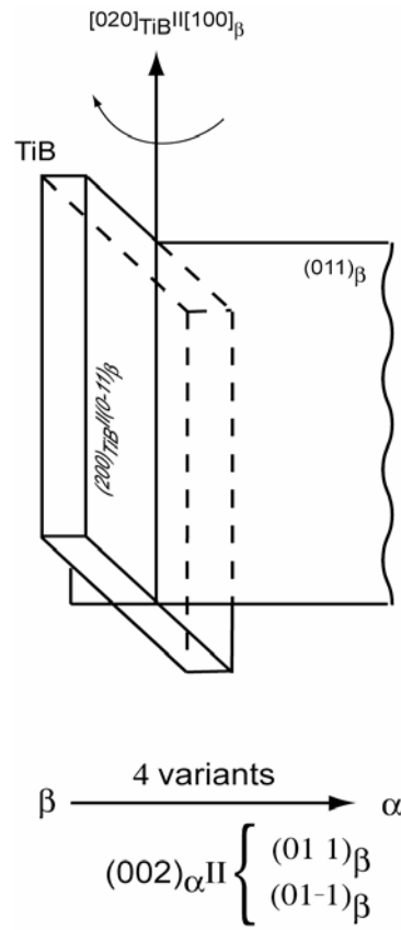
Fig. 8 Crystallography of eutectic couple TiB – beta Ti.
