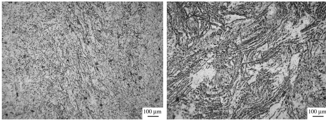
Fig. 10. Typical microstructures of forged slab: (a) - structure resulted from regular eutectic grains; (b) – structure resulted from degenerated zones. LM.
