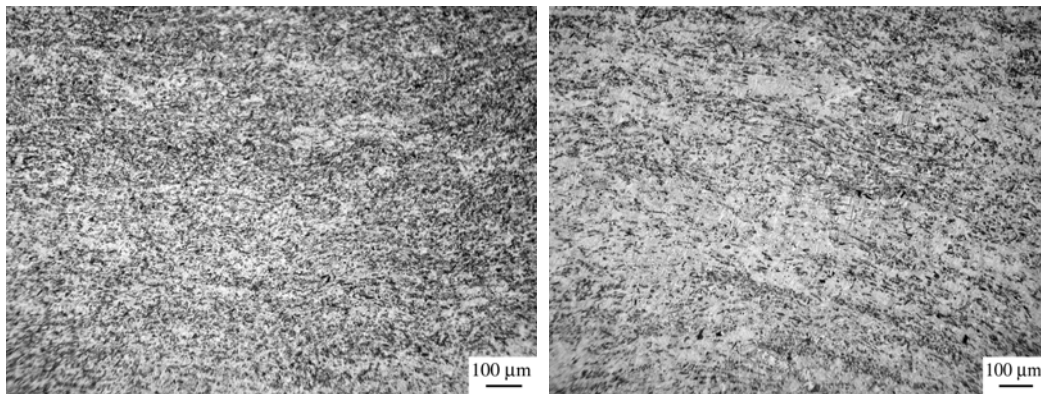
Fig. 10. Typical microstructures of forged slab: (a) - structure resulted from regular eutectic grains; (b) – structure resulted from degenerated zones. LM.
