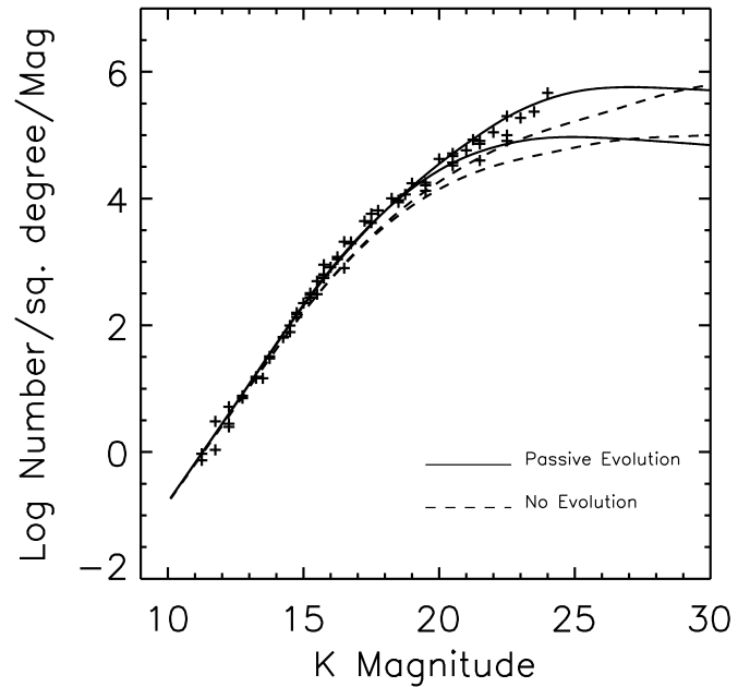
FIG. 3.— K -band number counts (Djorgovski et al. 1995; Gardner, Cowie, & Wainscoat 1993; Gardner et al. 1996; Glazebrook et al. 1994; Huang et al. 1997; Mobasher, Ellis, & Sharples 1986; Moustakas et al. 1997; McLeod et al. 1995; Metcalfe et al. 1996) together with models of the luminosity function modeled using the formalism of Gardner (1998), which has been used to extrapolate the number counts into the NGST domain. The solid lines include the effects of passive evolution, while the dashed lines include only K -corrections. The upper line in each case is for q_0 = 0.1 , and the lower lines are for q_0 = 0.5 . Current number counts imply at least 3500 objects per 3'3 NGST field, while the extrapolations shown here suggest as many as 11,000 to K = 29.5 .
