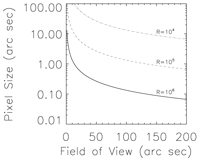
FIG. 4.—Pixel size as a function of the field of view required to spatially fully sample fringes at the edge of the FPA and hence maintain modulation efficiency. Curves are plotted for resolutions R = k/\delta k = 10^4 , 10^5 , and 10^6 assuming an 8 m diameter primary aperture and a beam splitter of diameter 10 cm.
