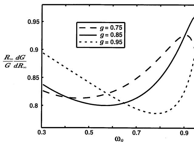
Fig. 11. Normalized sensitivity coefficient of G with respect to R_\infty for g of \beta_{HG} .
